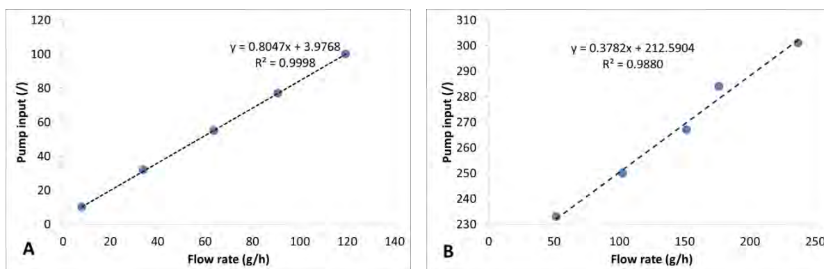
Figure 2-16. Calibration curves for enzyme (A) and substrate (B) pumps established on Ctec2 , dillution 10x and sugarcane bagasse.
