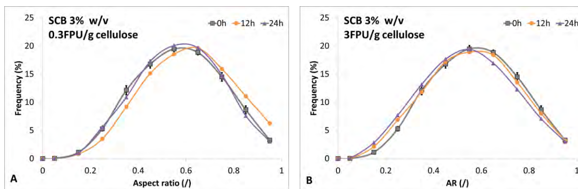
Figure 3-45. Number distribution of aspect ratio (AR) during enzymatic hydrolysis of SCB 3 %w/v with Ctec2 at E/S equal to 0.3 (A) and 3 (B) FPU/g cellulose.
