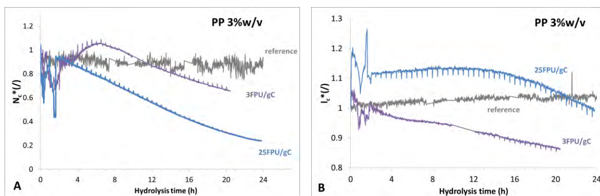
Figure 3-39. Evolution in N_c^* (A) and l_c^* (B) during enzymatic hydrolysis of PP 3 %w/v using Ctec2.
