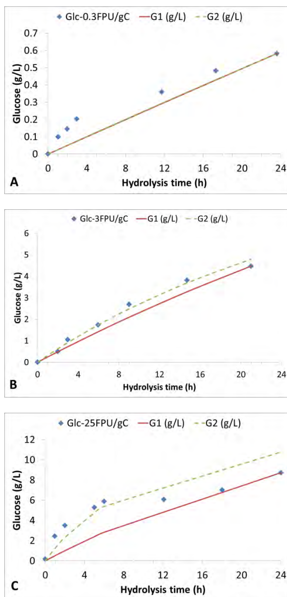
Figure 3-13. Predicted versus experimental values of glucose concentration released during the enzymatic hydrolysis of FP at 0.3 (A), 3 (B), 25 (C) FPU/g cellulose and 1.5 %w/v solid loading. G1: first order model, G2: second order model.
