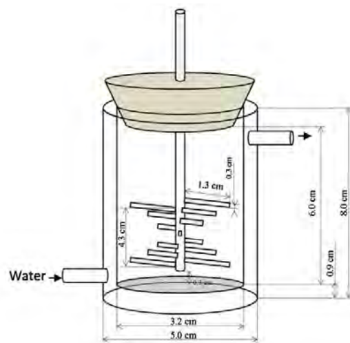
Figure 1-15. Peg-mixer bioreactor (Caspeta, Caro-Bermudez et al. 2014)
