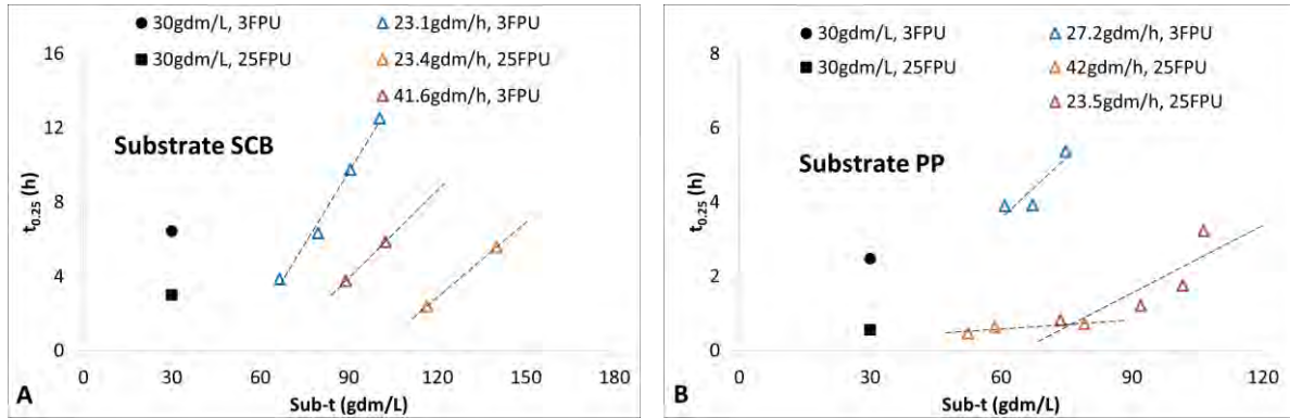
Figure 3-63. Time for 75 % viscosity reduction as a function of initial substrate concentration for batch and fed-batch hydrolysis with SCB (A) and PP (B).
