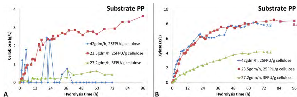
Figure 3-53. Cellobiose (A) and xylose (B) concentrations as a function of time and different feeding rates and E/S ratios with PP.
