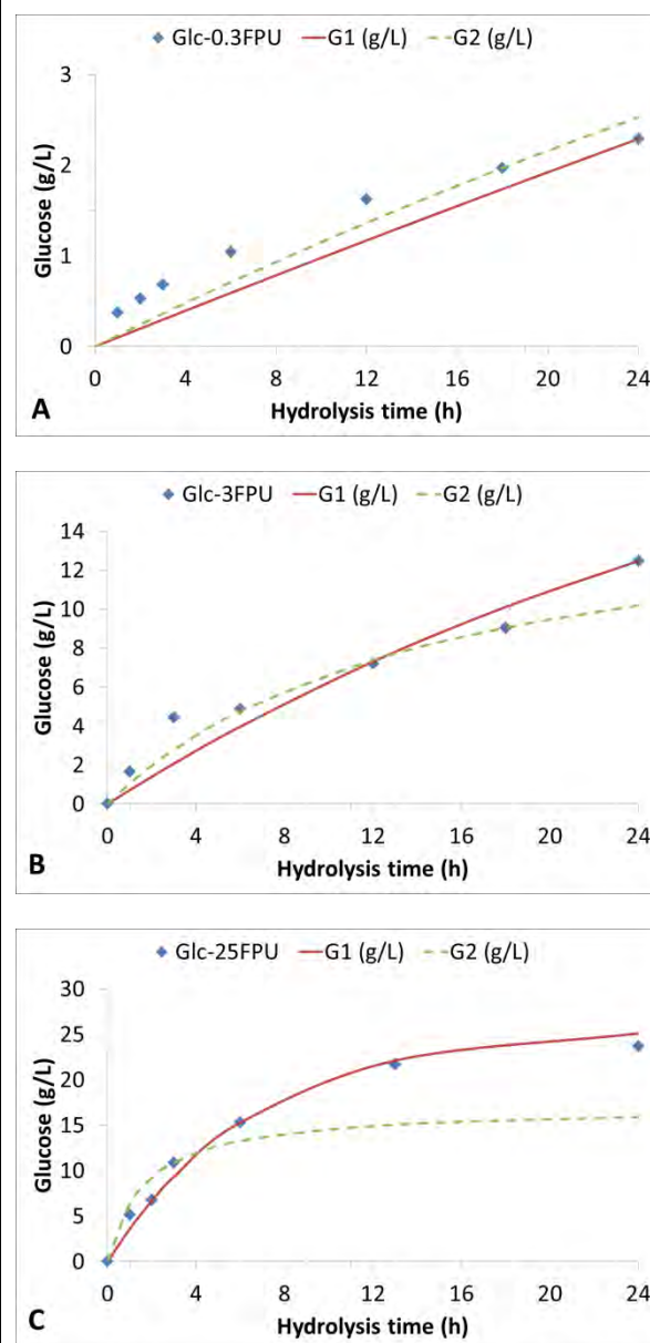
Figure 3-14. Predicted versus experimental values of glucose concentration released during the enzymatic hydrolysis of PP at 0.3 (A), 3 (B) and 25 (C) FPU/g cellulose and 1.5 %w/v solid loading. G1: first order model, G2: second order model.
