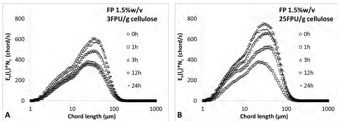
Figure 3-40. Evolution of number weighted chord count distribution (FP suspension, 1.5 %w/v) during hydrolysis with Ctec2 at E/S equal to 3 (A) and 25 (B) FPU/g cellulose
