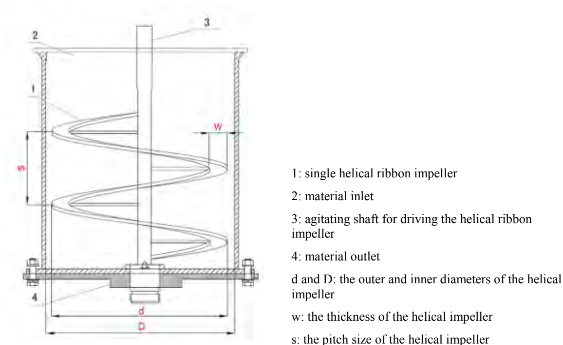
Figure 1-17. Schematic diagram of the mock-up reactors from Zhang, Zhang et al. (2014)
