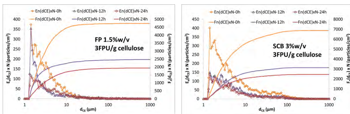
Figure 3-46. Change in E_n(d_{CE}) \times N for FP suspension during enzymatic hydrolysis using Ctec2 at 3 FPU/g cellulose (dilution rate 1/10).
