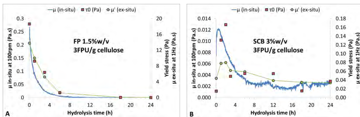
Figure 3-21. Correlation between ex-situ rheometry and in-situ viscometry for FP and SCB at 3 FPU/g cellulose.
