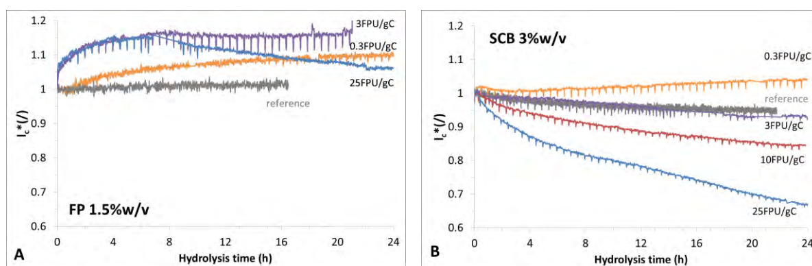
Figure 3-38. Evolution in l_c^* during enzymatic hydrolysis of FP 1.5 %w/v (A) and SCB 3 %w/v (B) for enzyme/substrate loading ranging from 0.3 to 25 FPU/g cellulose.
