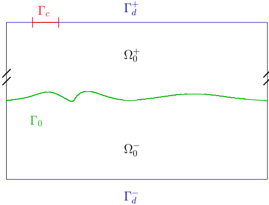
Figure 3.1: Initial configuration in dimension d = 2 with \Gamma_c \subset \subset \Gamma_d^+ .
