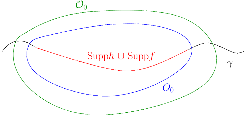
Figure 2.2: Construction of the cut-off \eta .
