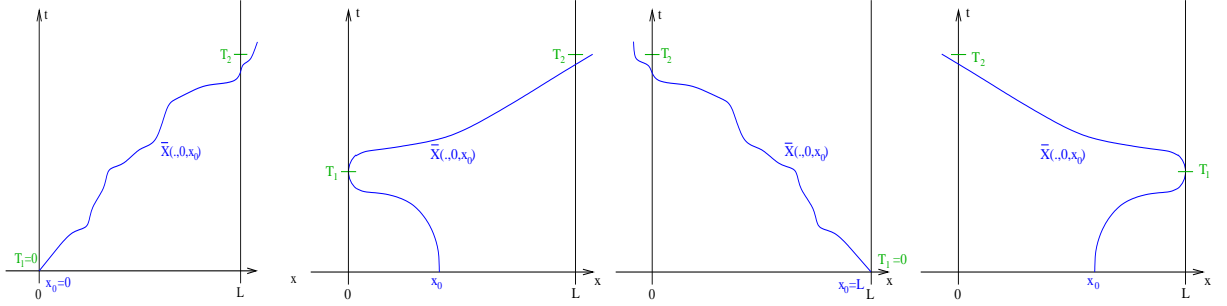
Figure 1.1: Some possible trajectories t \mapsto \bar{X}(\cdot, 0, x_0) .
