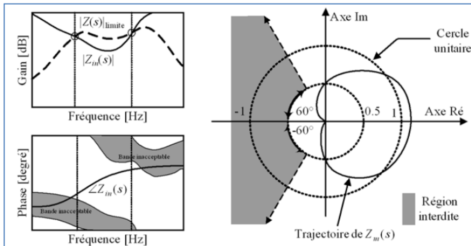
Figure 1-33 Bande inacceptable [66]
