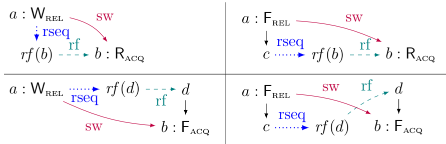
Figure 2.13: Illustration of the “synchronizes-with” definition: the four cases inducing an \text{sw} edge.
