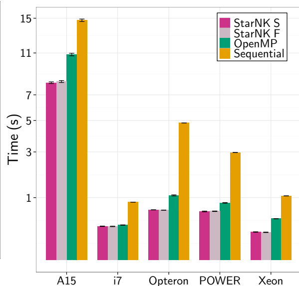
Figure 6.11: LDPC
