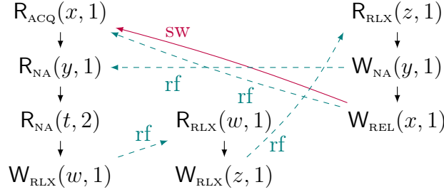
Figure 3.3: Execution generating new behaviour if the expression evaluation order is linearised.
