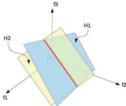
Figure 3.10: Hyperplanes in a three-dimensional image space for two measurements which corresponding lines in the projection matrix are equations of planes of \mathbb{R}^3 . the red segment belongs to the line of solutions. Therefore if only H1 and H2 are available to estimate the solution in the form of a point, the problem is ill-posed since no unique solution can be found.
