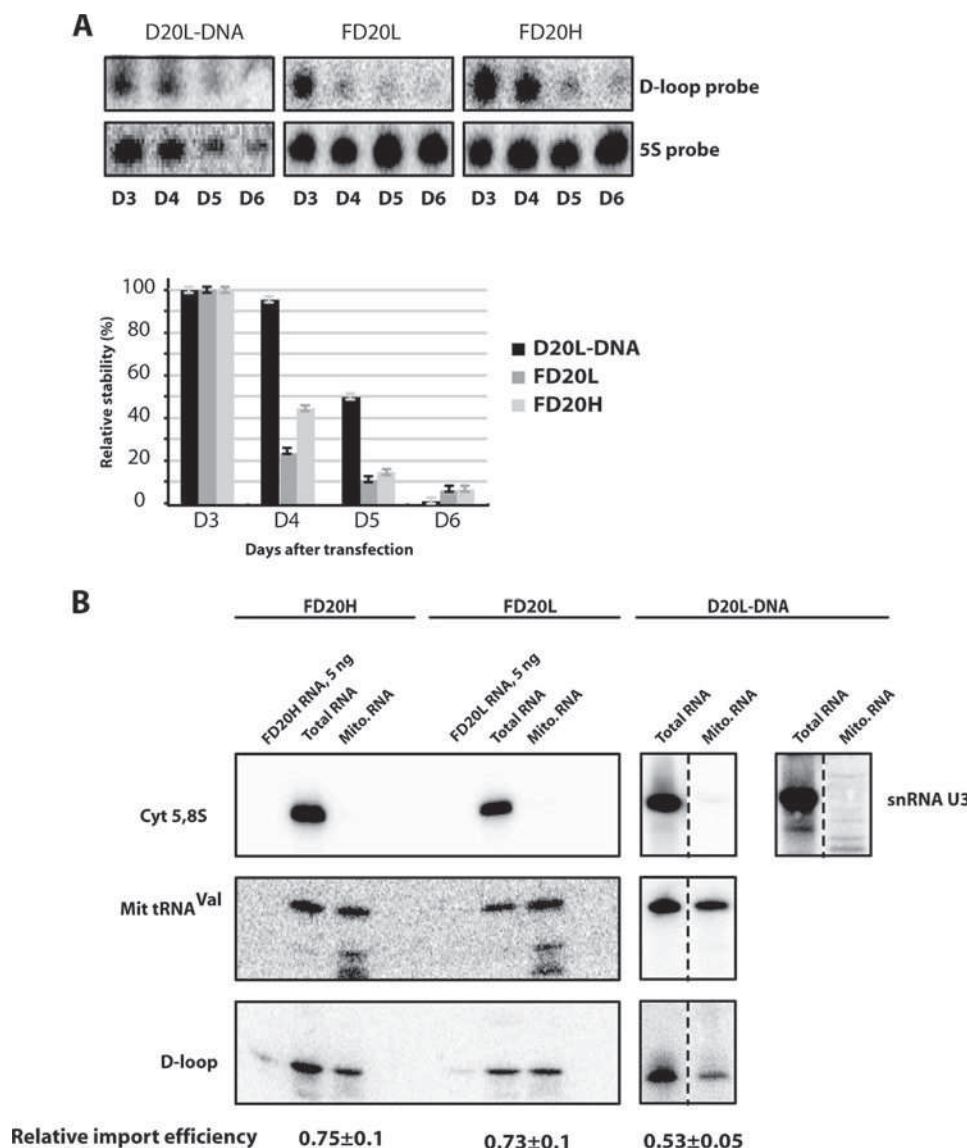
FIGURE 4. Anti-replicative RNA stability and mitochondrial import in transiently transfected cybrid cells. A , an example of Northern hybridization of total RNA isolated in 3–6 days after cell transfection (as indicated below) with various recombinant molecules (indicated above the panels). Probes used for hybridization: D-loop, specific for all recombinant molecules used for transfection; 5S, against 5 S rRNA to quantify the level of recombinant RNA in the cells. Time dependence of RNA decay is shown below (means \pm S.D. calculated from at least four independent experiments). B , mitochondrial import of recombinant molecules in transiently transfected cybrid cells. Northern hybridizations of RNA extracted from cells (Total RNA) or purified mitoplasts (Mito RNA) 48 h after transfection. Above, RNAs used for transfection are indicated. On the left, hybridization probes: D-loop, specific for recombinant molecules used for the transfection; Cyt 5.8S, against 5.8 S rRNA to check the absence of cytosolic RNA in mitochondrial samples; snRNA U3, demonstrating that the mitoplast fraction was not contaminated by the small nuclear RNAs; Mit tRNA Val , to normalize the level of recombinant RNA to amount of loaded material. Import efficiency was estimated as a ratio of mitochondrial to total signal for the D-loop probe after normalization of the both signals to those for mitochondrial tRNA Val probe.
