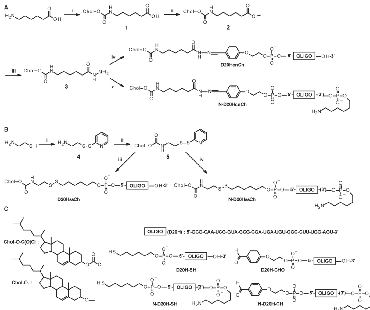
Figure 1. Synthesis of oligoribonucleotides conjugated with cholesterol through cleavable covalent hydrazone ( A ) and disulfide ( B ) bonds. Reagents: A , i) (\text{CH}_3)_3\text{SiCl} , Py, 4^\circ\text{C} ; \text{CholOC}(\text{O})\text{Cl} , Py, r.t.; \text{H}_3\text{O}^+ ; ii) \text{PCl}_3 , \text{CH}_2\text{Cl}_2 , argon, 50^\circ\text{C} ; \text{MeOH}_{\text{abs}} , r.t.; iii) \text{NH}_2\text{NH}_2 \cdot \text{H}_2\text{O} , \text{MeOH} , r.t.; iv) D20H-CHO, 0.1M NaOAc, pH 5.0/dioxane, r.t.; v) N-D20H-CHO, 0.1M NaOAc, pH 5.0/dioxane, r.t.; B , i) (\text{PyS})_2 , \text{MeOH}/\text{AcOH} , r.t.; ii) \text{CholOC}(\text{O})\text{Cl} , \text{CH}_2\text{Cl}_2/\text{dioxane}/\text{Et}_3\text{N} , argon, r.t.; iii) D20H-SH, dioxane, r.t.; iv) N-D20H-SH, dioxane, r.t. C . Structure of compounds used for the synthesis.
