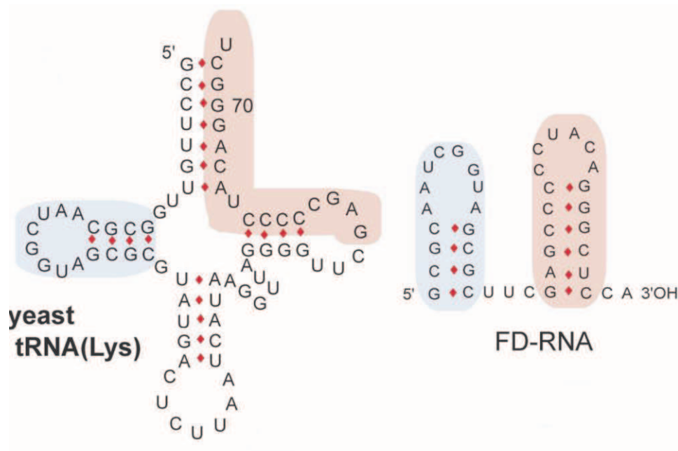
Figure 14. The structures of yeast tRNA Lys and short synthetic FD-RNA obtained by fusing both determinants of import: D-arm and F-hairpin (Comte et al., 2013).
