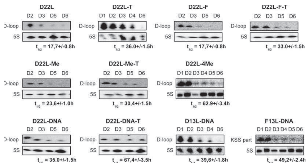
Fig. 2. Stability of synthetic oligonucleotides in transiently transfected cybrid cells. Northern hybridization of total RNA isolated in 2–6 days after cell transfection (“D2-6”, as indicated above the lanes) with various SO-specific 32 P-labelled probes (the SO is indicated above each panel, the probe – at the left). Probes used for hybridization: D-loop or KSS-part, specific for SO used for transfection; 5S, against 5S rRNA to quantify the level of SO in the cells. Below each panel, a half-life time for corresponding SO is indicated; \pm SD was calculated from n = 3 independent experiments.
