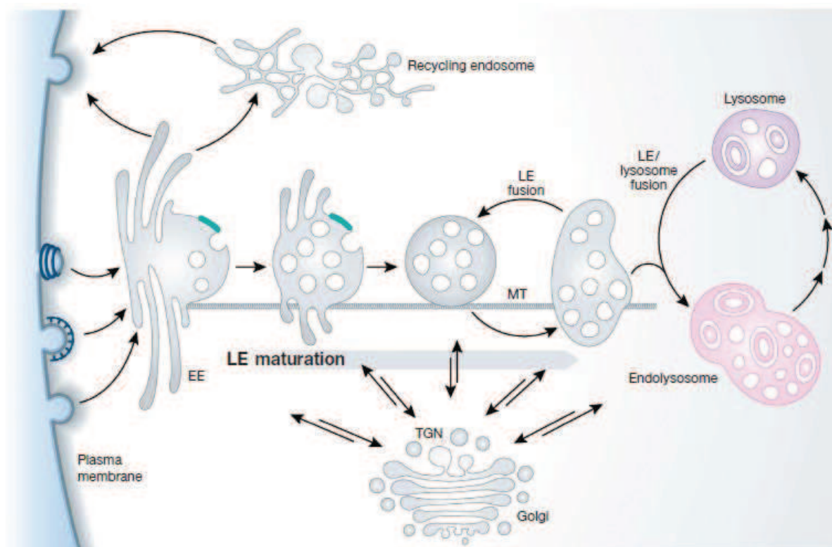
Figure 1. The endosome/lysosome system. Primary endocytic vesicles deliver their cargo to early endosomes (EEs) in the peripheral cytoplasm. During endosomal processing EEs move to the perinuclear space with the help of microtubules (MT) and mature into late endosomes (LEs). Processing of LEs results in the increased size due to fusing and concentration of lysosomal hydrolases derived from the trans-Golgi network (TGN). Moreover, the LE pH drops from 6.8 to 4.9 during the maturation process. Finally, LEs fuse with a lysosome and form the endolysosome, in which active degradation takes place (Huotari and Helenius, 2011).
