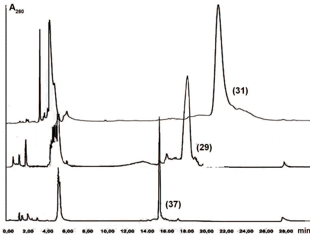
Figure S1. RP-HPLC of crude reaction mixtures of Ch0-ON1 ( 29 ), Ch6-ON1 ( 31 ) and OI-ON1 ( 37 ) performed using Alliance Waters chromatographic system with a XBridge C18 column (2.5 \mu m, 4.6 x50 mm) at 50°C. Flow rate 1 ml/min; buffer A, 0.05 M NaClO 4 ; buffer B, 0.05 NaClO 4 /90% CH 3 CN).
