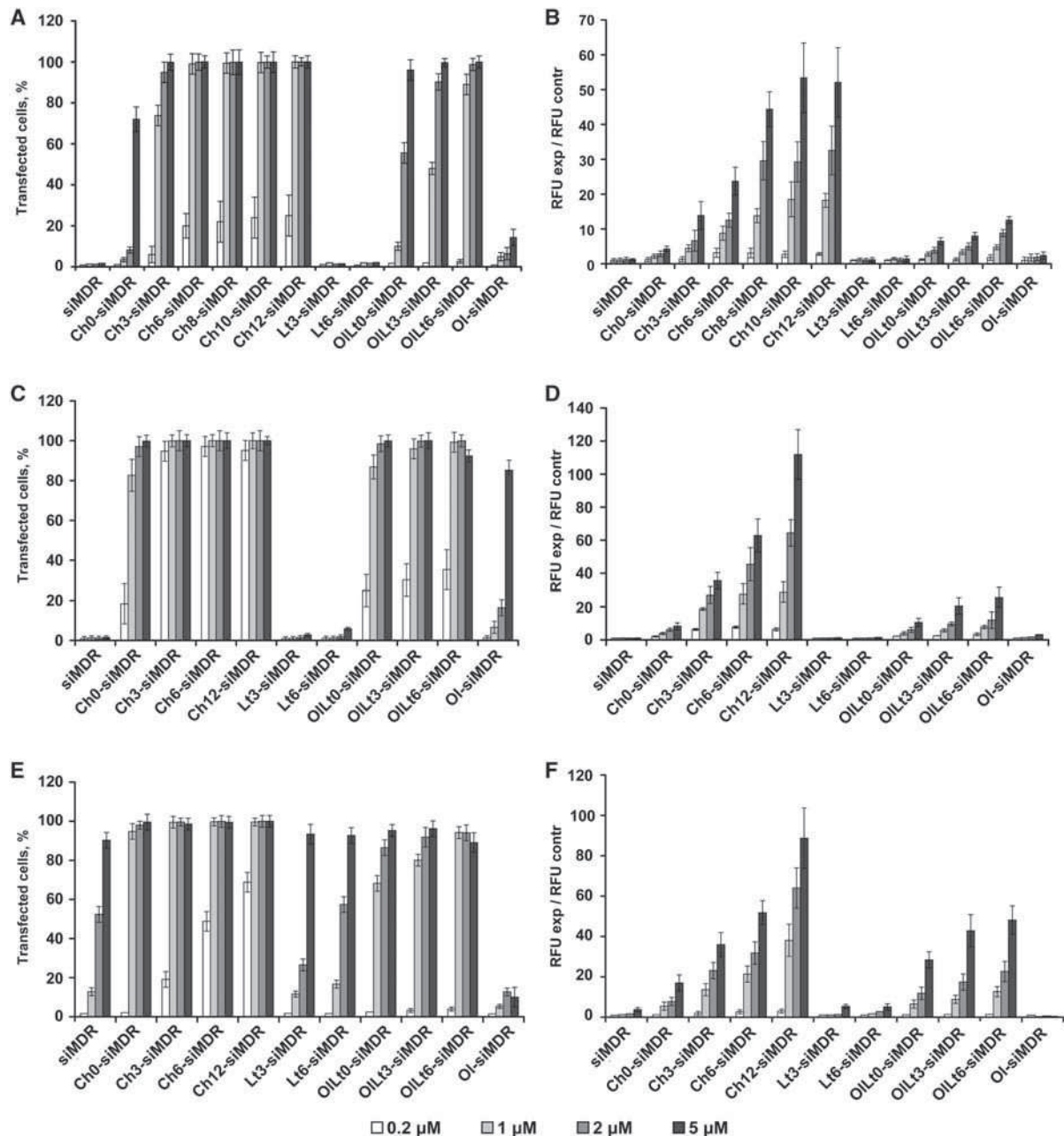
Figure 2. Cellular accumulation of FITC-labeled lipophilic siRNAs. The percentage of FITC-positive cells in the population (%) (A, C and E) and the normalized mean value of the cell fluorescence (RFU exp/RFU contr) (B, D and F) after incubation of KB-8-5 (A and B), HepG2 (C and D) and HEK293 (E and F) cells in the presence of corresponding siRNAs are shown. Data were obtained via flow cytometry. Fifteen thousand events were counted in each sample. Mean values ( \pm SD) from three independent experiments are presented.
