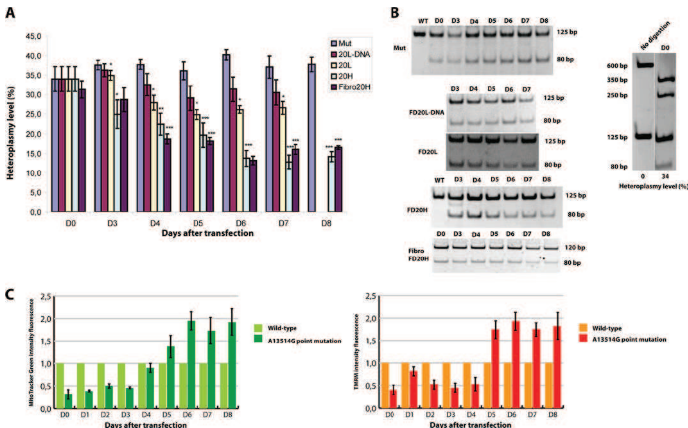
FIGURE 5. The effect of recombinant RNA on heteroplasmy level in transfected cybrid cells. A, time dependence of A13514G mutation heteroplasmy level (axis Y) followed during 7–8 days. D0–D8, days after transfection of cells with different recombinant molecules. Mut, mock-transfected cybrid A13514G cells; WT, mock-transfected 143B cells; FD20L, FD20H, or FD20L-DNA, cybrid cells transfected with corresponding recombinant molecule; Fibro 20H, primary fibroblasts transfected with FD20H RNA. Data are expressed as mean \pm S.D. for 3–5 independent experiments. Shown is an unpaired t test between values for mutant and transfected cells; *, p < 0.02 ; **, p < 0.003 ; ***, p < 0.0009 . B, an example of restriction fragment length polymorphism (RFLP) analysis for DNA samples isolated in 3–8 days (as indicated above) after cybrid cell transfection with recombinant molecules indicated at the left. Digestion control was performed for each reaction, as shown at the right panel. For this, 600-bp PCR fragment of mtDNA was cleaved by HaeIII to 350- and 250-bp fragments in the same tube as 125-bp PCR fragment spanning A13514G mutation site. The A13514G mutation creates a HaeIII-specific cleavage site, giving the fragment of 80 bp. Fragment size is indicated for each panel. C, evaluation of total and energized mitochondria content in 143B (wild type) and cybrid cells (A13514G) transfected with RNA FD20H during 8 days after cell transfection. MitoTracker Green (left panel) and TMRM (right panel) fluorescence normalized to the number of cells; values of wild type cells were taken as 1.
