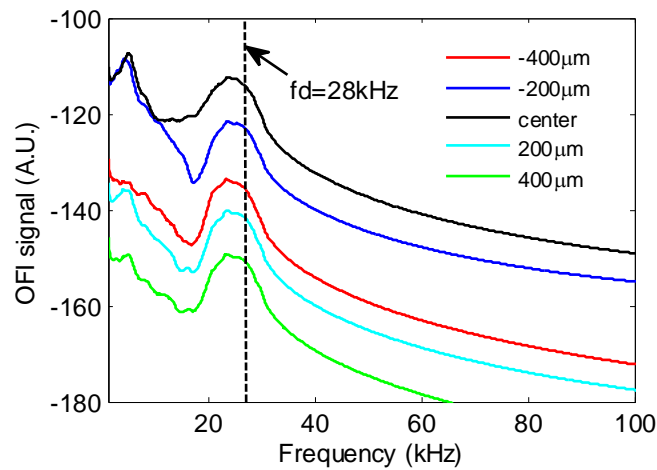
Fig.3.23. Simulated OFI spectra in different laser focus depth positions (from -400, -200, 0(center), +200, 400 \mu\text{m} reference to the channel center) at Q=10\mu\text{L}/\text{min} . The black dashed line denotes the frequency corresponding to the maximal velocity.
