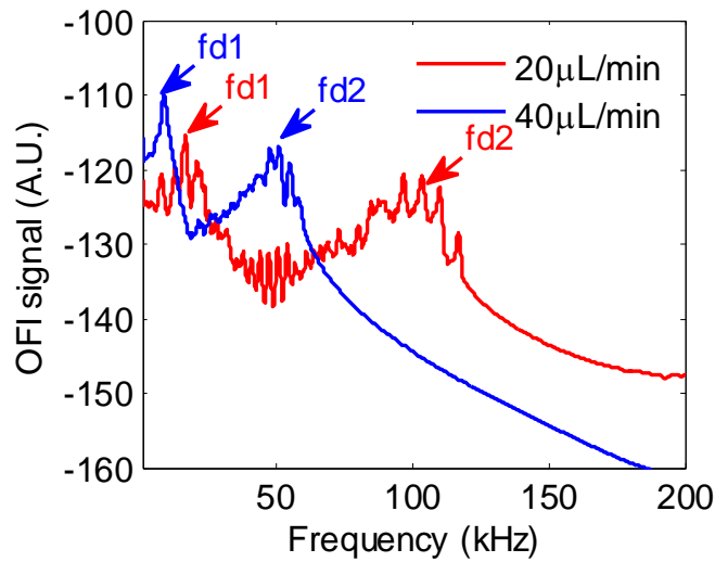
Fig. 2.24. Simulated OFI spectra in 20 \mu L/min and 40 \mu L/min.
