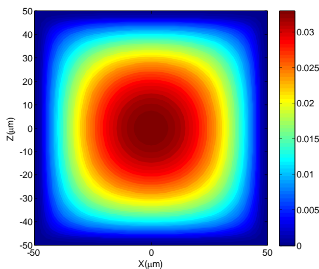
Fig.2.12.2D flowing velocity profile of the cross-section plane in a 100\mu\text{m} \times 100\mu\text{m} channel when the flow rate equals 10\mu\text{L}/\text{min} .
