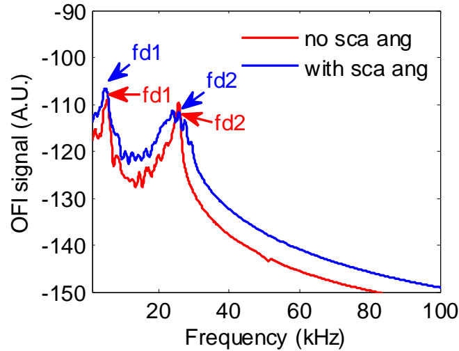
Fig. 2.23. Simulated OFI spectra in 20 \mu L/min and 40 \mu L/min.
