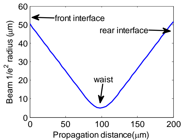
Fig.4.8. Simulated 1/e^2 radius profile during the laser beam propagation inside the 200\mu\text{m} height channel full of water with a micro-scale focusing lens of 80\mu\text{m} diameter 16\mu\text{m} thickness and 53\mu\text{m} curvature radius.
