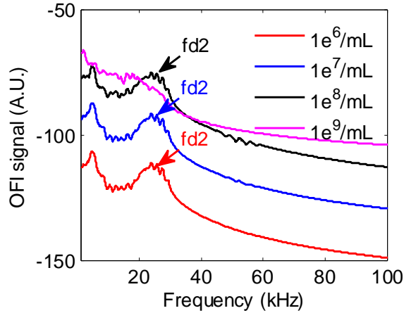
Fig. 2.28. Spectra of different PS concentrations ( 1e^6/mL , 1e^7/mL , 1e^8/mL and 1e^9/mL ).
