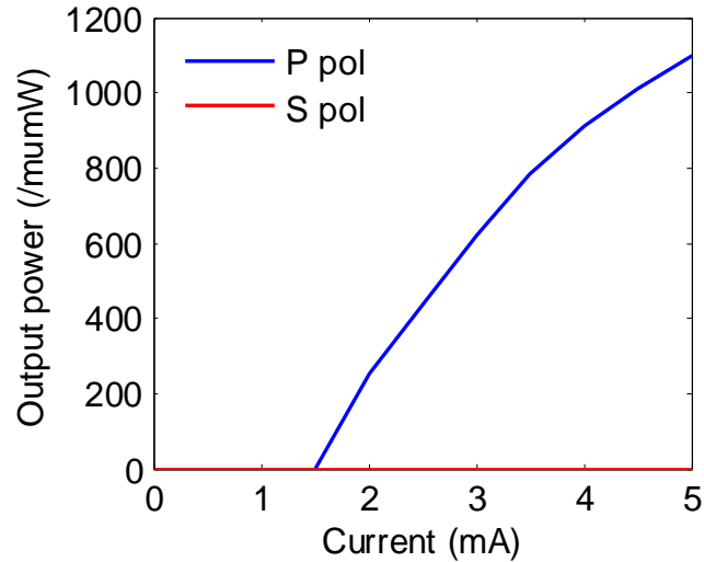
Fig.4.23. Polarization-resolved L-C current of lensed VCSEL. The blue curve is P polarization direction, and red line is S polarization direction which is perpendicular to P direction
