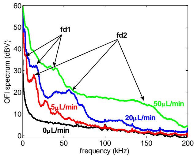
Fig.3.13. Measured OFI spectral of various flow rates: Q=0 \mu\text{L}/\text{min} (in black), Q=5 \mu\text{L}/\text{min} (in red), Q=20 \mu\text{L}/\text{min} (in blue) and Q= 50\mu\text{L}/\text{min} (in green). Both fd1 and fd2 in each flow rate case are denoted as well.
