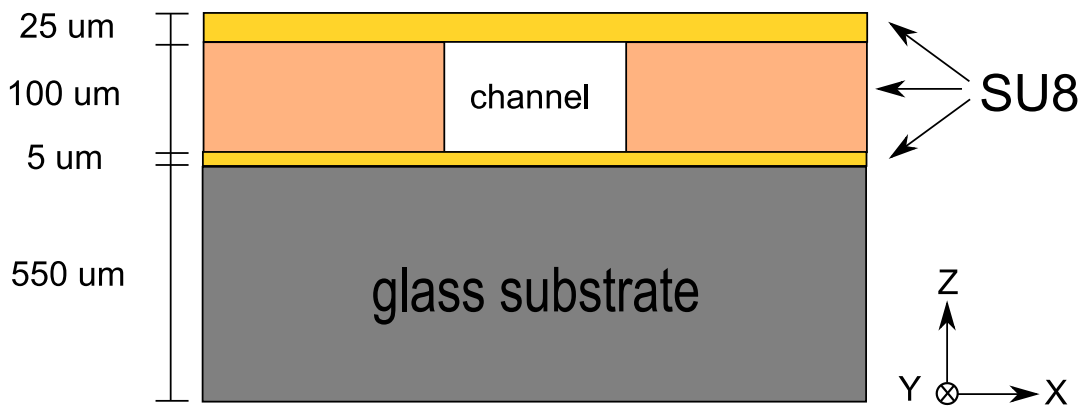
Fig.2.6. Cross-section view of the microfluidic channel chip.
