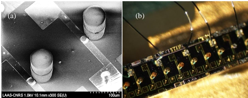
Fig.4.13. (a) SEM image of pedestals integrated on 1×20 VCSEL array mounted on a PCB thanks to double soft thermal printing of 2 DF-1050 films and to laser writing. (b) Optical image of the array after bonding.
