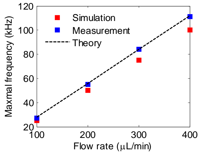
Fig.3.9. Maximal frequency trend versus flow rate inside 1\text{mm}\times 1\text{mm} PDMS channel. Simulations are the red square marks, measurements are the blue square makers. Black dashed line expresses the theoretical value.
