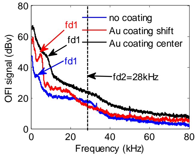
Fig.3.21. Measured spectra of 4.89 \mu\text{m} PS particles inside DF channels in Q=10\mu\text{L}/\text{min} . Blue: non-coating channel center; black: Au coating at channel center; red: Au coating with a lateral position shift; The dashed line denotes the theoretical maximal frequency 28 kHz.
