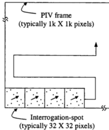
Fig.1.11. Correlation-based PIV process in a 32×32 pixel interrogation spot system, plotting the flow vectors[40].
