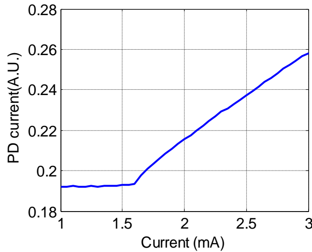
Fig.3.2.The light-current characteristic of the PS67-FIP1U-4U-AC 670 nm VCSEL.
