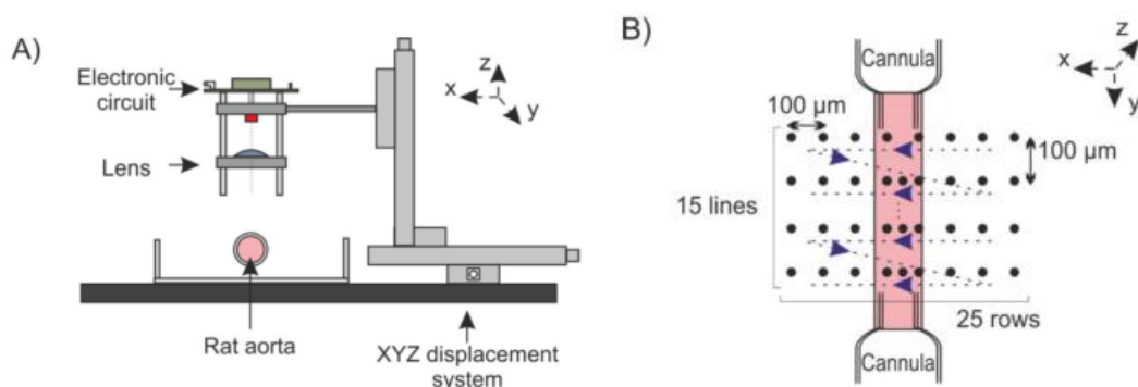
Fig.1.21. OFI based myograph system: A) Lateral view of setup. B) Top view of the aorta scanning[94].
