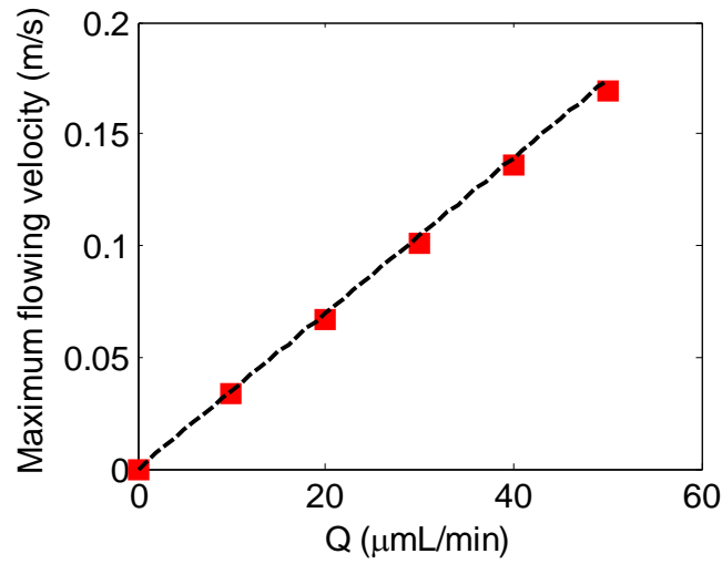
Fig.2.14. Maximal flowing velocities as a function of flow rate ranging from 0 to 50 \mu\text{L}/\text{min} . The red square markers denote the simulated results, and the black dashed line represents the calculation from eq(2.38).
