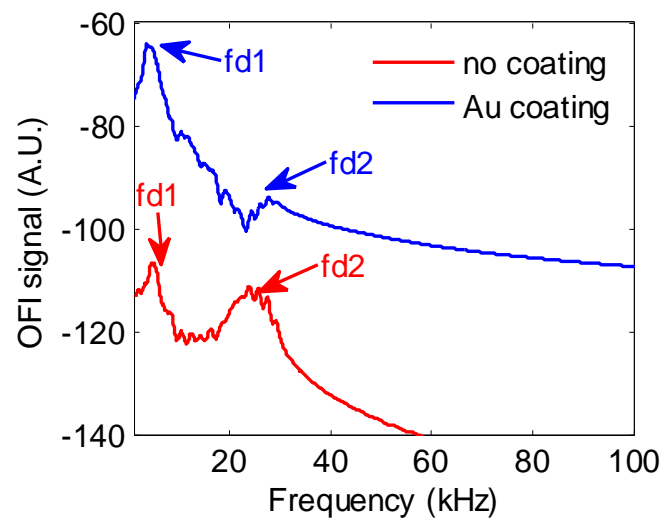
Fig.3.20. Simulated spectra of 4.89\mu\text{m} PS particles inside DF channels in Q=10\mu\text{L}/\text{min} . Blue: Au coating; red: non-coating.
