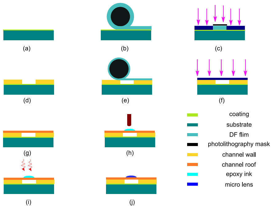
Fig.4.26. Channel chip fabrication procedure: (a) SAM grafting (b) first DF film lamination (c) UV exposure (d) development (e) second film lamination (f) UV exposure (g) photolithography and FDTS grafting (h) microlens inkjet printing and (i) thermal curing.
