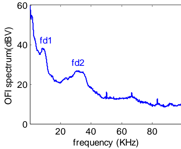
Fig.3.12. Measured OFI spectrum inside the 100\mu\text{m}\times 100\mu\text{m} SU-8 channel at Q=10\mu\text{L}/\text{min} .
