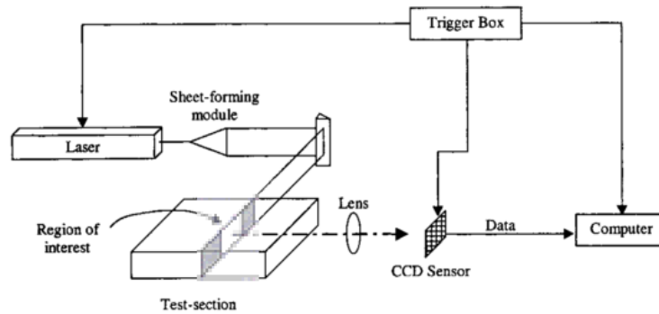
Fig.1.9. Basic setup of a PIV system [40].
