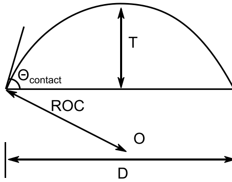
Fig.4.5.Geometrical parameters of the microlens.
