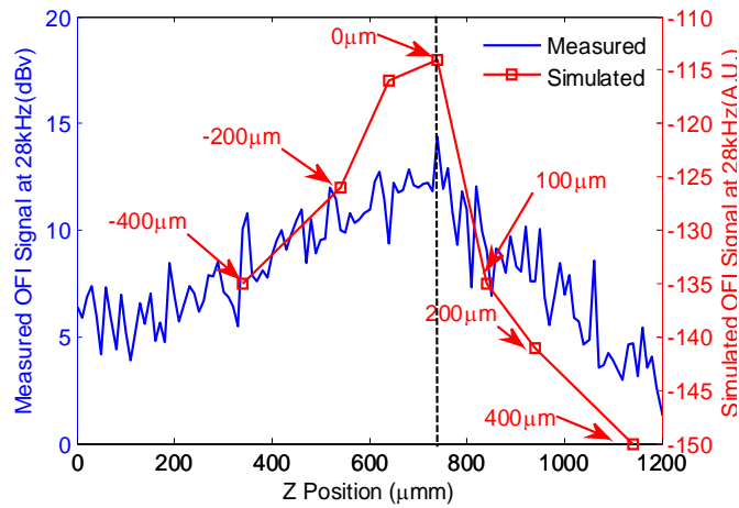
Fig.3.25. OFI signal levels at the maximal Doppler frequency ( fd=28\text{kHz} ): simulation: red line (the red square markers show the simulation positions refer to the channel center). Measurement: blue line; the channel center position: the black dashed line.
