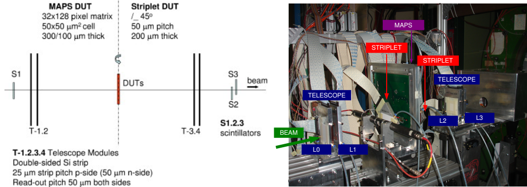
Figure 3.8: (left)The SLIM5 Beam Test Setup. (right)Picture of the SLIM5 demonstrator at the T9 facility of the CERN PS in September 2008. The telescope, 2 striplets modules and one Apseld4D are visible.
