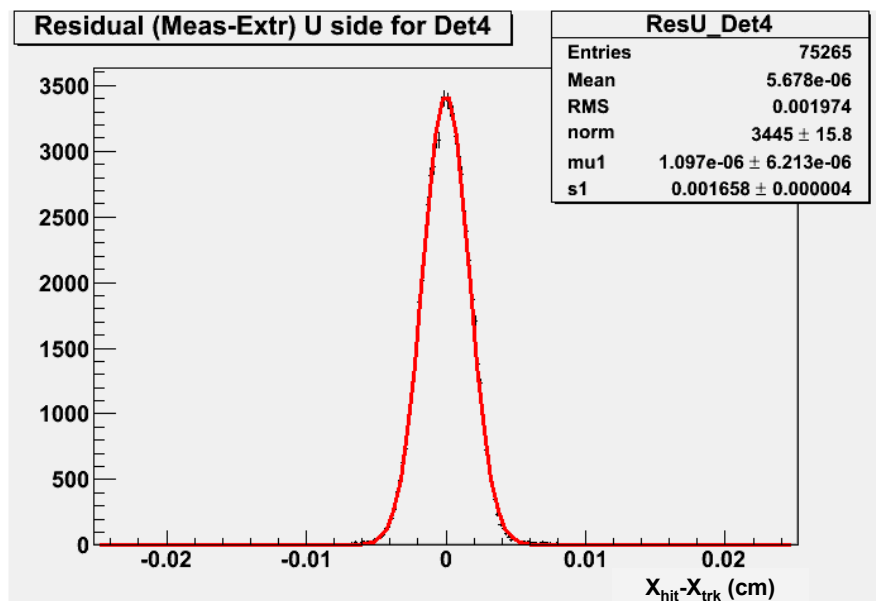
Figure 3.12: Residuals distribution for hits registered on the p -side of a triplet module. Points are data, the red line is the result of a Gaussian fit to the distribution.
