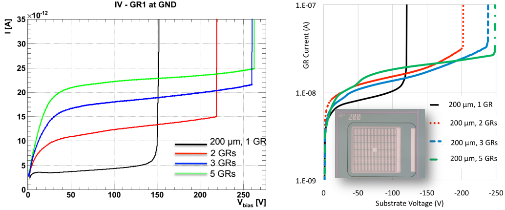
Figure 4.2: IV curves for edgeless n-on-p pixel test structures. (left) TCAD simulations (right) Real data from [7]. Detectors with the same pixel-to-edge minimal distance and different number of GRs are compared. In the right figure a photo of the tested detector is shown in the inset. Vertical scales are different due to the simulated detector area which is smaller than the real one.
