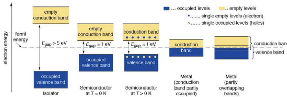
Figure 2.3: Energy band structure of several materials. For semiconductors the T = 0 K and T > 0 K situations are reported; for metals two possible band configurations are represented (After [31]).
