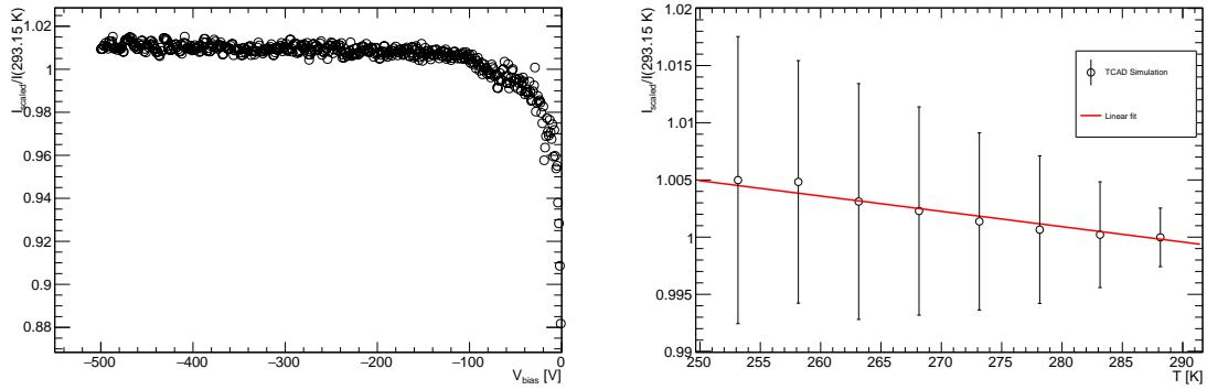
Figure 4.12: (Left) ratio of IV curve at t = -20^\circ \text{C} to the one at t = 20^\circ \text{C} after the former has been rescaled to t = 20^\circ \text{C} . (Right) Average ratio of scaled currents to reference one as a function of the temperature. Both plots were created under the default scenario.
