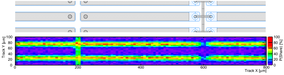
Figure 7.12: Top: Design of the sample of the region shown in the plot below. Bottom: Charge sharing probability for DO9 at V_{bias}=1200V . Note the reduced charge sharing in the bias grid region on the right-hand side of the central pixel.
