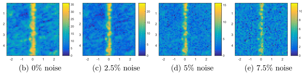
Figure 2.7: Effect of noise on the reconstruction. The parameters are the same used in Figure 2.4b.
