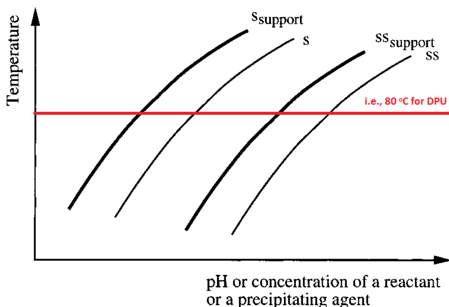
Figure 2-2: Phase diagram of precipitation and dissolution equilibrium of metal species in solution as a function of temperature and concentration of a reactant: in a pure solution (solid lines) and in the presence of a support in solution (bold lines) [7]
