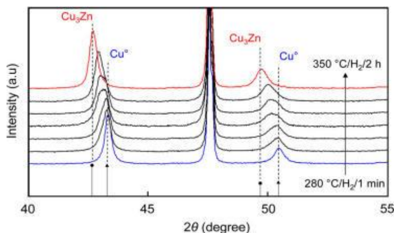
Figure 1-8: XRD patterns (in the range 2\theta=40-55^\circ ) of sample 10 wt% Cu/ZnO sample calcined at 400^\circ\text{C} followed by \text{H}_2 reduction at different temperatures and for different times: 1 min at (a) 280^\circ\text{C} , (b) 330^\circ\text{C} , (c) 340^\circ\text{C} , and (d) 350^\circ\text{C} , and T_R=350^\circ\text{C} for (e) 5 min, (f) 30 min, and (g) 2 h. ▲ and ●: the most intense peaks from the JCPDS files of \text{Cu}^0 (#04-0836) and \text{Cu}_3\text{Zn} (#65-6567), respectively [104].
