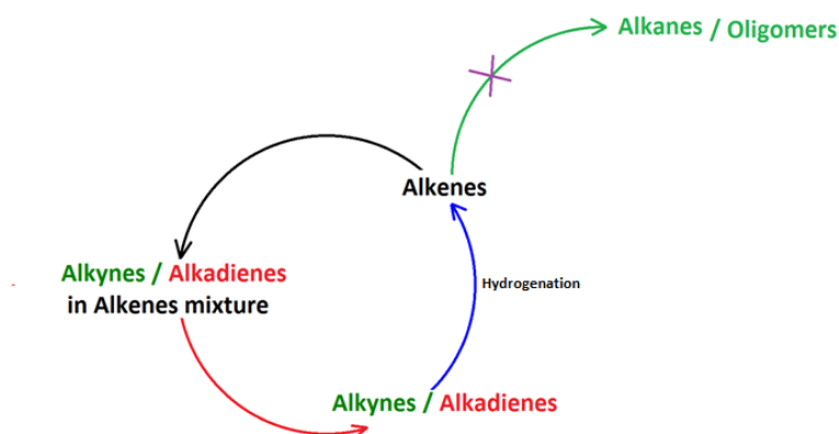
Figure 1-1: a net for increasing alkenes concentration by selective hydrogenation of alkynes impurities
