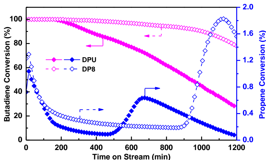
Figure 4-14: Evolution of the conversion of butadiene and propene with time on stream at 105 °C for the DPu and DP8 \text{CuZn 1:1/TiO}_2 catalysts.
