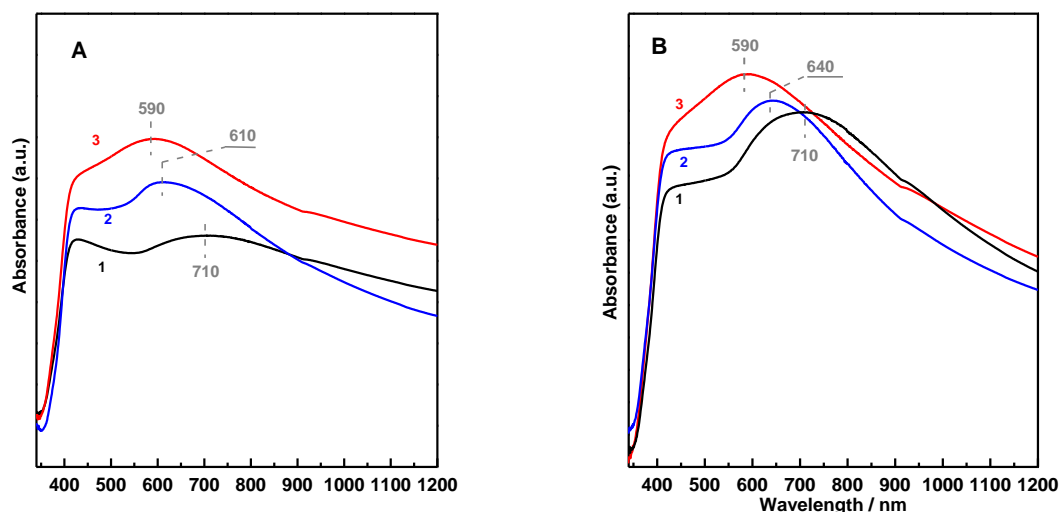
Figure 4-6: UV-visible spectra of the calcined-reduced DPu (A) and DP8 (B) samples: 1, \text{Cu}/\text{TiO}_2 ; 2, \text{CuZn } 3:1/\text{TiO}_2 ; 3, \text{CuZn } 1:1/\text{TiO}_2 ;
