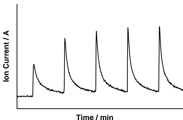
Figure 2-9: calibration of mass spectrometry for \text{NH}_3 desorption
