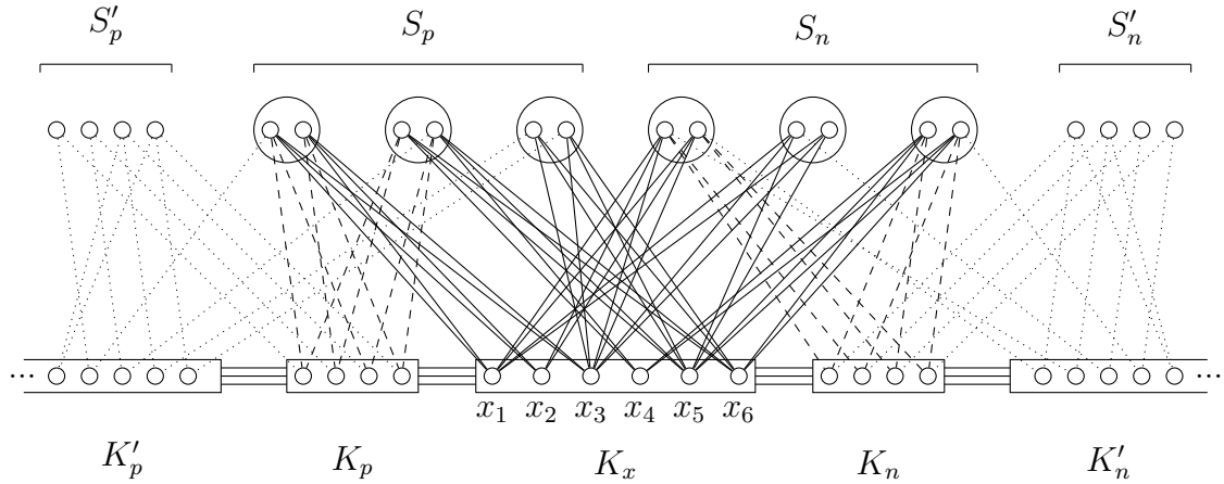
Figure 6.2: The split graph G defined from the instance I = (X, C) with X = \{x_1, x_2, x_3, x_4, x_5, x_6\} and C = \{x_1 \vee x_2 \vee x_3, x_4 \vee x_5 \vee x_6, x_3 \vee x_5 \vee x_6, \overline{x_1} \vee \overline{x_2} \vee \overline{x_3}, \overline{x_1} \vee \overline{x_3} \vee \overline{x_5}, \overline{x_4} \vee \overline{x_5} \vee \overline{x_6}, \}
