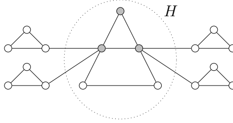
Figure 3.5: A graph in which the subset H is a lambda set but not an LS set.
