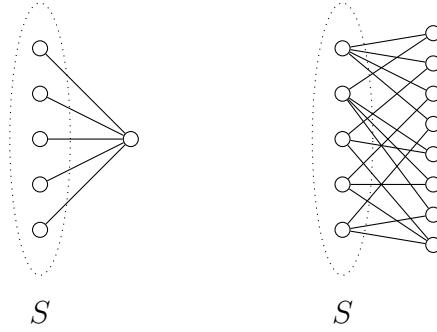
Figure 7.2: Two graphs in which S is an independent 2-clique.
