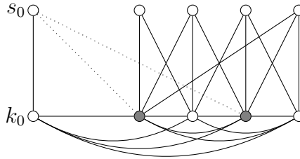
Figure 6.3: The graph G' and a set of edges (represented by dotted lines) of minimum size to add to make G' having diameter 2 (a minimum dominating set is given in gray).
