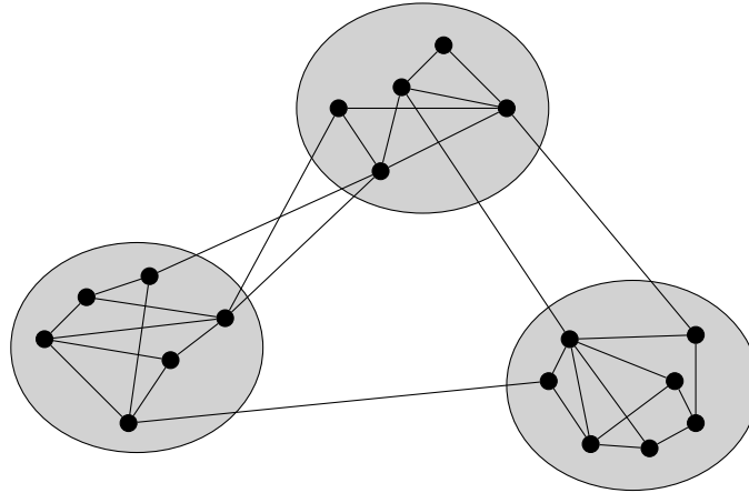
Figure 3.1: A social network partitioned into intuitive communities
