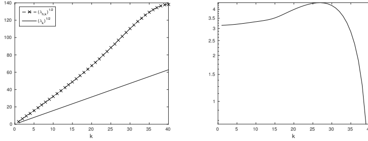
FIGURE 22 – Comparaision between the behaviour of the square roots of the eigenvalues associated to (4.5.7) and the behaviour of the continuous ones (left) and behaviour of the gap \sqrt{\lambda_{h,k+1}} - \sqrt{\lambda_{h,k}} > k = 1, \dots, N-1 (right) for N = 40 and \gamma = 3
