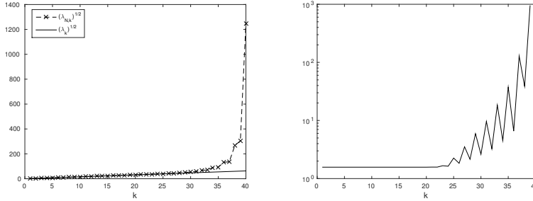
FIGURE 15 – Comparaision between the behaviour of the square roots of the eigenvalues associated to (4.5.7) and the behaviour of the continuous ones (left) and behaviour of the gap \sqrt{\lambda_{N,k+1}} - \sqrt{\lambda_{N,k}} > k = 1, \dots, N - 1 (right) for N = 40 and \gamma = 1
