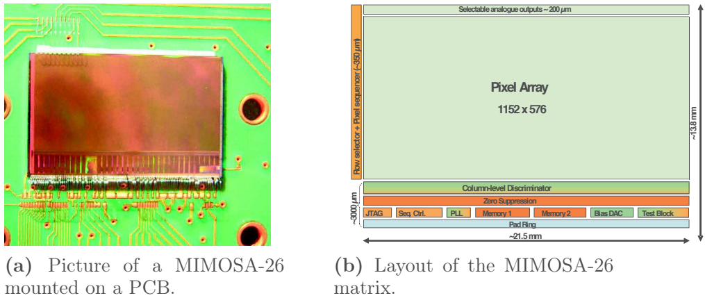
Figure 4.16 – Block-diagram and a picture of the MIMOSA-26
