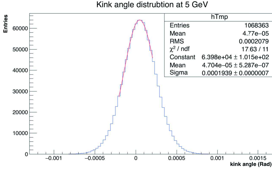
Figure 7.9 – Distribution of the kink angle \theta_0 given by GBL for an energy of 5 GeV without any fiducial cut. The asymmetry of the distribution arises from an incorrect alignment procedure.
