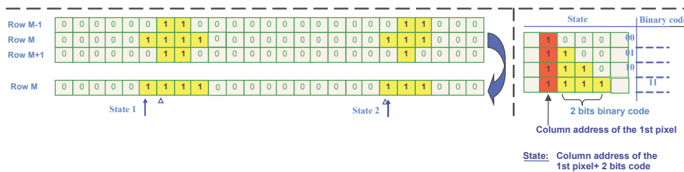
Figure 4.14 – Principle of the zero suppression logic.
