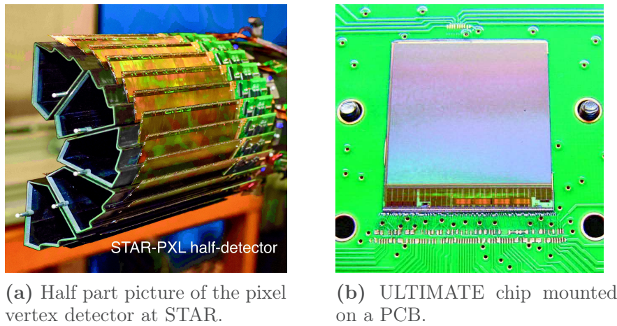
Figure 4.17 – Pictures of the STAR vertex detector and an ULTIMATE chip
