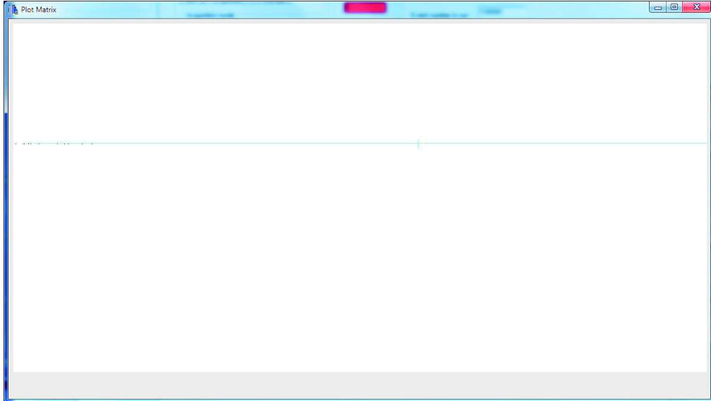
Figure 5.9 – Matrix response in discriminator mode, where all the discriminators are closed. One line of pixels is always activated, as well as few pixels in one column. This will increase the fake hit rate of the sensor.
