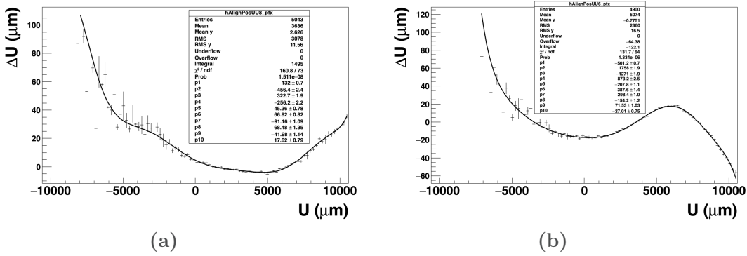
Figure 6.9 – Profile of the scatter plot showing the track-hit residual in the u -direction as a function of the hit position on the plane for the same direction: 6.9a shows the profile of the front plane and 6.9b shows the profile of the back plane. Both profiles were fitted with a sum of Legendre polynomials up to the eleventh order. p1 to p10 are the coefficients \omega_k of equation 6.4 of the polynomials.
