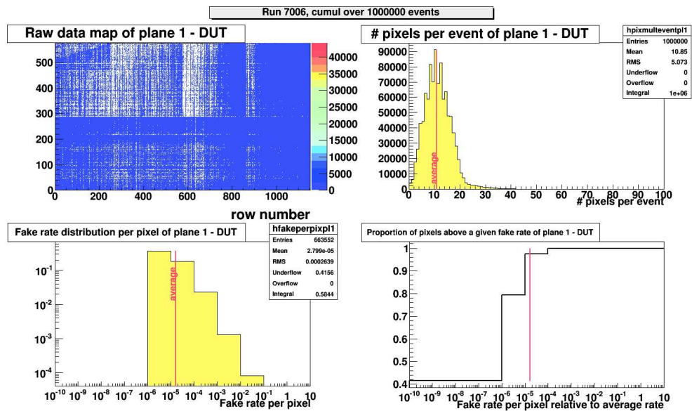
Figure 5.14 – Results of the fake hit rate measurement for a threshold three times bigger than the noise. The top left plot represents a raw picture of the million events accumulated over the whole matrix. The top right one is the distribution of the number of pixels hit per event. The bottom left plot is the fake hit rate per pixel distribution, while the bottom right one is the fake hit rate relative to the average rate distribution.
