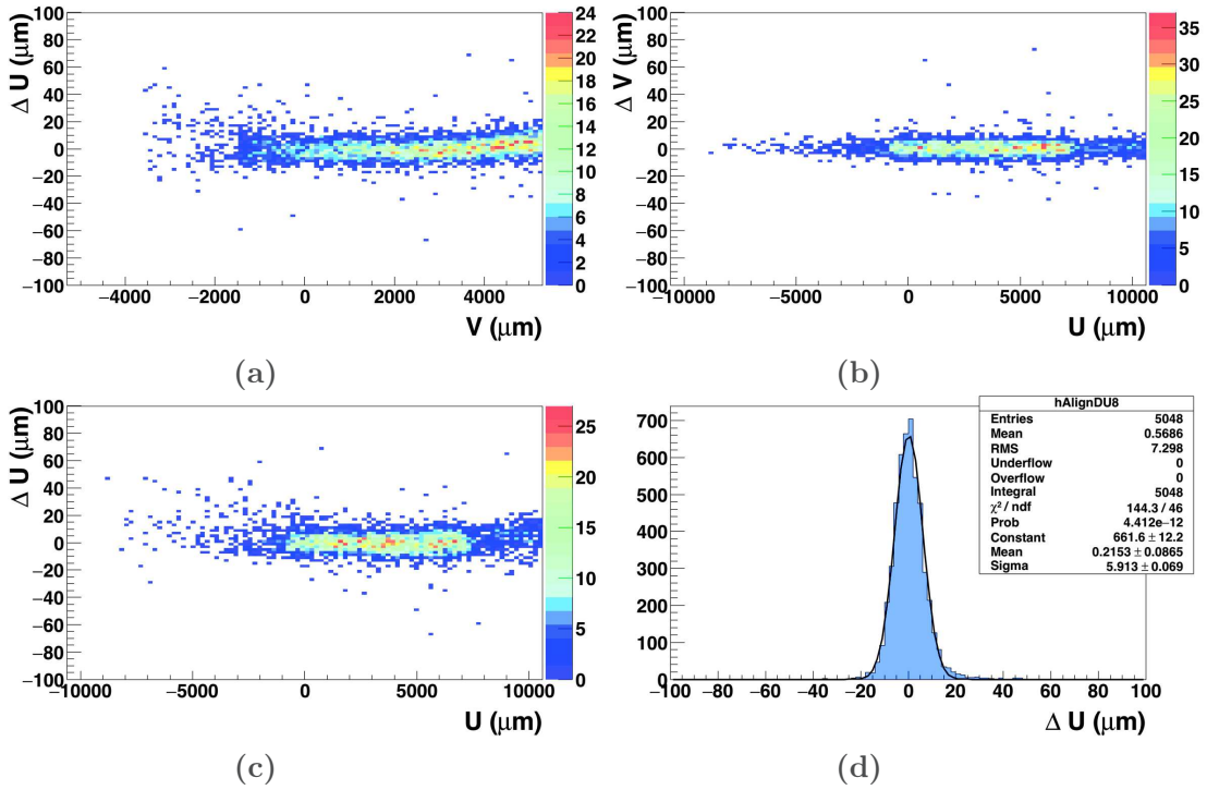
Figure 6.10 – Results of the alignment after applying the Legendre polynomial correction and taking into account the angle of the incoming particles for the front sensor: 6.10c \Delta u = f(u_{\text{hit}}) and 6.10d distribution of the residuals.
