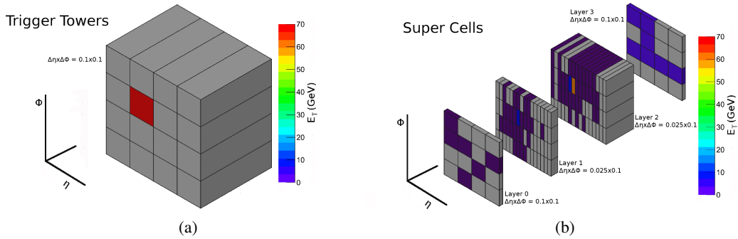
Figure 37: An electron (with 70 GeV of transverse energy) as seen (a) by the existing L1 calorimeter trigger electronics and (b) by the upgraded trigger electronics [30].
