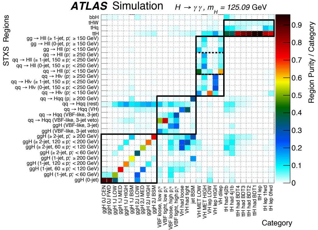
Figure 26: The fraction of signal events assigned to each reconstructed category ( x axis) and originating from a given region of the stage-1 simplified template cross section framework ( y axis). The black lines separate the t\bar{t}H and tH , VH leptonic, VH hadronic and VBF enriched, and untagged categories, along with the simplified template cross-section regions they are most sensitive to. The color shows the purity of the region per category [24].
