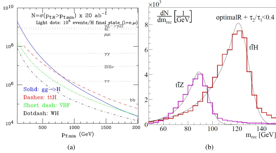
Figure 48: (a) Integrated Higgs boson transverse momentum rates, for various production channels, with 20 \text{ ab}^{-1} [43]. (b) Reconstructed m_{bb} invariant mass of the Higgs boson and Z boson candidates in a boosted topology [42].
