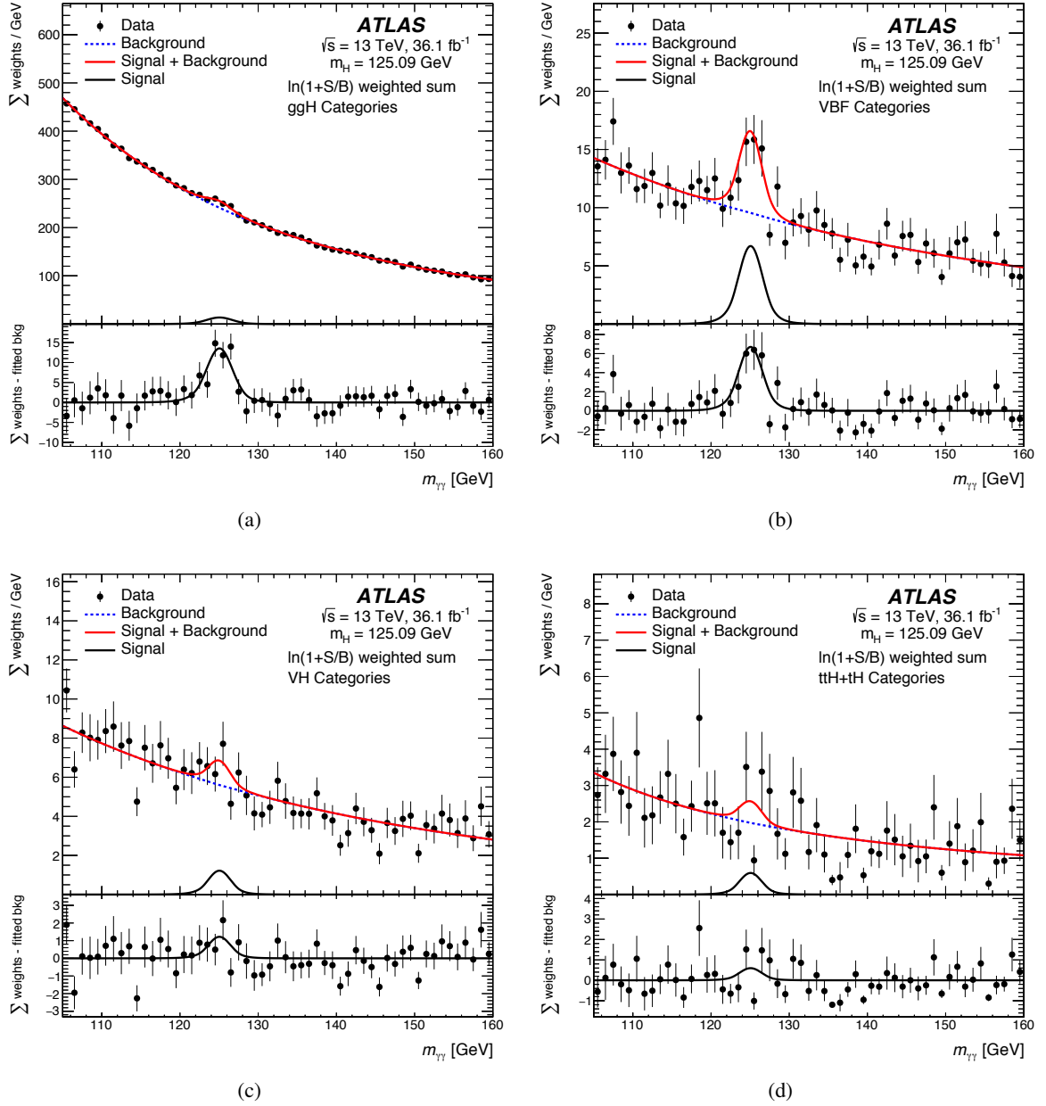
Figure 29: Weighted (from the expected signal to background ratio in each category) diphoton invariant mass spectra observed in the 13 TeV data for events belonging to: (a) ggF categories (b) VBF categories, (c) VH categories and (d) t\bar{t}H categories [24]. The bottom inserts show the residuals between the data and the background component of the fitted model.
