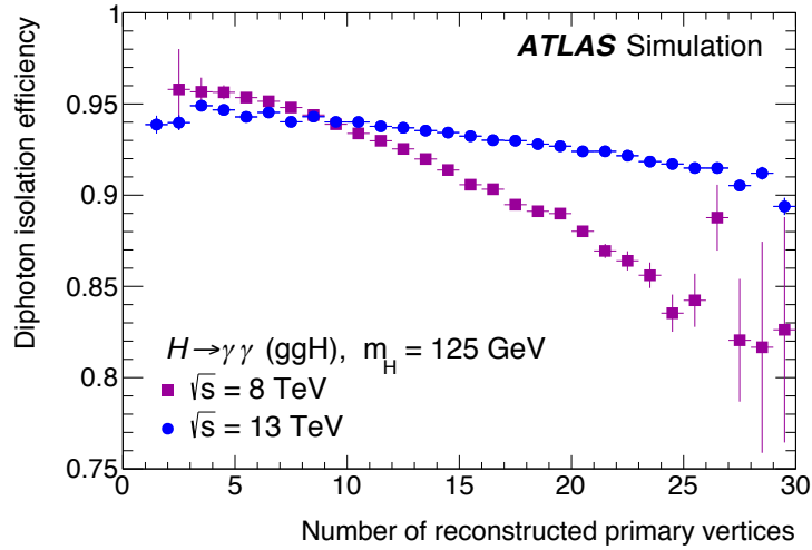
Figure 25: Efficiency for both photons to fulfill the isolation requirement as a function of the number of primary vertex candidates in each event (estimated on a simulation sample of ggF events) [24].
