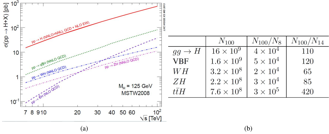
Figure 47: (a) Higgs boson production cross sections as a function of the centre-of-mass energy [6]. (b) Indicative total event rates at 100 TeV ( N_{100} ), and statistical increase with respect to the statistics of LHC Run 1 ( N_8 ) and HL-LHC ( N_{14} ), for various production channels [43].
