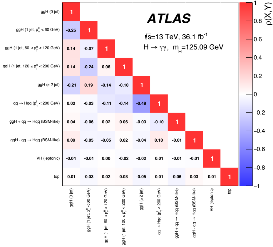
Figure 30: Observed correlations between the measured simplified template cross sections (including both the statistical and systematic uncertainties) [24].
