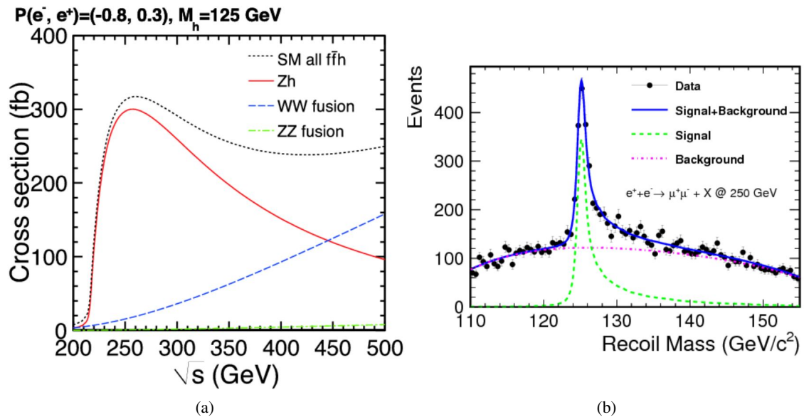
Figure 46: (a) Production cross section for ee \rightarrow ZH , ee \rightarrow \nu\nu H and ee \rightarrow eeH processes as a function of the centre-of-mass energy for m_H = 125 GeV [40]. (b) Recoil mass distribution in the Z \rightarrow \mu\mu case at \sqrt{s} = 250 GeV [41].
