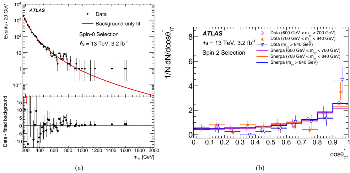
Figure 4: (a) Distribution of the invariant mass of the diphoton candidates for the selection used in the search for a spin-0 resonance with the best background-only fit [5]. The difference between the data and this fit is shown in the bottom panel. (b) Distribution of \cos \theta^* for events in the mass interval 700–840 GeV, and the regions 600–700 GeV or > 840 GeV [5]. This illustrates the countless crosschecks performed in the context of the ‘750 GeV excess’.
