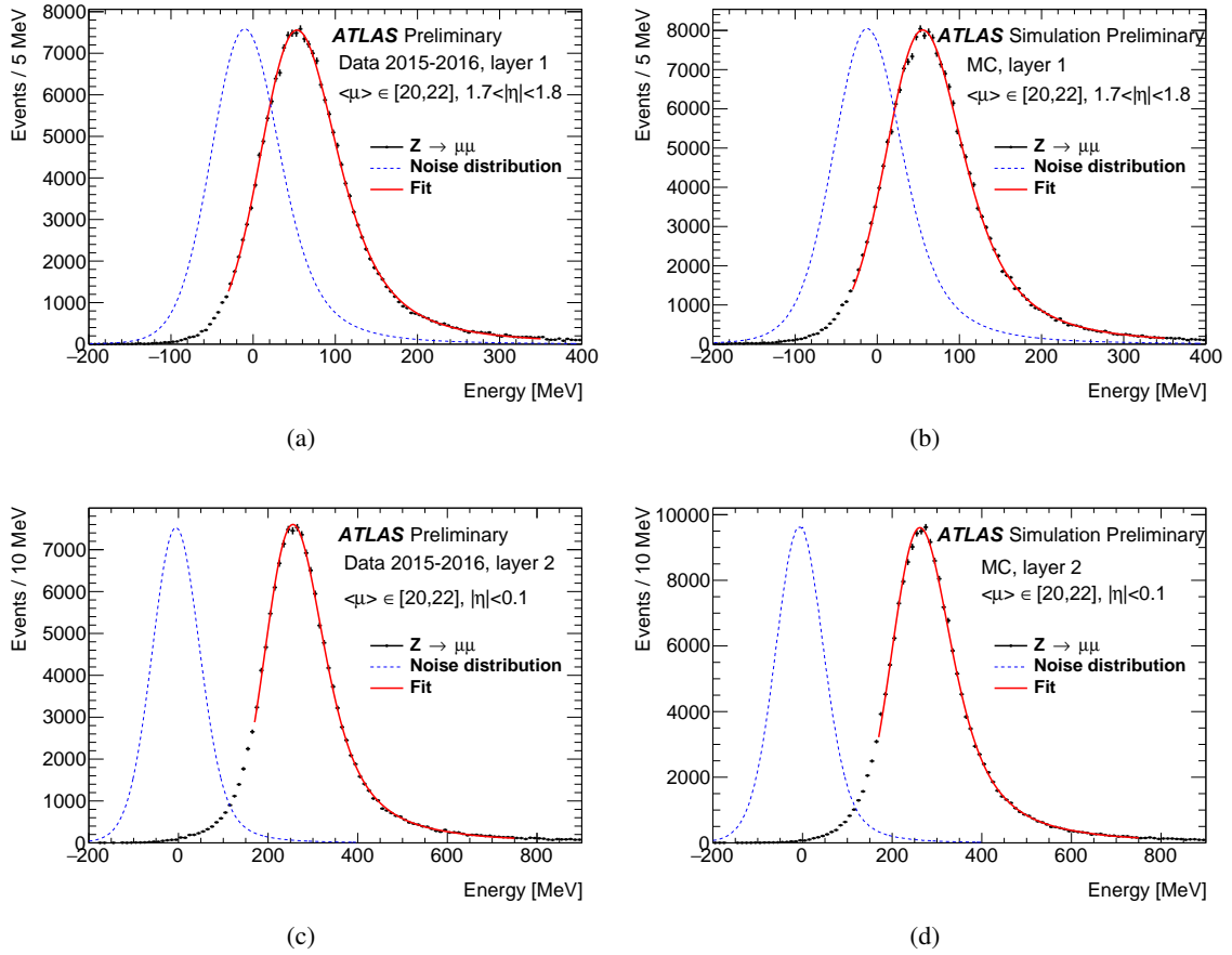
Figure 16: Distribution for one endcap bin of the energy loss by a muon in the first sampling of the EM calorimeter for data (a) and MC (b), and for one barrel bin in the the second sampling of the EM calorimeter for data (c) and MC (d). The results of fits performed with a Landau convoluted to a noise template are overlaid.
