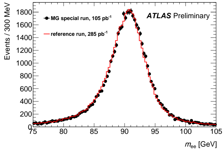
Figure 22: Distribution of the dielectron invariant mass for Z \rightarrow ee candidates recorded in 2017 during LHC fill 6035 (August 2nd, 2017). Data taken with a lower energy transition threshold between the high gain and medium gain for the L2 of the EM calorimeter are compared to data taken in the same LHC fill but with the standard thresholds.
