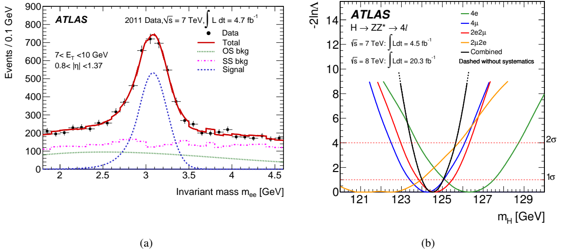
Figure 3: (a) Invariant mass distribution for the J/\psi \rightarrow ee sample in the short-lifetime range, used to measure electron identification at low p_T via a tag-and-probe technique [3]. (b) Profile likelihood as a function of m_H for the combination of all H \rightarrow ZZ^* \rightarrow 4l channels and for the individual channels, for the combined 7 TeV and 8 TeV data samples [4].
