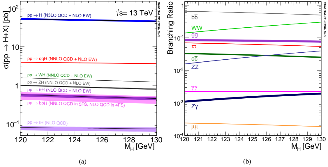
Figure 5: (a) Higgs boson production mode cross sections in proton-proton collisions at 13 TeV [6]. (b) Higgs boson branching ratios [6].
