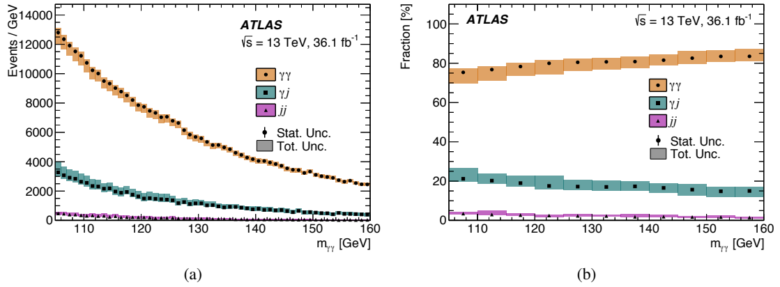
Figure 28: (a) Data-driven background decomposition: event yields (a) and (b) event fractions for \gamma\gamma , \gamma j and jj events as a function of m_{\gamma\gamma} [24].
