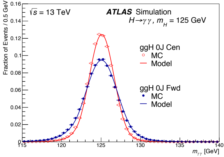
Figure 27: Diphoton mass signal shapes (simulated events and fit models) for two ggF categories [24].
