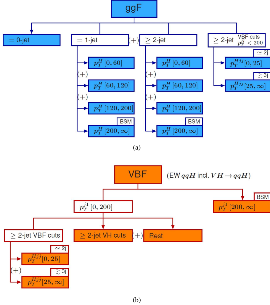
Figure 24: (a) Stage 1 binning for the gluon fusion production [6]. (b) Stage 1 binning for the vector fusion production [6].
