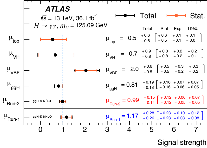
Figure 31: Summary of the signal strengths measured for the different production processes (ggH, VBF, VH and top) and globally ( \mu_{\text{Run-2}} ) [24]. The global signal strength measured at 7 and 8 TeV ( \mu_{\text{Run-1}} ) is also shown [26].
