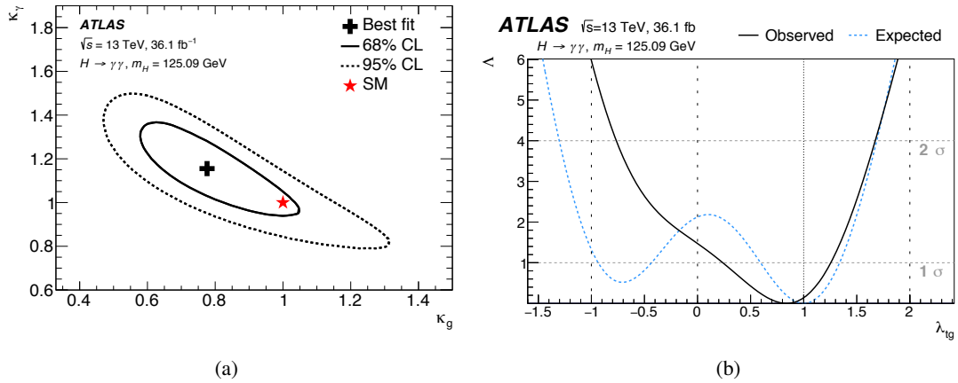
Figure 32: (a) Likelihood contour in the (\kappa_g, \kappa_\gamma) plane compared to the Standard Model prediction (red star) [24]. (b) Likelihood profile of the observed and expected coupling-strength modifier ratio \lambda_{tg} [24].
