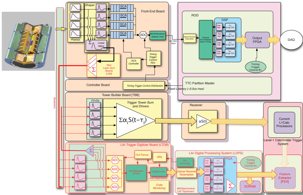
Figure 38: Schematic block diagram of the Phase-I upgrade LAr trigger readout architecture [30]. The new components are indicated by the red outlines and arrows.
