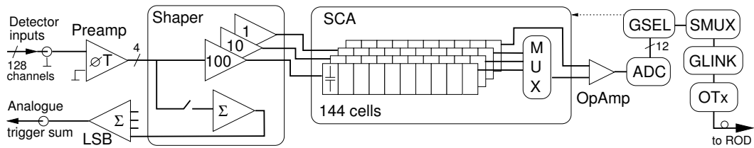
Figure 14: LAr front-end board schematics
