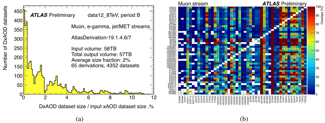
Figure 12: (a) Size of DxAOB (derivation) datasets as a fraction of the size of the parent xAOD datasets. (b) Event-wise fractional overlaps between derivations.
