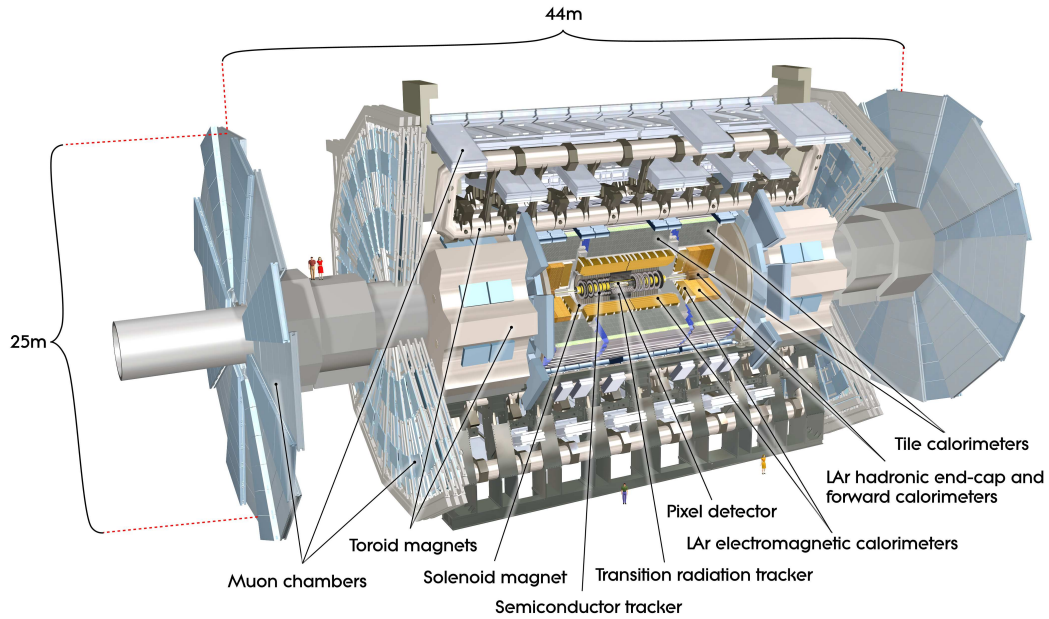
Figure 7: Overall view of the detector
