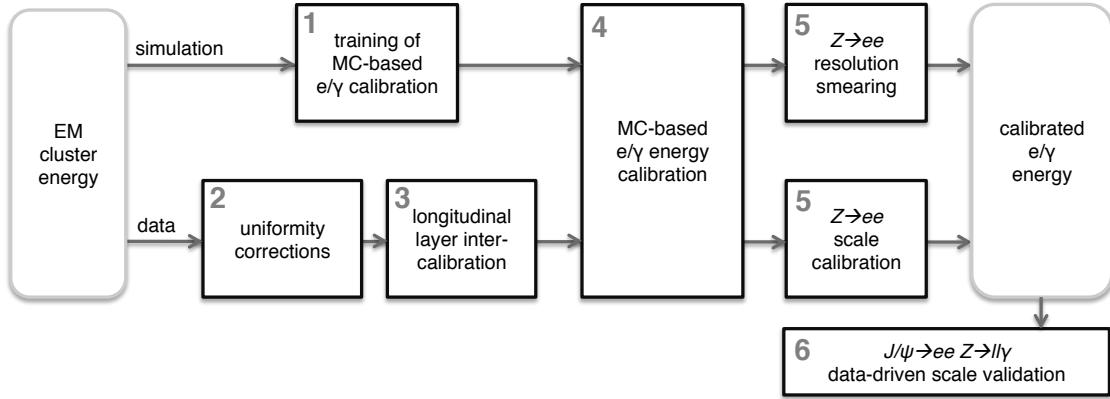
Figure 15: Schematic overview of the procedure used to calibrate the energy response of electrons and photons in ATLAS [21].
