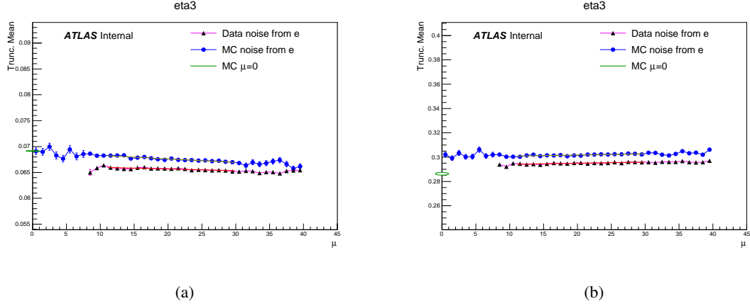
Figure 18: Truncated mean values as function of \mu , extracted from data and MC energy distributions of L1 (a) and L2 (b) for one barrel bin. TM values computed from the corresponding MC sample generated without pileup are also indicated.
