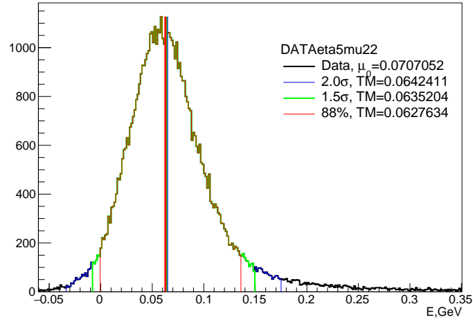
Figure 17: Truncated mean values computed for various range definitions: iterative procedure corresponding to intervals \mu_0 \pm 2 \cdot RMS (nominal case) and \mu_0 \pm 1.5 \cdot RMS where \mu_0 is mean within initial range, and within smallest interval containing 88% of distribution.
