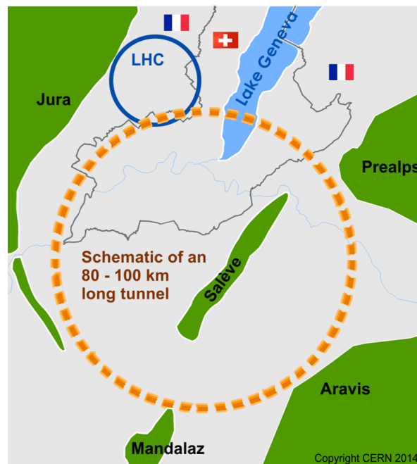
Figure 35: Schematic view of the FCC tunnel infrastructure.
