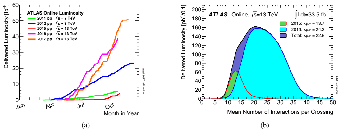
Figure 8: (a) LHC delivered luminosity to ATLAS versus time for the 2011-2017 period (pp collision data only). (b) Mean number of interactions per crossing for the 2015 and 2016 pp collision data.
