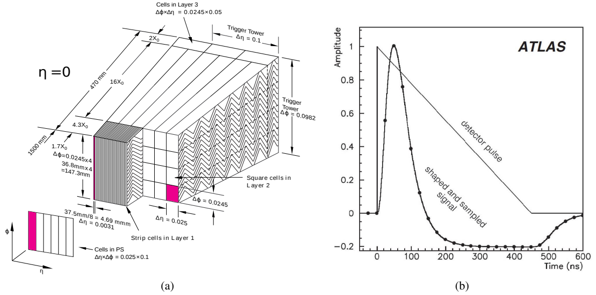
Figure 13: (a) View of the granularity of the LAr calorimeter (barrel part). (b) LAr signal before and after bipolar shaping [19].
