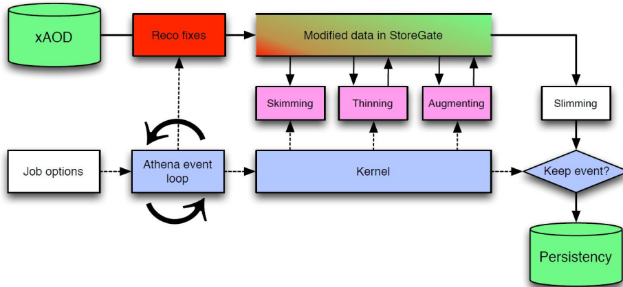
Figure 11: Implementation in Athena of the derivation framework [18]
