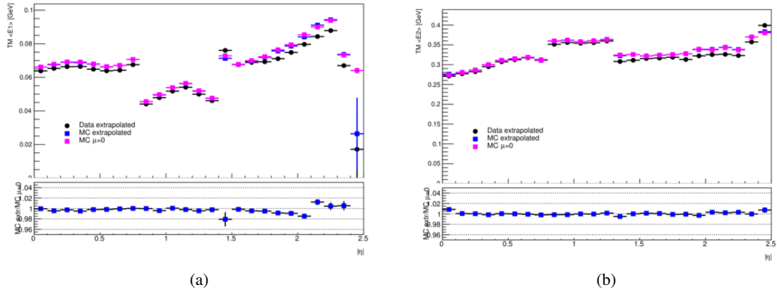
Figure 19: Truncated mean values computed as a function of |\eta| extracted from data and MC after extrapolation to \mu = 0 . The corresponding TM values computed with MC without pileup are also indicated for crosscheck. Ratio panel shows the ratio of extrapolated MC to MC at \mu = 0 .
