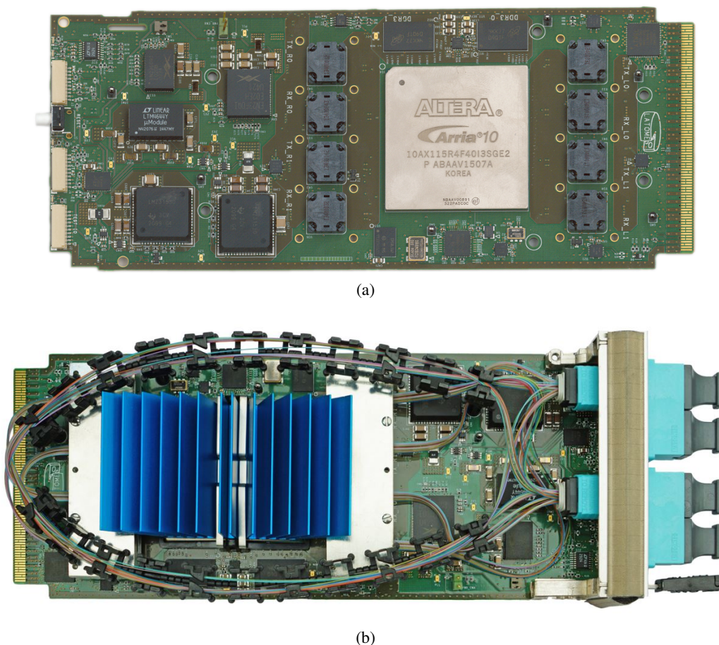
Figure 40: (a) Picture of one bare LATOME board. (b) Picture of one equipped LATOME board.
