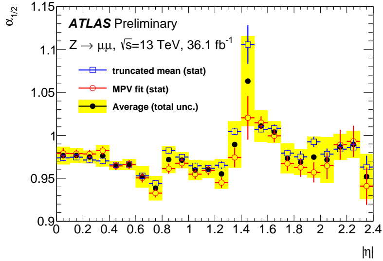
Figure 20: Comparison of the E_{1/2}^{\text{data}}/E_{1/2}^{\text{MC}} double ratio as a function of the corrected |\eta| coordinate for the 2015+2016 dataset. The blue points are the results for the TM method, the red points are the results for the Landau-based fit method and the black points show the average results.
