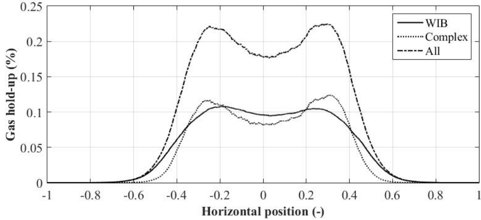
Figure II.16: Void Fraction Profil in Horizontal Direction in the case of Water, Membrane Injection and a Flow Rate of 50 \frac{l}{h}
