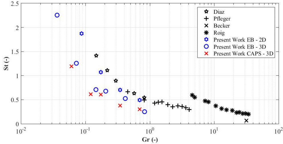
Figure III.56: Strouhal as a function of Grashof in Water
