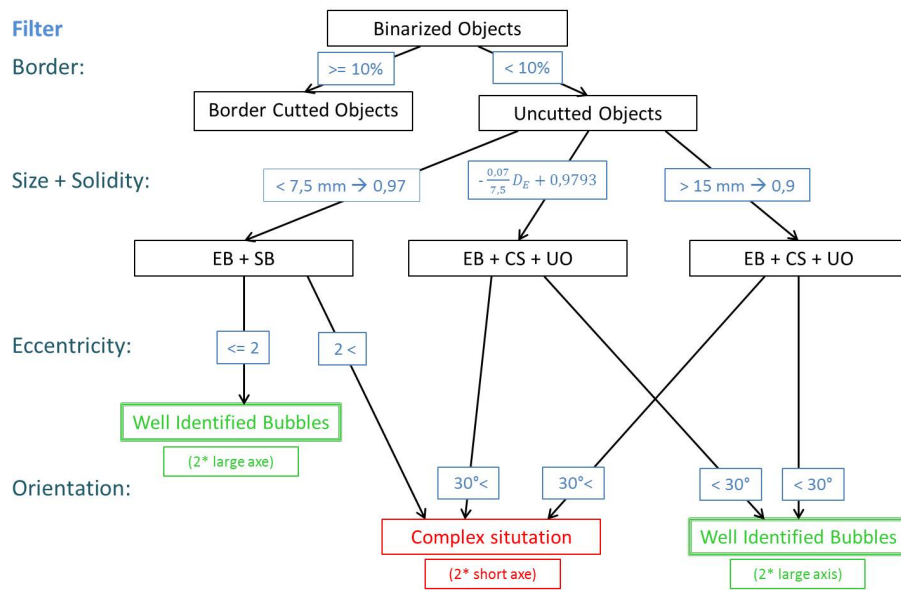
Figure II.8: Scheme of applied filters where: SB = Spherical Bubbles; EB = Ellipsoidal Bubbles; CS = Spherical CAPS; UO = Undefined Objects
