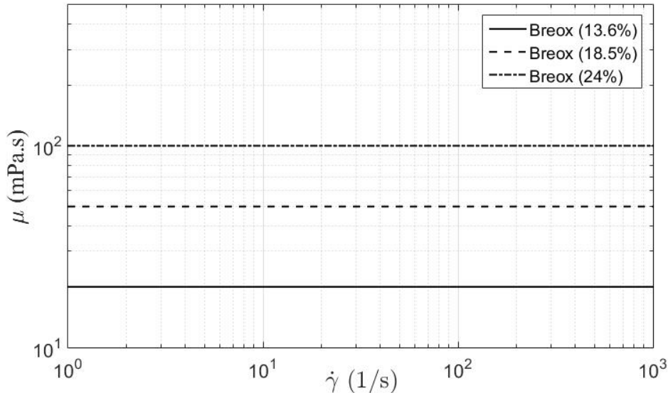
Figure II.2: Dynamic Viscosity as a function of the shear rate in different Fluids: Breox (13.6%) ; Breox (18.5%) ; Breox (24%)
