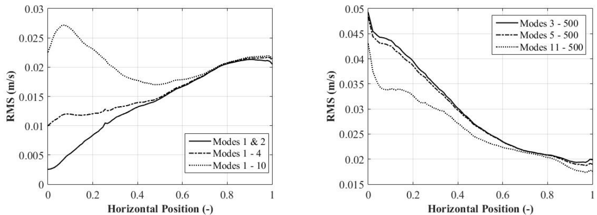
Figure III.27: Reconstructed RMS from POD Treatment for Slugflow Sparger
