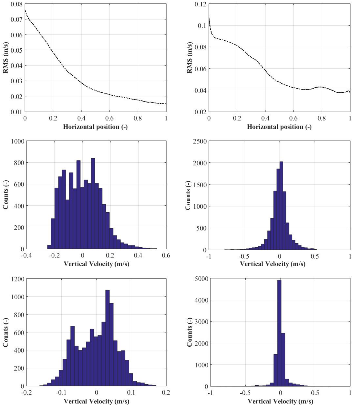
Figure III.34: RMS and Histograms of Velocity in Vertical Direction at X = 0.25 (middle) and X = 0.9 (bottom) in Brex (13.6%) and 50 \frac{l}{h} for Membrane Sparger (left) and Slugflow Sparger (right)
