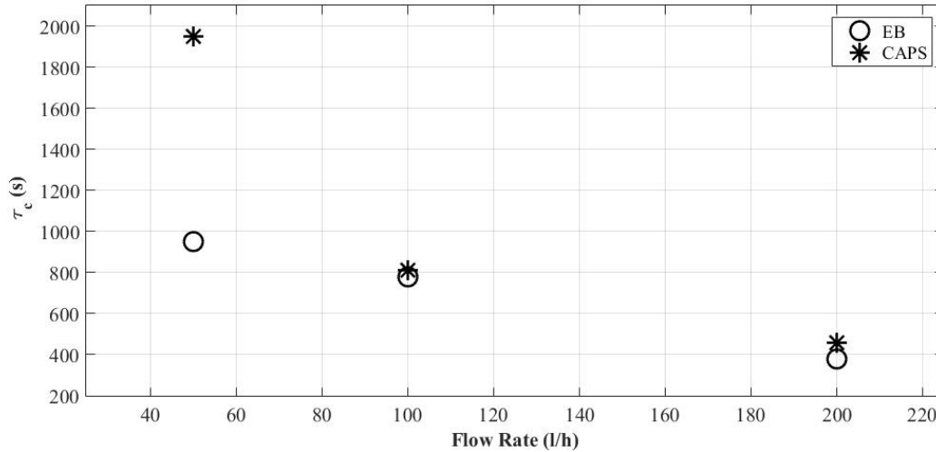
Figure III.53: Mass Transfer Time Scales as a function of the Flow Rate in Water for both Spargers
