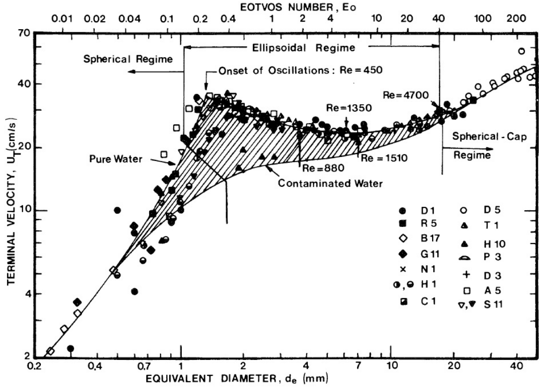
Figure I.2: Terminal Bubble Velocity in function of E\ddot{o} and Re by Grace, Clift & Weber (1978)
