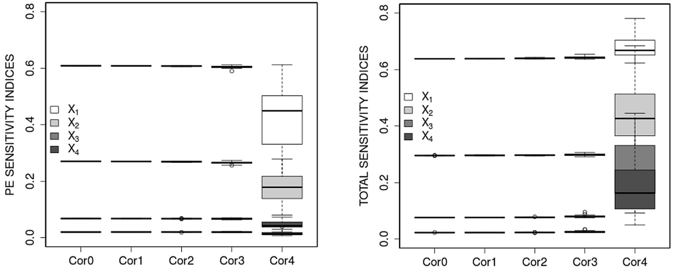
Fig. 2. Sobol' function: influence of the correlation between the inputs on the four PC 5 -PESI(OLS) (left panel where the y-axis "PE Sensitivity Indices" represents the four PC 5 -PESI(OLS)), and the four PC 5 -TSI(OLS) (right panel where the y-axis "Total Sensitivity Indices" represents the four PC 5 -TSI(OLS)). The same comment about the x-axis as in Fig. 1 applies here as well. Cor0 = 0 stands for non-correlated inputs, and correct estimations of the analytical solutions of the analytical solutions of the First-Order Sensitivity Indices for the independent X 1 , X 2 , X 3 and X 4 are then obtained in this case. We recall these analytical solutions here: the First-Order Sensitivity Indices for the independent X 1 , X 2 , X 3 and X 4 are 0.6037, 0.2683, 0.0671 and 0.0200, respectively, and the Total Order Sensitivity Indices for X 1 , X 2 , X 3 and X 4 are 0.6342, 0.2945, 0.0756 and 0.0227, respectively.
