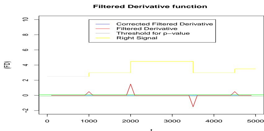
FIGURE 2.3 – Filtered Derivative function without noise ( \sigma = 0 ).
