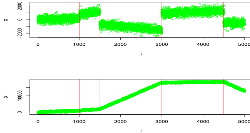
Figure 2.15: The linear regression with four change points on the slope and no change on the intercept.
