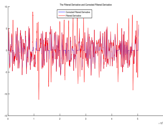
FIGURE 2.13 – The Filtered Derivative and Corrected Filtered Derivative
