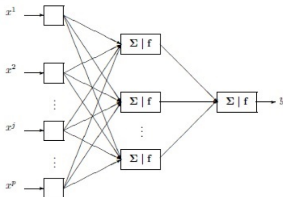
FIGURE 4.2 – Perceptron Multicouche
