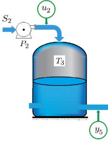
Figure 4.5: Scheme and equations of subsystem \Sigma_3 .
