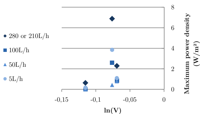
Figure 30. Maximum surface power density vs logarithm of the volume.
