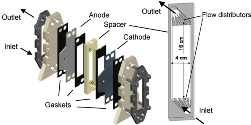
Figure 15. Filter-press reactor (modified from Rivero et al. 128 ).
