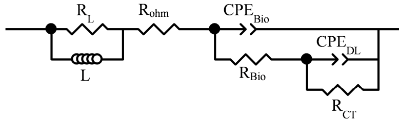
Figure 19. Electrical equivalent circuit used to fit anode impedance spectra. L: inductance; R_L : resistance from inductive behavior; R_{ohm} : electrolyte resistance; R_{CT} : charge transfer resistance; R_{Bio} : biofilm resistance; CPE_{DL} & CPE_{Bio} : constant phase elements respectively from double layer and biofilm.
