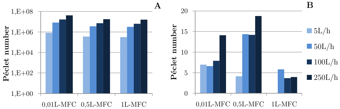
Figure 31. Calculated Péclet number from theoretical expression (A) and Péclet number extracted from RTD experiment (B).
