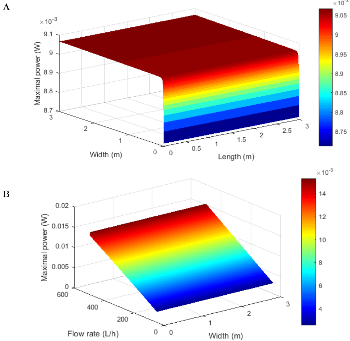
Figure 34. Simulation of maximal power generated by changing the length, the width and the flow rate applied to the flat-plate air-cathode MFC used in this work, at a constant flow rate of 280 L/h (A) or at a constant length of 0.35 m (B).
