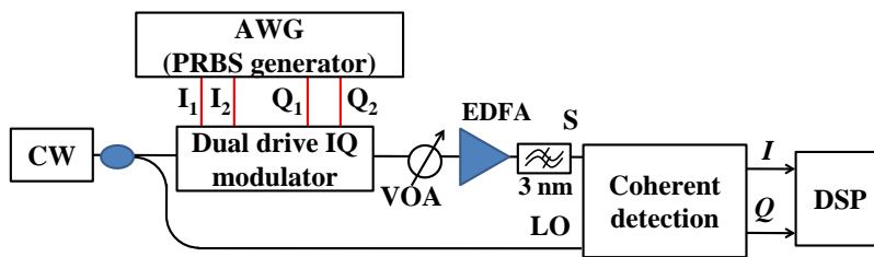
Figure III.4: Experimental setup for characterizing the quadrature imbalance compensation in a QPSK coherent system.
