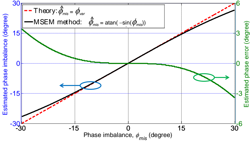
Figure III.1: Analytical prediction of the estimated phase imbalance values for different predefined phase imbalance values using the proposed MSEM method and their corresponding estimated phase error.
