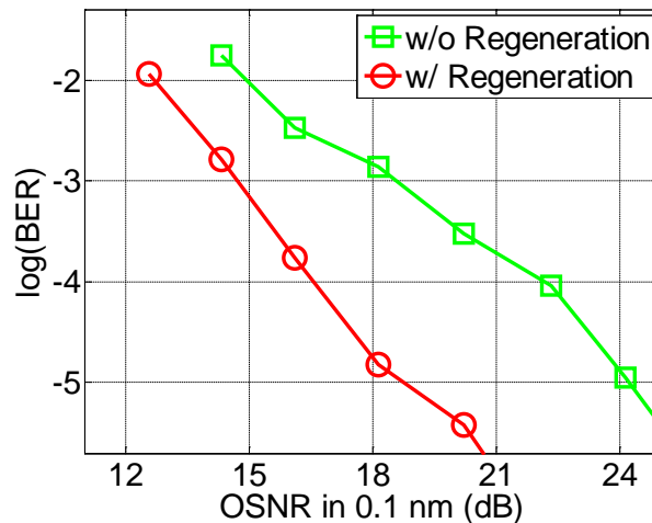
Figure III.34: BER versus input OSNR ( P_{rec} = -20 dBm).
