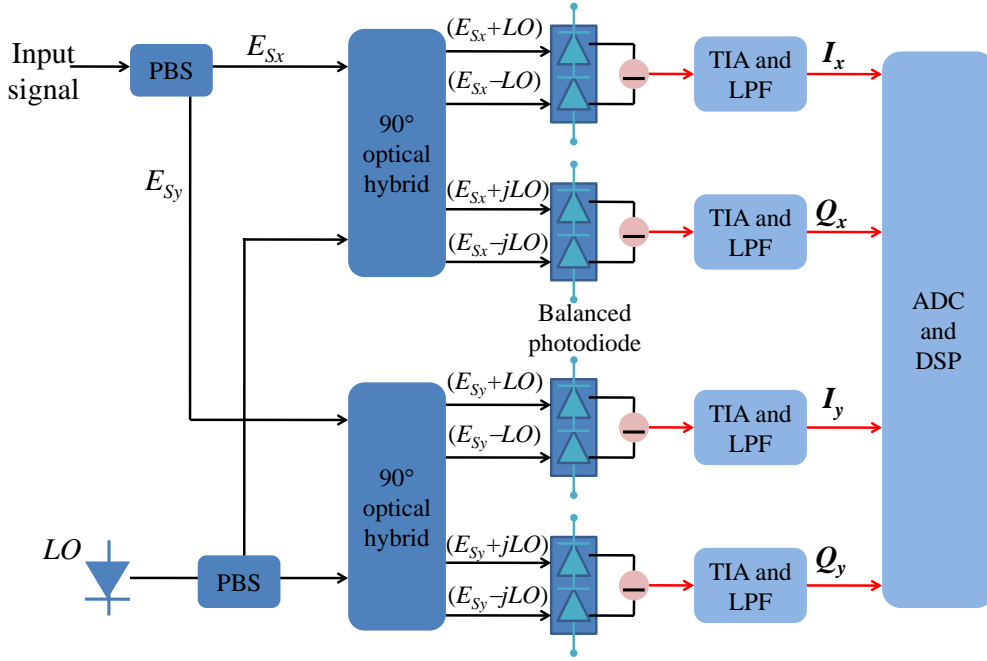
Figure I.10: General structure of dual-polarization, dual-quadrautres coherent receiver. S_{x(y)} corresponds to the x(y) -polarization. PBS: polarization beam splitter; TIA: trans-impedance amplifier; LPF: low-pass filter; ADC: analog-to-digital converter.
