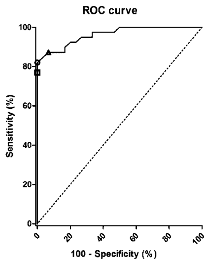
Fig. 1. Performance of GM detection according to the threshold. Receiver Operating Characteristics (ROC) curve for determination of cut-off and assay sensitivity (Se) and specificity (Sp). The thresholds 0.35, 0.4 and 0.5 are shown on the ROC curve with a triangle, circle and square, respectively.
