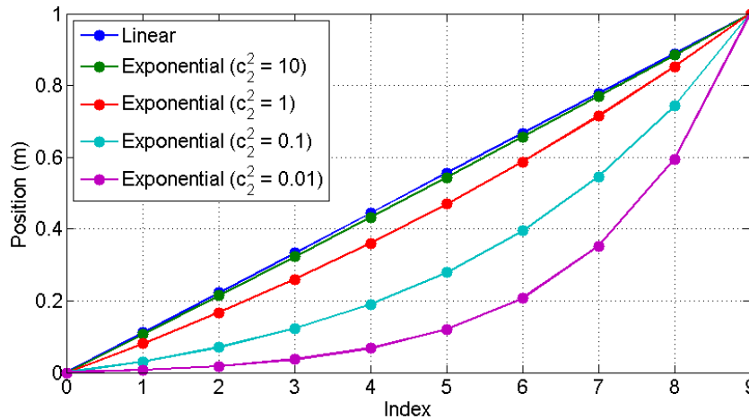
Figure 4.1: Point distribution options
