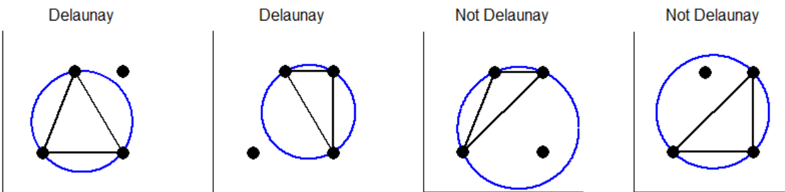
Figure 2.18: Delaunay triangulation
