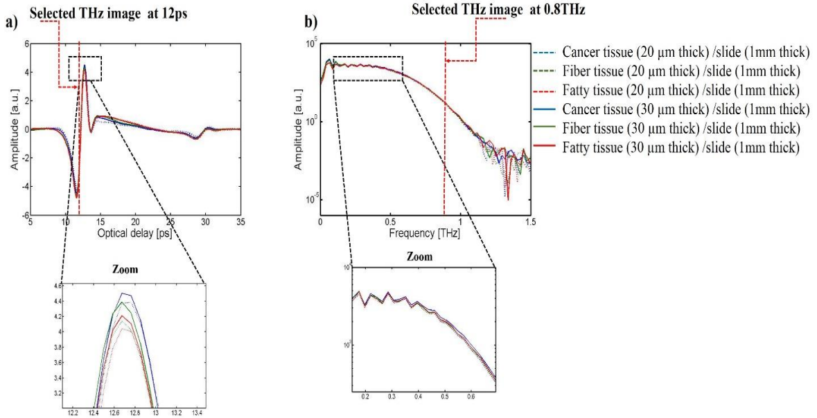
Figure 53: Transmission results on paraffin-embedded tissue (20 & 30 \mu\text{m} thick), mounted on microscope slides 1 mm thick, a) time-domain signals collected from cancer, fiber, and fatty tissues, and b) FFT spectra of these signals.
