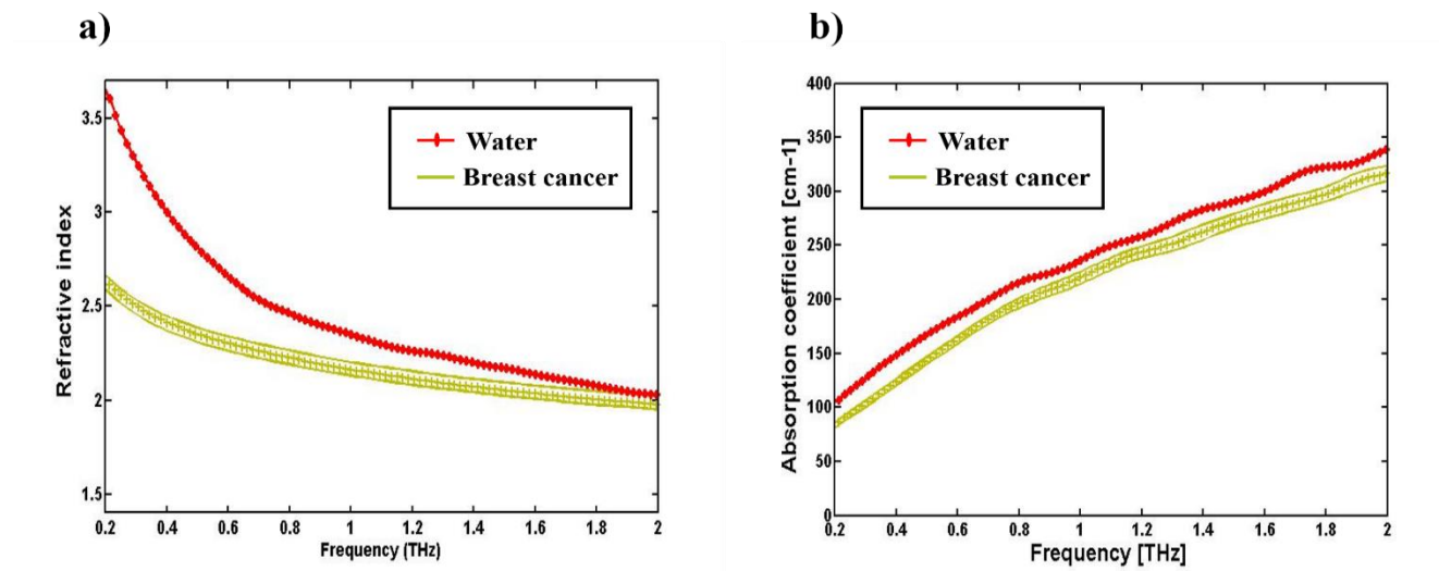
Figure 42: The a) refractive indices and b) absorption coefficients of inhomogeneous cancer tissue and water measured in THz reflection mode.
