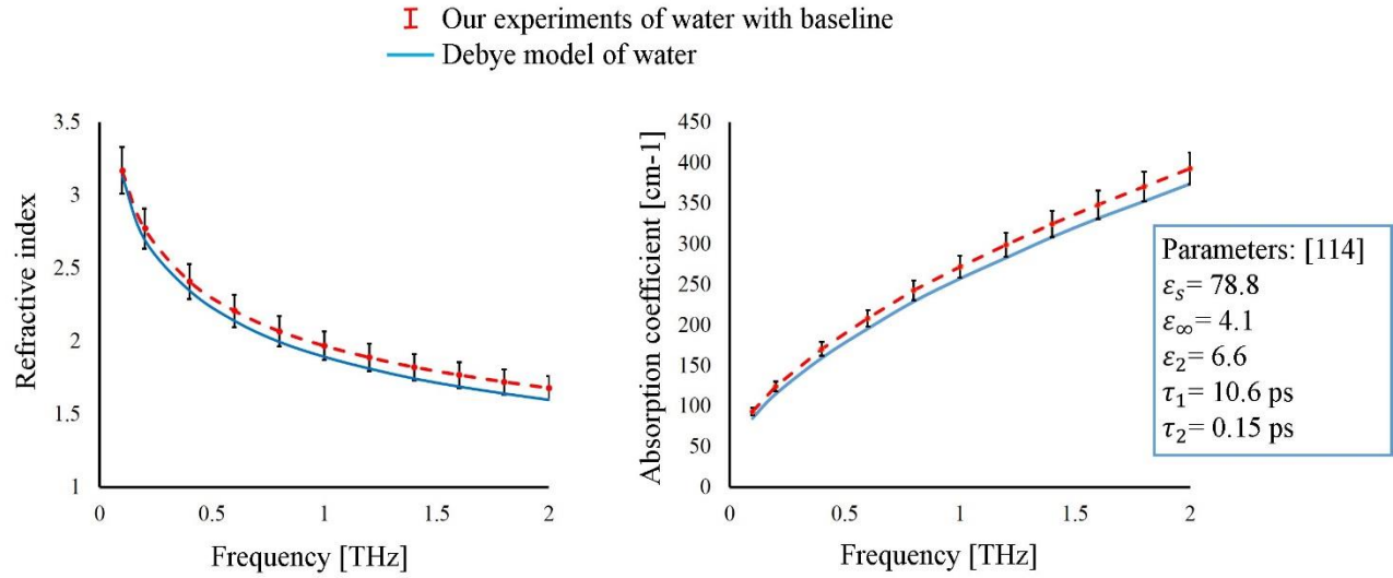
Figure 36: The refractive index (a) and absorption coefficient (b) of distilled water measured with TeraPulse 4000 in reflection mode, showing the error bars calculated from 10 measurements and 30 averaging in a hospital environment.
