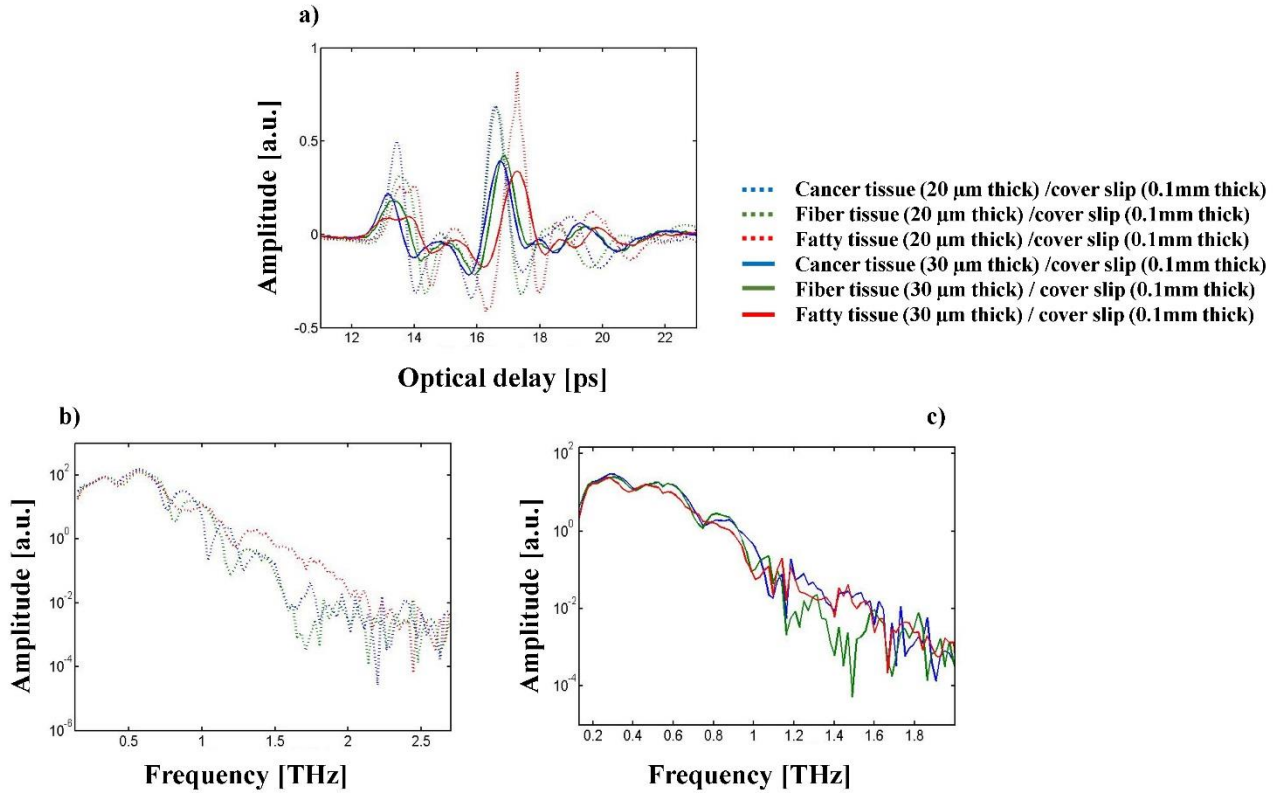
Figure 56: THz reflection results on paraffin-embedded tissue (20 & 30 \mu\text{m} thick), mounted on 0.1 mm-thick coverslips: a) time-domain signals collected from cancer, fiber, and fatty tissues; and b & c) FFT spectra of these signals.
