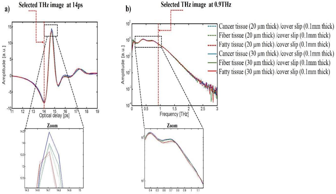
Figure 52: Transmission results on paraffin-embedded tissue (20 & 30 \mu\text{m} thick), mounted on coverslips 0.1 mm thick, a) time domain of signals collected from cancer, fiber, and fatty tissues, and b) FFT spectra of these signals.
