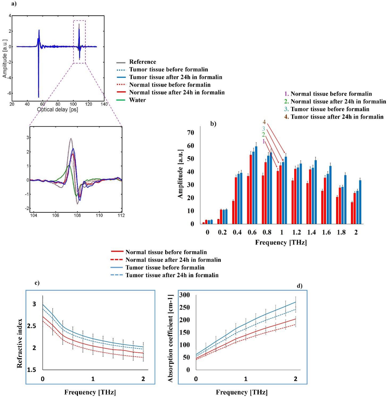
Figure 66: a) THz reflected in time domain; b) average spectrum amplitude with error bar for normal and tumor tissue as a function of frequency; and c & d) average with error bars for refractive index and absorption coefficient of tumor and normal tissue before and after formalin fixing.
