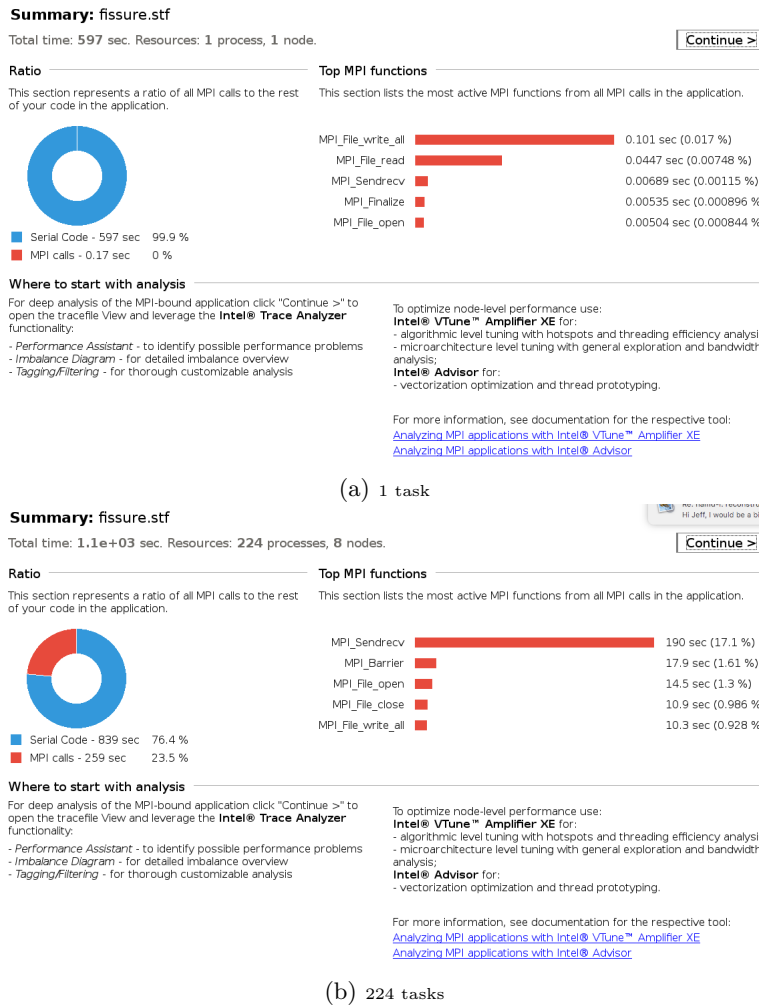
Figure 5.5: Computational statistics for the nonlocal algorithm.
