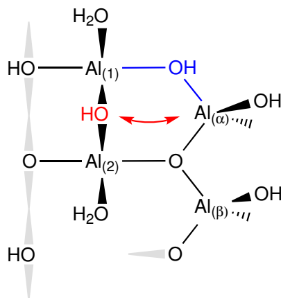
Figure 8.1: Skeletal representation of the s5 primitive cell surface of \gamma - \text{Al}_2\text{O}_3 (110). The bonds in blue are associated with the two CVs of metadynamics #1, namely \text{CN}(\text{Al}_{(1)}, \text{OH}_{(1\alpha)}) and \text{CN}(\text{Al}_{(\alpha)}, \text{OH}_{(1\alpha)}) . The red double arrow stands for \text{CN}(\text{Al}_{(\alpha)}, \text{OH}_{(12)}) used in metadynamics #2 along with \text{CN}(\text{Al}_{(\alpha)}, \text{O}) .
