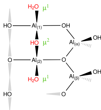
Figure 9.1: Skeletal representation of surface \gamma -Al 2 O 3 . In this work we considered the exchange of the functional groups represented in red (namely \mu^1 water molecules and the bridging \mu^2 hydroxyle group).
