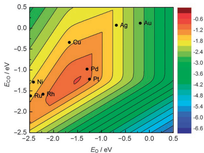
Figure 3: 2D volcano plot obtained from first principles calculations for the reaction \text{CO} + \frac{1}{2} \text{O}_2 \rightarrow \text{CO}_2 . It represents the activity (the color scale gives the effective activation energy in eV) of catalysts as a function of oxygen and carbon monoxide binding energies to the surface. From Falsig et al. , 5 Copyright ©2000 by John Wiley Sons, Inc. Reprinted by permission of John Wiley & Sons, Inc.
