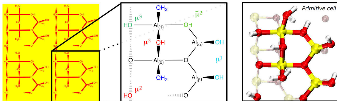
Figure 7.2: Skeletal representation of the \gamma -Al 2 O 3 (110) primitive surface model used in this work. The unit cell consists of four of those. Aluminum atoms are not represented for simplicity but are found at each intersect between at least two bonds.
