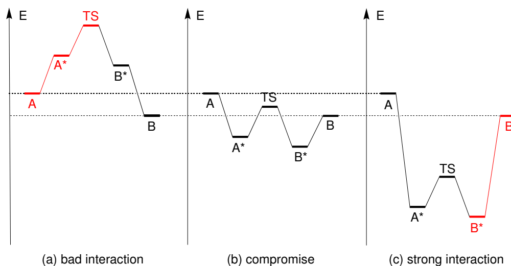
Figure 1: Energy profiles of the reaction A \rightarrow B . A^* , B^* and TS stand for the adsorbed states of A and B and the transition state for the elementary step A^* \rightarrow B^* . The barrier of the latter is considered constant, representing the influence of the interaction of A and B with the surface catalyst.
