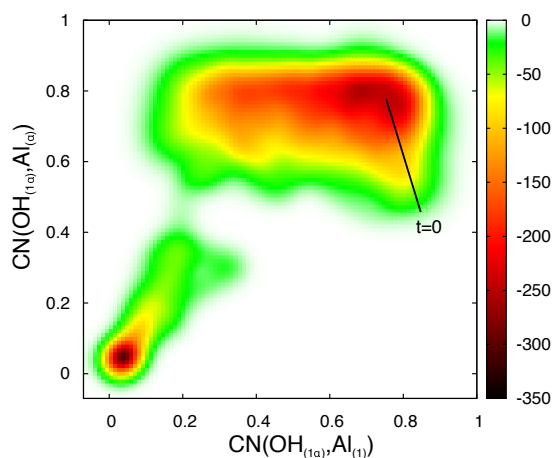
Figure 8.2: Reconstructed Free Energy profile in the dimensions of the two CVs used for metadynamics #1. The color scale is given in kJ/mol.
