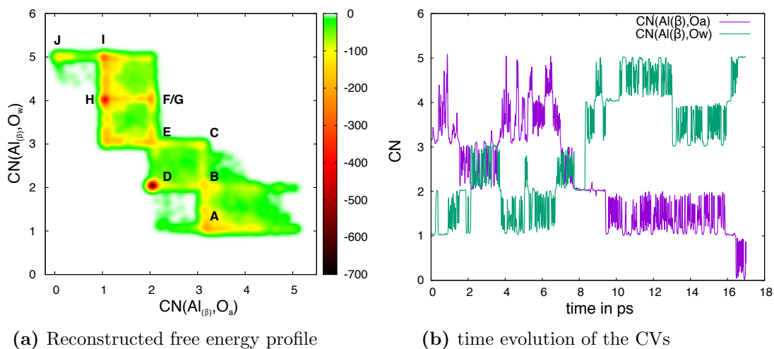
Figure 8.7: Free energy profile and time evolution of the CVs for metadynamics #5.
