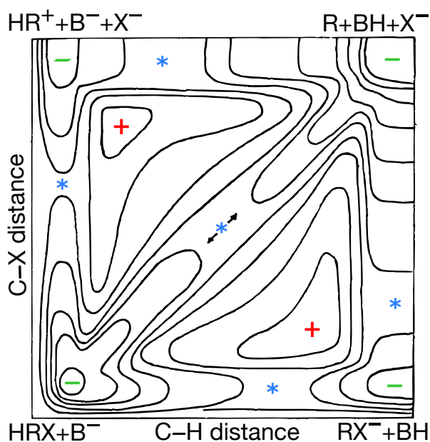
Figure 1.1: More O'Ferrall Jencks diagram of the \beta -elimination \text{HRX} + \text{B}^- \rightarrow \text{R} + \text{BH} + \text{X}^- . R, X and B represent a \text{CH}_2\text{CH}_2 unit, a leaving group, and a base respectively. It gives an isovalue free energy diagram plotted versus the C–H and C–X distance. Pluses, minuses and asterisks indicate maxima, minima and 1st order saddle points respectively. Adapted from More O'Ferrall 1 with permission of the Royal Chemical Society.
