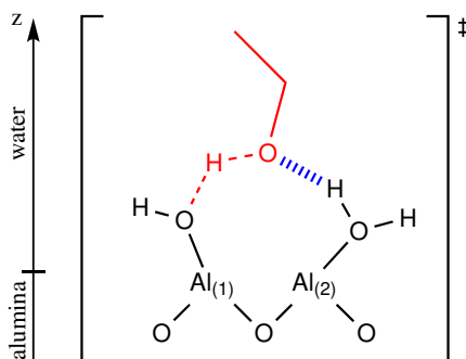
Figure 9.4: Transition state associated with the desorption of EtO - from state B to state C . The proton of a neighboring chemisorbed water molecule is transferred to the EtO - group, implying a displacement of the resulting hydroxyle group in a bridging position between Al (1) and Al (2) .
