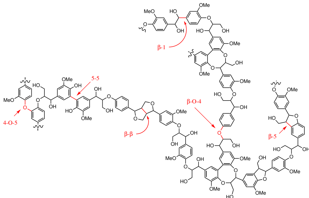
Figure 2.1: Representative structure of lignin with its characteristic linkages highlighted in red. 1
