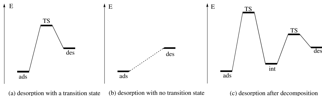
Figure 1.2: Three different energy profiles of desorption. ads , int , des and TS stand for adsorbed reactant, adsorbed intermediate, transition state and desorbed product respectively. The vertical axis reports variations of the potential energy.
