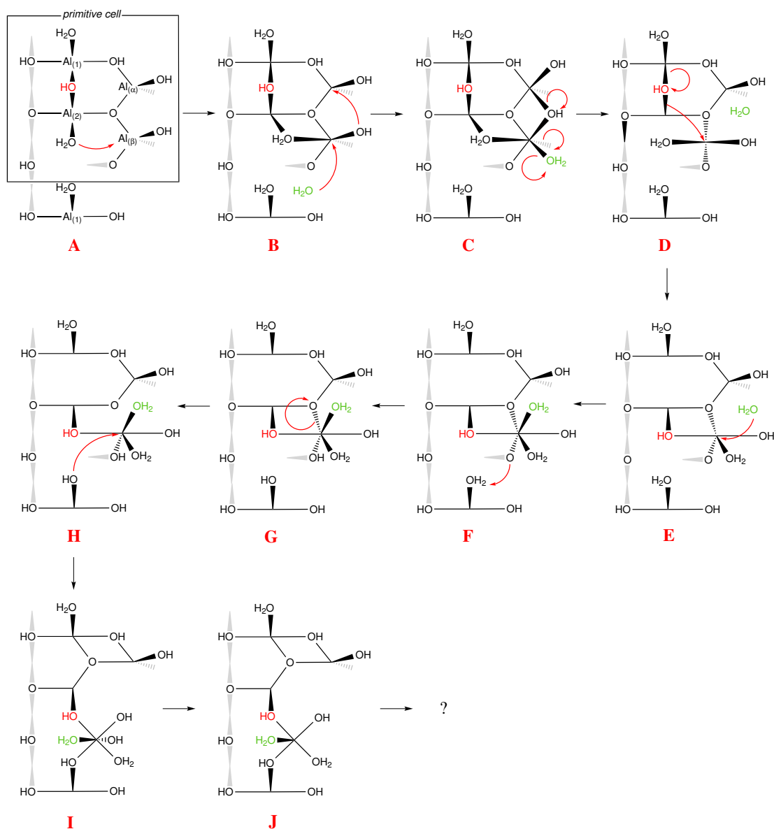
Figure 8.8: Schematic mechanism associated with metadynamics #5 using the skeletal representation for the alumina surface. For simplicity, aluminum atoms are explicitly represented only for structure A. Green \text{H}_2\text{O} does not represent any specific water molecule.
