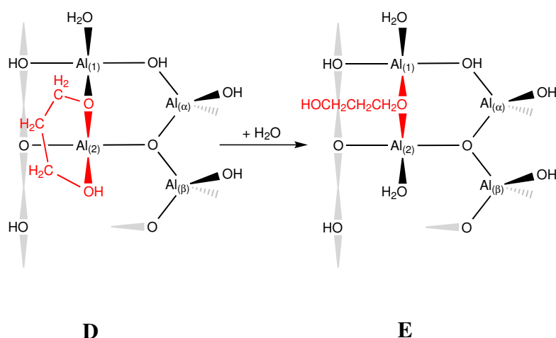
Figure 9.5: Partial desorption of bidentate 1,3-PDO on \gamma - \text{Al}_2\text{O}_3 (including exchange with water) from state D to state E .
