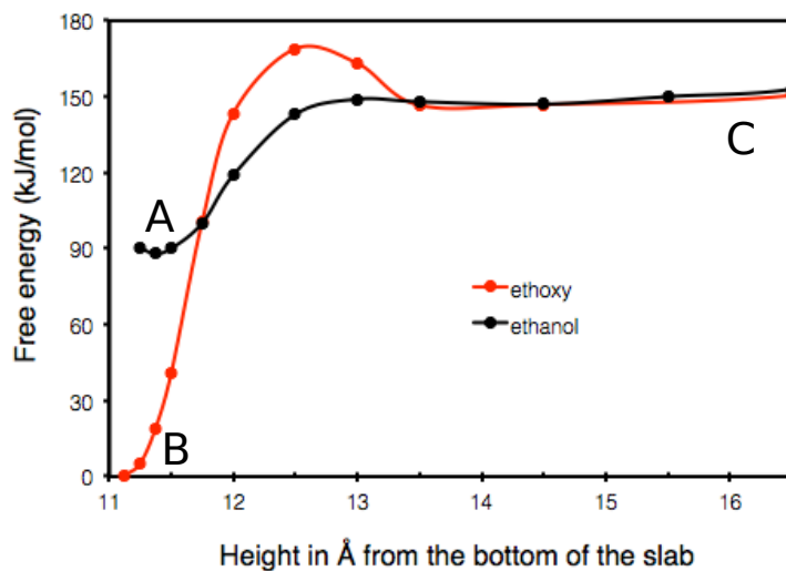
Figure 9.3: Free-energy profiles of EtOH/EtO - desorption (including water exchange) associated with the states A , B and C as given in Figure 9.2.
