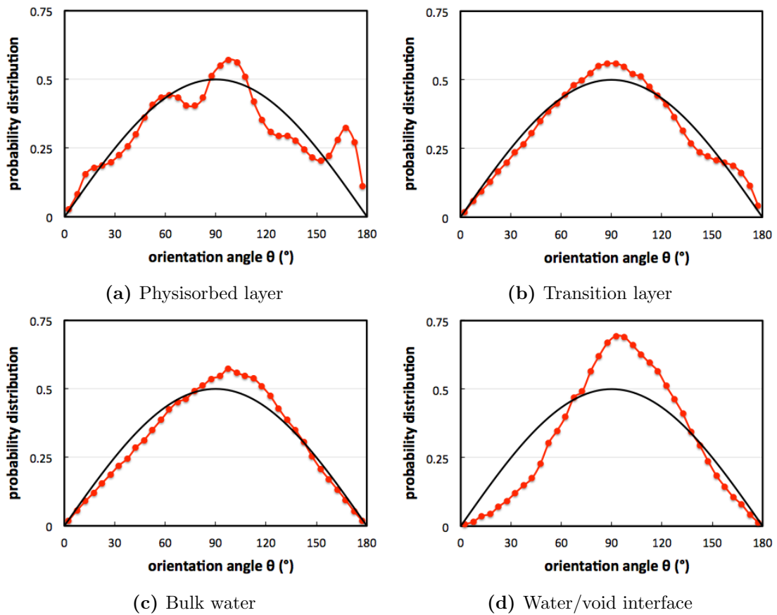
Figure 7.6: Dipole orientation distributions in (a) the physisorbed layer, (b) the transition layer, (c) bulk water, and (d) the interface with void. The black plain curve is the uniform distribution \frac{1}{2} \sin \theta and the red dotted curves are the distributions obtained from the simulation.
