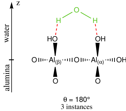
Figure 7.7: Favored orientation of water at the interface with \gamma -Al 2 O 3 .
