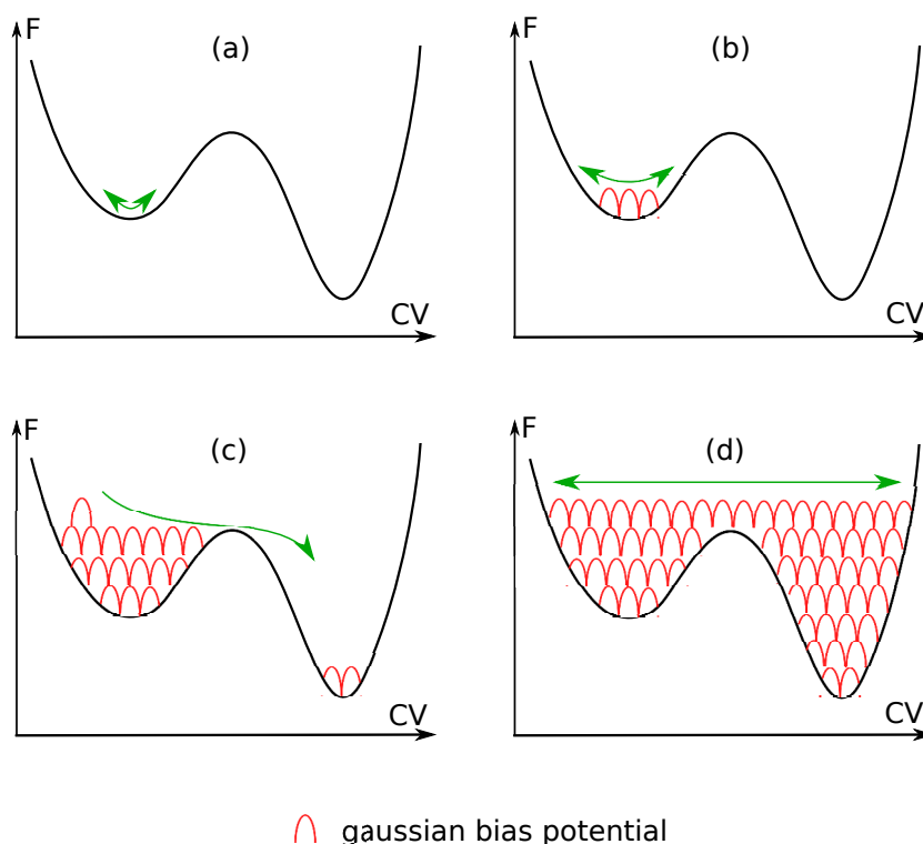
Figure 1.3: Representation of the principle of metadynamics at four different instants of the dynamics. Here we consider a one-dimension sampling along one CV. During the simulation, repulsive gaussians are added to have the the system visit a larger and larger phase-space. The green arrow represents the amplitude of phase-space sampling.
