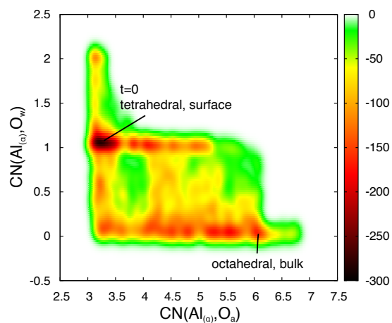
Figure 8.6: Reconstructed Free Energy profile in the dimensions of the two CVs used for metadynamics #4. The color scale is given in kJ/mol.
