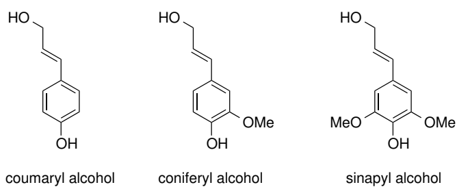
Figure 2.2: Alcohol monomers of lignin.
