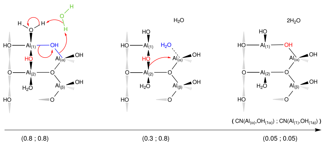
Figure 8.3: Skeletal representation of the hydrolysis of the \text{Al}_{(1)}\text{-OH}_{(1\alpha)}\text{-Al}_{(\alpha)} bond along the reaction coordinate described by \text{CN}(\text{Al}_{(\alpha)}, \text{OH}_{(1\alpha)}) and \text{CN}(\text{Al}_{(1)}, \text{OH}_{(1\alpha)}) . The initially bridging OH group is colored in red to facilitate its tracking along the process. The extra physisorbed water molecule involved in the proton transfer is colored in green.
