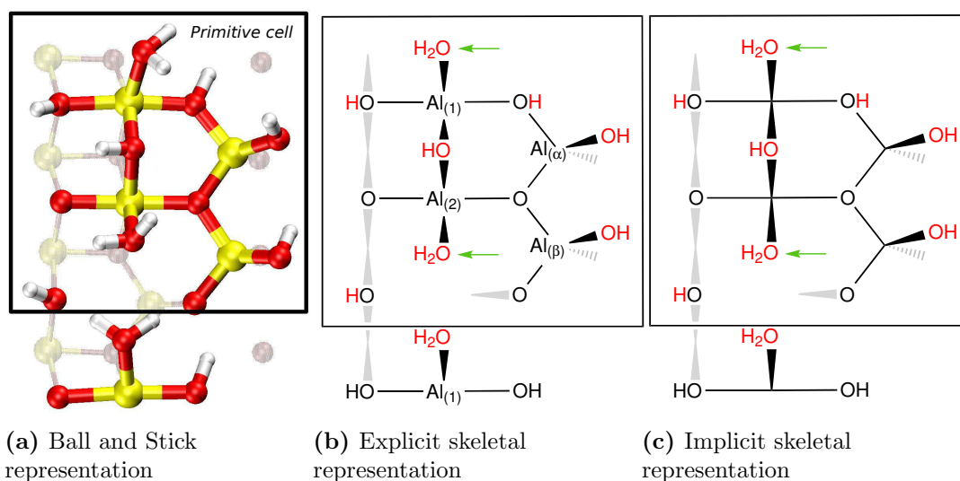
Figure 6.3: Three different representations of the initial (110) surface s5 used in the present work. (a) Ball and stick representation with yellow balls for Al, red balls for O and white balls for H, (b) explicit skeletal representation with the labelling of the Al atoms used in the present work, (c) implicit skeletal representation (the Al atoms are not represented but are found at the intersection of at least two bounds). In (b) and (c), green arrows point out the two extra water molecules added on surface s3a (see Figure 6.2), red atoms come from the chemisorption of water on pristine \gamma -Al 2 O 3 and are therefore not considered to belong to \gamma -Al 2 O 3 . In (a), (b) and (c) the square represents the limits of the surface primitive cell.
