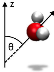
Figure 7.5: Definition of the dipole orientation angle \theta . The z -axis is the normal to the \gamma -Al 2 O 3 surface.
