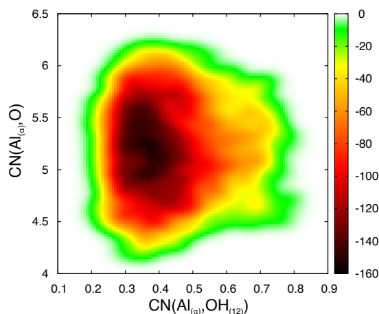
Figure 8.4: Reconstructed Free Energy profile in the dimensions of the two CVs used for metadynamics #2. The color scale is given in kJ/mol.
