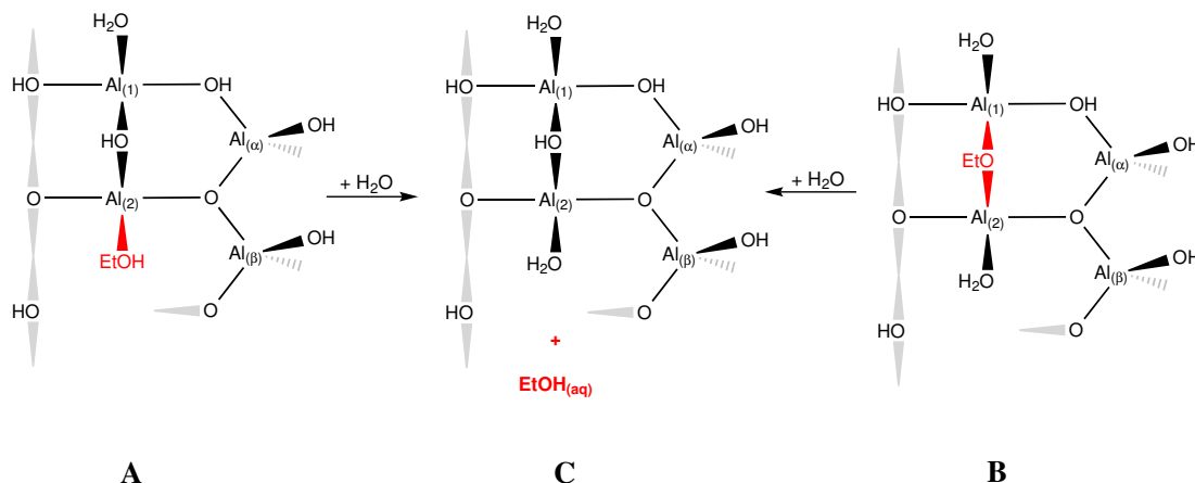
Figure 9.2: Ethanol desorption from states A and B to state C . This desorption process is actually an exchange of EtOH/EtO - with water molecular since the simulation is performed in liquid water.
