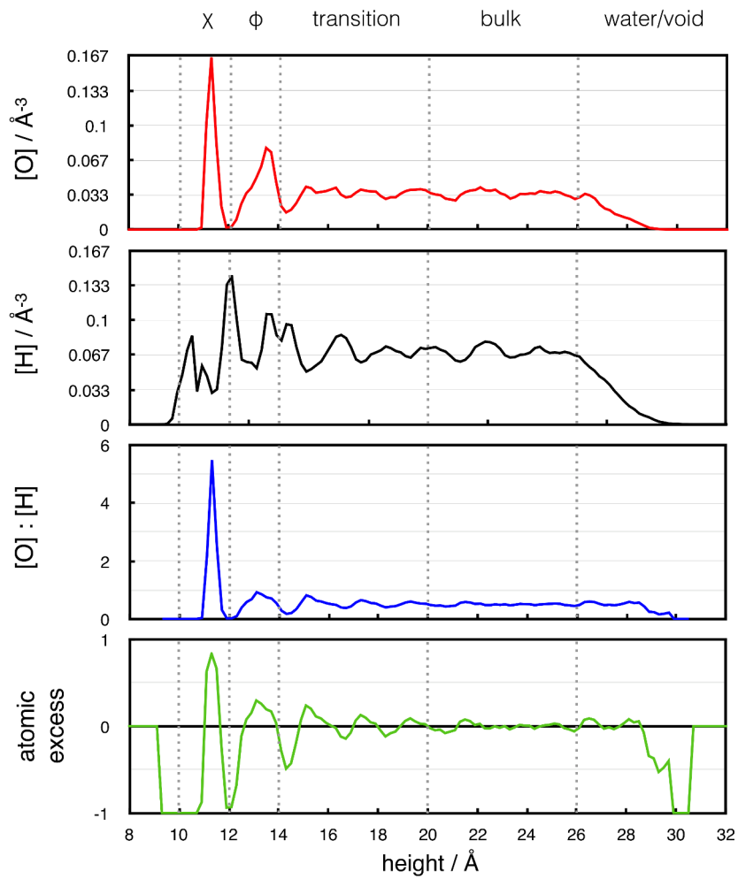
Figure 7.3: Concentration based characteristics of water as a function of height (the scale starts from the bottom of the alumina slab).
