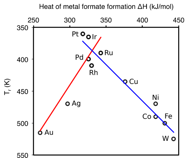
Figure 2: Volcano-plot for formic acid decomposition as a function of the heat of formation \Delta H of formate. T_r is the temperature at which a rate of 6.3 \text{ s}^{-1} is reached for a given catalyst. Replotted from data published by Rootsart and Sachtler. 3
