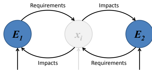
Figure 0.8: Coupling between two biogeochemical cycles through a shared biotic compartment. In this context, requirements and impacts of the biotic compartment correspond to incoming and outgoing fluxes of matter.
