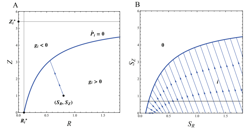
Figure 2.3: A: Illustrative ZNGI (blue, thick), impact vector (blue, thin) and supply point (black dot) for a plant species i . The ZNGI resembles the uptake function g_i(R) of Fig. 2.2, except that it starts on the x-axis at R_i^* and saturates at Z_i^* (gray lines). The impact vector maps this particular supply point to the corresponding equilibrium point on the ZNGI. B: Bifurcation diagram representing the ecological outcome of this plant species i growing on the resource R and being preyed upon by Z , as a function of the external supply (S_R, S_Z) . The conditions are too harsh in zone 0 for the plant to survive (above ZNGI _i ) whereas they are good enough to enable plant growth in zone i . Note that the plant can never grow when S_R < R_i^* or when S_Z > Z_i^* . The impact rays (blue, dashed) map the supply points onto their corresponding limiting factor values (R, Z) at equilibrium, on ZNGI _i . In this example, \alpha_i = 1 , \mu_i = 0.25 and a_i = 0.033 , the other parameters being from Table 2.1.
