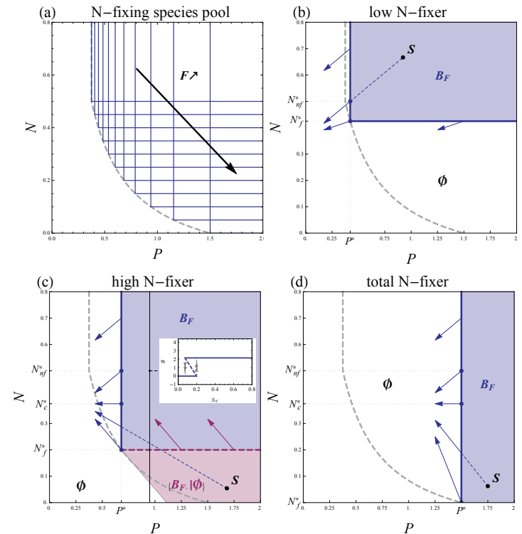
Figure 3.2: (a) ZNGIs (blue, L-shaped) representing the competitive abilities of N-fixers from the species pool with normalized fixation abilities F/m comprised between 0 and 1. The ZNGI corners all line up on a decreasing envelope (dashed grey), which materializes the trade-off between P^* and N_{nf}^* . (b), (c) and (d): Ecological phase diagrams along N and P availabilities for three different N-fixing strategies: low, high and total N-fixer corresponding respectively to F/m = 0.15, 0.6 and 1 . The ZNGI (thick, L-shaped), a strategy’s minimal nutrient requirements for growth, also gives the possible nutrient levels at equilibrium, which can be either stable (blue, plain) or unstable (purple, dashed). The impact vectors (blue and purple vectors) correspond to a strategy’s per capita impact on the two nutrients. They point down when this impact is negative, up when it is positive. The blue-shaded region (labeled B_F ) gives the external nutrient supplies S = (S_P, S_N) (e.g. black dot) under which the N-fixer can subsist, leading to a vegetated ecosystem. In the white region (labeled \emptyset ), supplies are too low and the N-fixer goes extinct, leading to the bare substrate. The purple-shaded region (labeled B_F|\emptyset ) has the vegetated ecosystem and the bare substrate as two alternate stable states. This can be seen in the inset in (c), where the biomasses at equilibrium (blue) of these two stable states (plain) and the unstable state that separates them (dashed) have been plotted against a nutrient gradient with increasing S_N and fixed S_P (black, vertical line). High N-fixer biomass is constant along this N gradient because only P is limiting.
