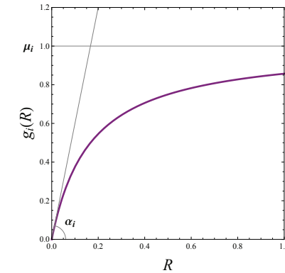
Figure 2.2: Type-II functional response, or Michaelis-Menten kinetics, used to model plant i resource uptake g_i as a function of available resource concentration R . When resource is limiting ( R \ll \mu_i/\alpha_i ), plant uptake is directly proportional to R via the affinity \alpha_i . When resource is not limiting ( R \gg \mu_i/\alpha_i ), plant uptake is no longer controlled by resource availability R and saturates to the plant maximal growth rate \mu_i . In this example, \alpha_i = 6 and \mu_i = 1 .
