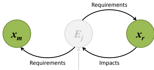
Figure 0.6: Resident-mutant interaction mediated by the environment. The mutant density is at first to low to have any impact on the environment.
