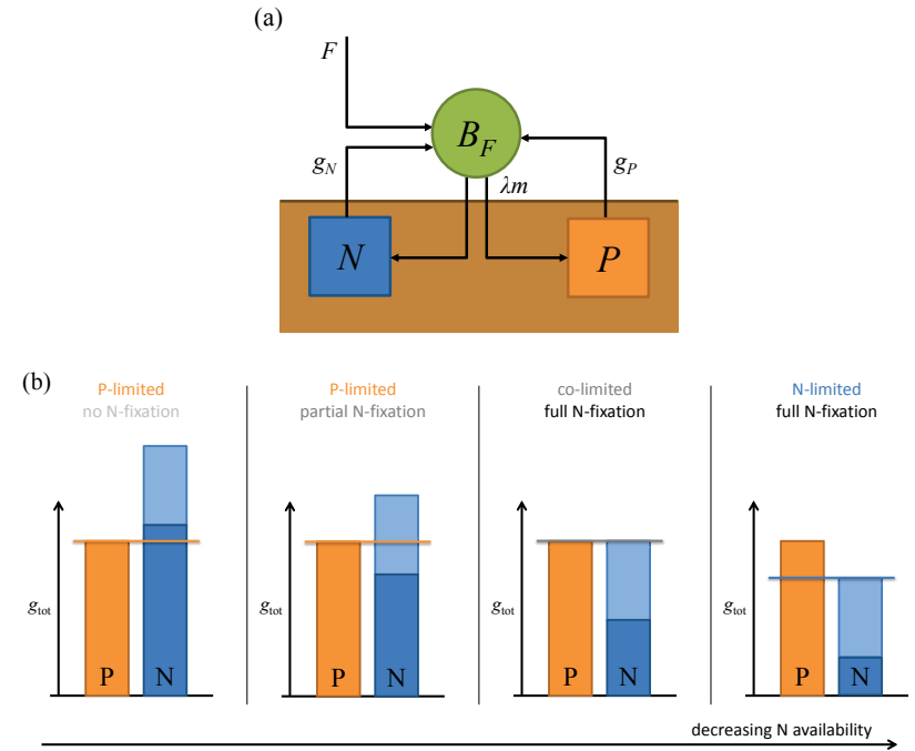
Figure 3.1: (a) Flow diagram of the model. (b) Schematic representation of how soil P availability (orange), soil N availability (dark blue) and N-fixing ability (light blue) combine in Liebig's law to determine plant growth g_{tot} and uptake rates (black arrow) along a N availability gradient. When soil P is more limiting than soil N, plants are P-limited and fixation is unnecessary (far left). When soil N is more limiting than soil P, there are three possibilities. Either maximal fixation rate is large enough for N not to be limiting, leading to P-limitation with partial N-fixation (center left), or fixation is just right to reach colimitation (center right), or fixation is insufficient to overcome N limitation, leading to N-limitation with full N-fixation (far right).
