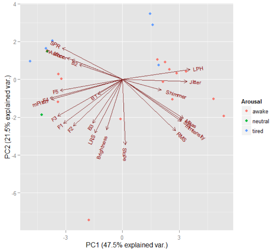
Figure 2.10: PC1 and PC2 of all the vocal features clustered by Arousal
