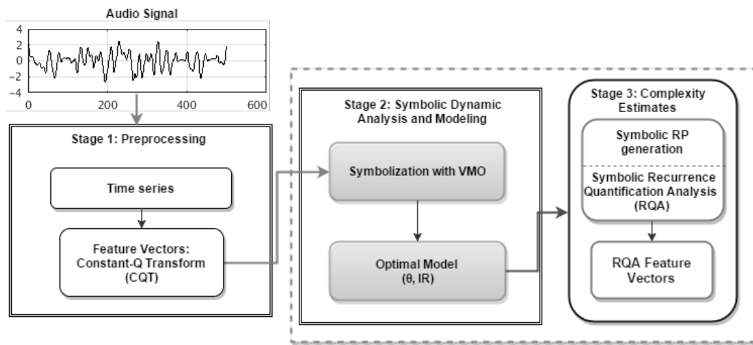
Figure 5.1: Nonlinear Symbolic Dynamical Framework
