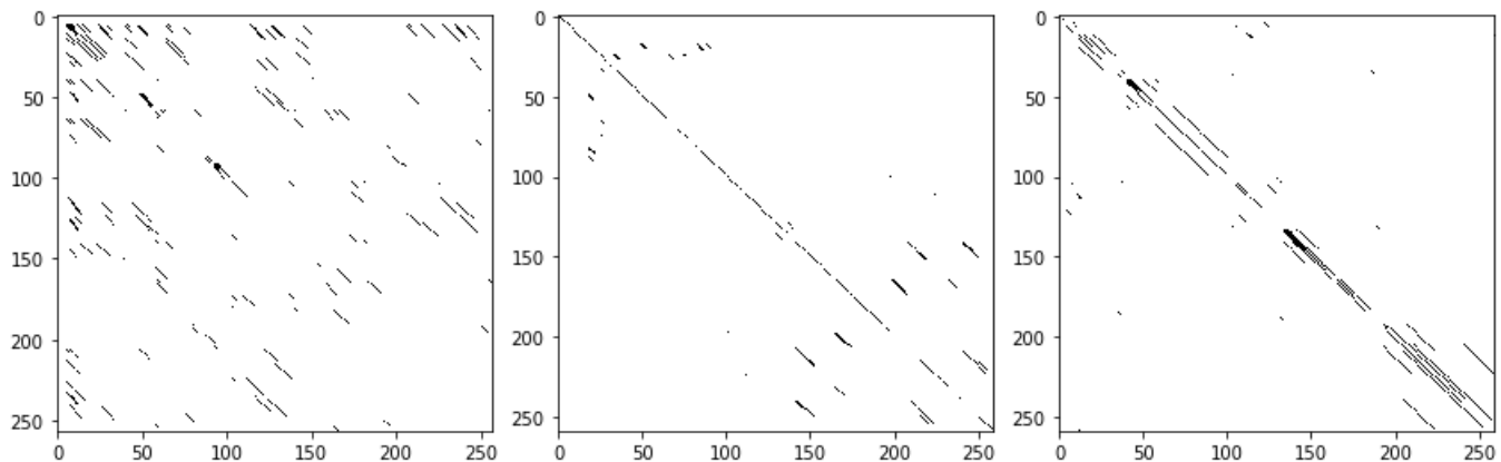
Figure 5.4: RP_s for pleasant scenes: countrynight ( left ), carousel ( middle ), tropical ( right )
