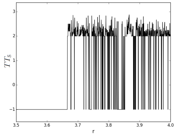
Figure 5.3: RQA s of the logistic map: r \in [3.5, 4.0] , \Delta r = 0.0005 and T = 1000
