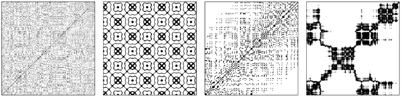
Figure 4.1: Characteristic Structures of recurrence plots: (A) Homogeneous, (B) Periodic, (C) Drift, (D) Disrupted [134]
