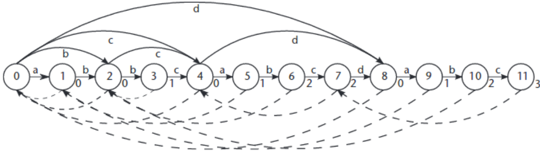
Figure 4.2: Factor Oracle for string \mathcal{S} = \text{"abbcabcbcdabc"} . A symbol is attributed to each forward link [222]
