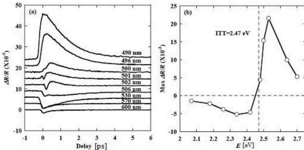
Figure 3.8: (a) Transient reflectivity of gold excited by 800nm pump-photons at 5.28 mJ/cm 2 fluence and probed by varying wavelengths, with curves shifted vertically for clarity. (b) Dependence of the amplitude of the transient reflectivity on the probe photon energy (the vertical dashed line marks the energy for ITT) [GX14].
