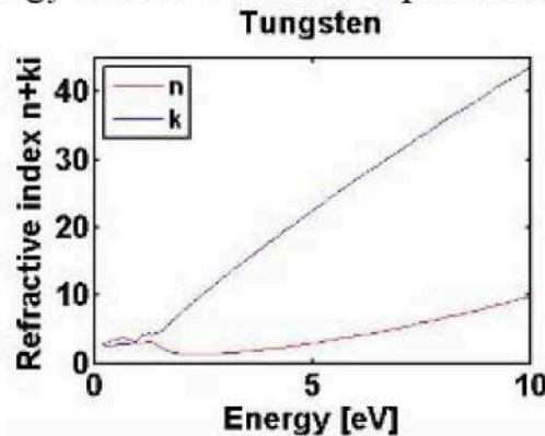
Figure 4.7: The frequency-dependent refractive index of tungsten [Ham04].
