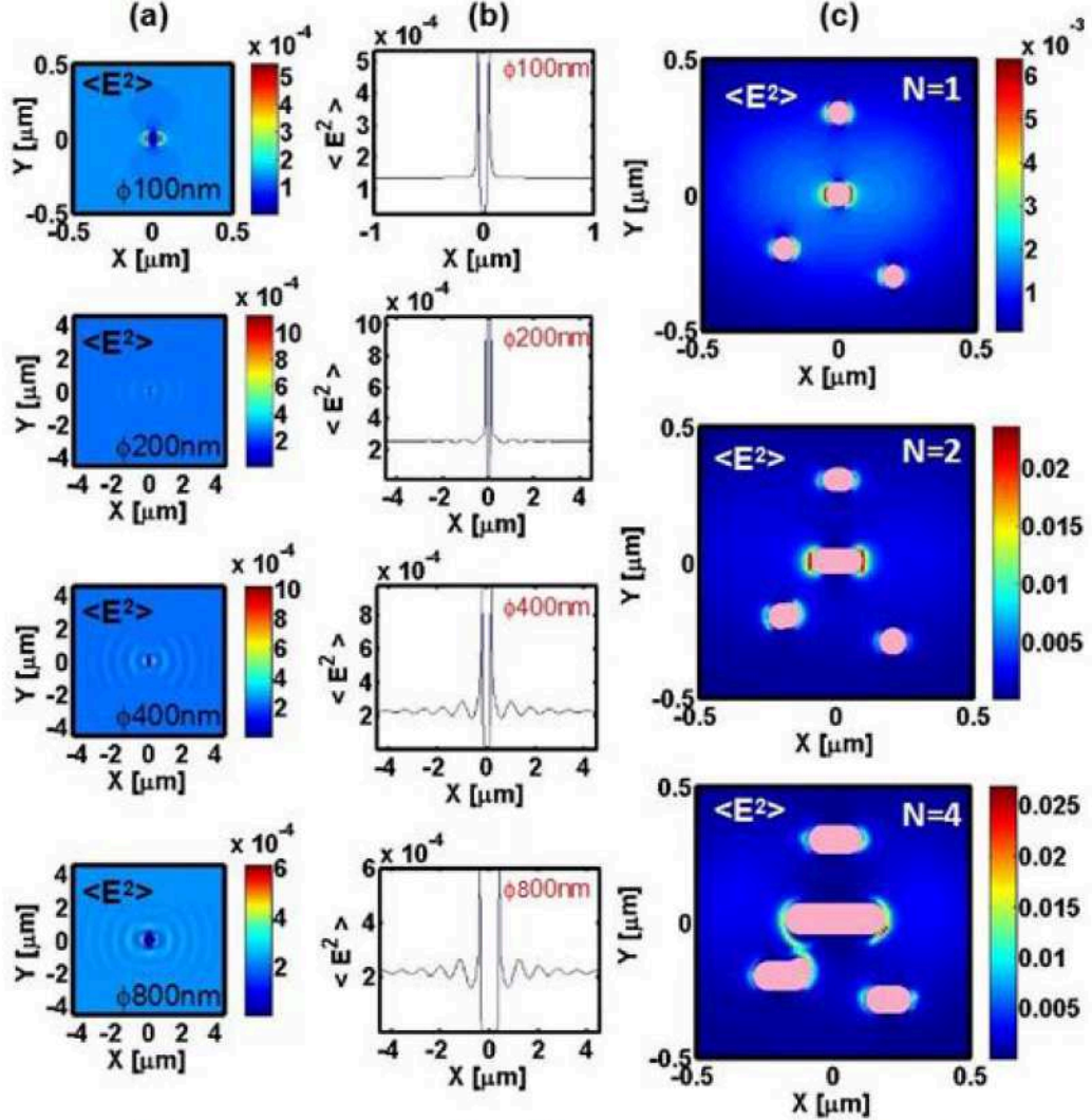
Figure 6.27: (a) Time-averaged E^2 distribution on the surface XOY plane induced by a hemisphere of different diameters: \phi=100 nm, \phi=200 nm, \phi=400 nm, \phi=800 nm; (b) Time-integrated E^2 distribution along Y=0 axis induced by a hemisphere with different sections: \phi=100 nm, \phi=200 nm, \phi=400 nm, \phi=800 nm; (c) Time-averaged E^2 distribution on XOY plane induced by four hemispheres of \phi=100 nm with the number of pulses. Top: a first incident pulse, middle: elongated structures interact with a second pulse, bottom; more elongated ripple in interaction with a fourth pulse. The ripple domains are indicated by the pink color. The polarization direction of the incident planewave is along X axis.
