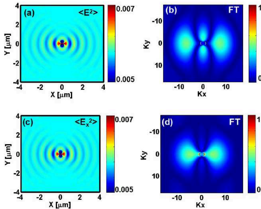
Figure 6.12: (a) Total energy distribution pattern on surface derived from stationary fields (time-averaged E^2 ) with (b) its Fourier decomposition. (c) Energy distribution of interferential terms pattern (time-averaged E_x^2 ) on surface with (d) its Fourier (FT) decomposition. Note that laser polarization is along X axis. Identical color bars are used for (b) and (d).
