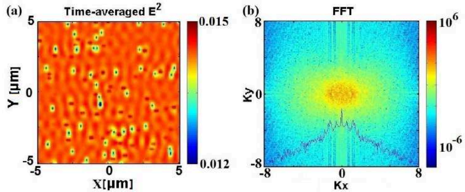
Figure 6.15: (a) Time-averaged E^2 distribution just above the rough surface for an ensemble of scatterers. (b) 2D-FFT of the intensity distribution in (a), the values along K_y=0 is shown at the bottom of Fig. 6.15(b). A logarithmic color bar is used to emphasize the details.
