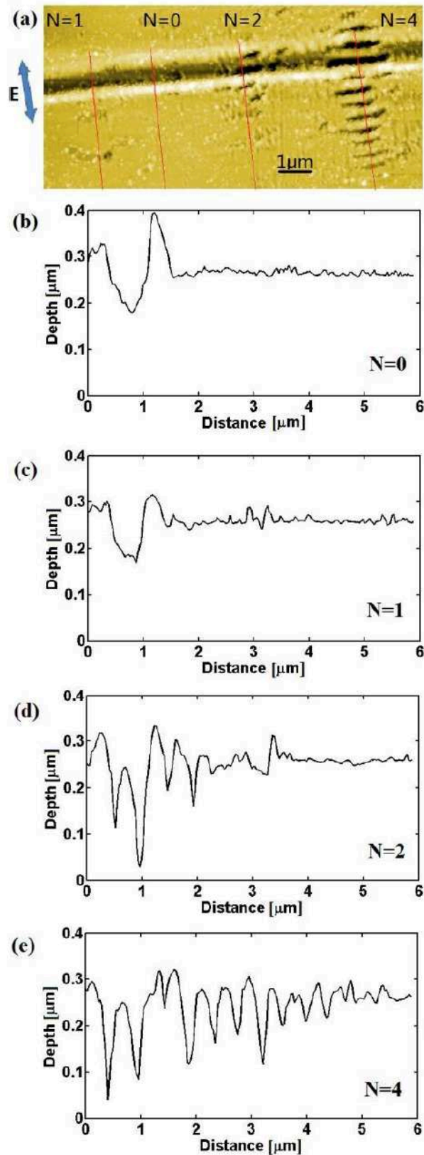
Figure 6.16: (a) AFM image of the groove shot by N=1 , 2, and 4 pulses. The laser polarization is indicated by the double-arrow in (a) and the laser fluence is 1.15\text{ J/cm}^2 ; (b-e) cross-section profiles of groove: (b) not irradiated; (c) after N=1 pulse; (d) after N=2 pulses; (e) after N=4 pulses.
