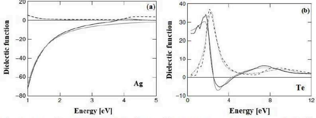
Figure 3.1: (a) Drude model of Ag. (b) Lorentz model of Te. Black lines represent literature values of \text{Re}[\varepsilon] (solid) and \text{Im}[\varepsilon] (dashed) [Pal85], while gray lines represent the best-fit values of \text{Re}[\varepsilon_{\text{model}}] (solid) and \text{Im}[\varepsilon_{\text{model}}] (dash-dotted).
