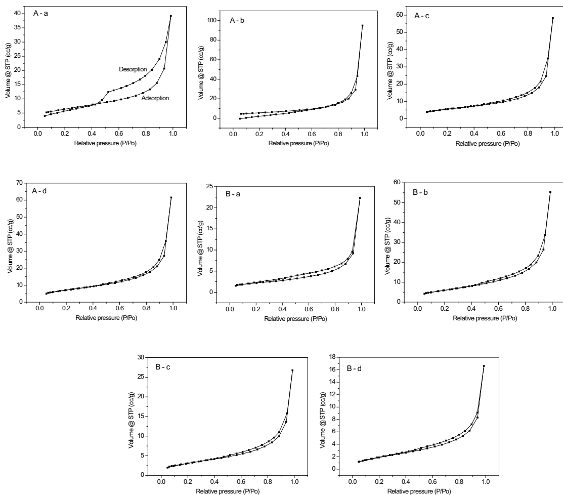
Figure 7 - Adsorption and desorption nitrogen isotherms of raw montmorillonite (Aa) and samples after milling for 3 h (Ab); 6 h (Ac); 9 h (Ad); raw talc (Ba) and samples after milling for 6 h (Bb); 9 h (Bc); 12 h (Bd).
