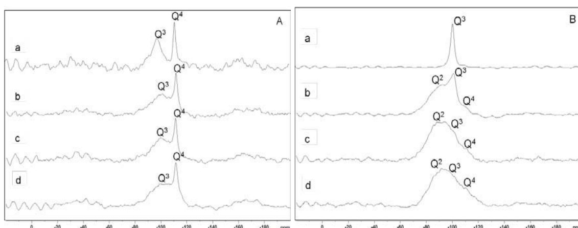
Figure 7 – ^{29}Si MAS NMR spectra of raw montmorillonite (Aa) and samples after milling for 3 h (Ab); 6 h (Ac); 9 h (Ad); raw talc (Ba) and samples after milling for 6 h (Bb); 9 h (Bc); 12 h (Bd).
