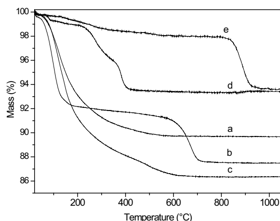
Figure 4 - TGA curves of the milled MMT/ \text{K}_2\text{HPO}_4 (a), raw MMT (b), milled talc/ \text{K}_2\text{HPO}_4 (c), \text{K}_2\text{HPO}_4 (d) and raw talc (e). MR = 1:2 and milling times of 9 h and 12 h for MMT and talc, respectively.
