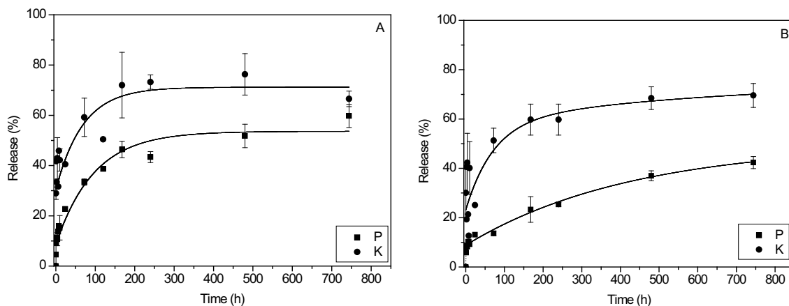
Figure 6 – Release assays of MMT/ K_2HPO_4 system (A) and talc/ K_2HPO_4 system (B). MR = 1:2 and milling times of 9 h and 12 h for MMT and talc, respectively.
