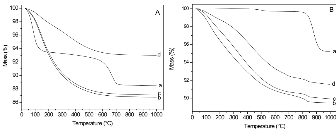
Figure 5 – TGA curves of raw montmorillonite (Aa) and samples after milling for 3 h (Ab); 6 h (Ac); 9 h (Ad); raw talc (Ba) and samples after milling for 6 h (Bb); 9 h (Bc); 12 h (Bd).
