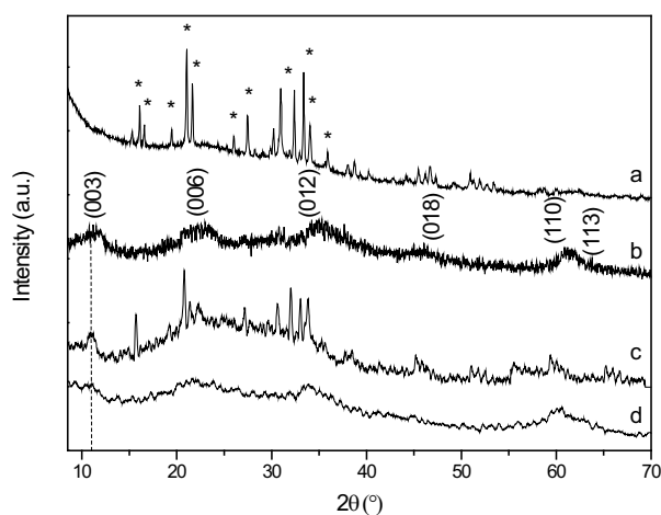
Figure 13 – XRD data for solid residues for: \text{MgAl}_{200}/\text{K}_2\text{HPO}_4 after 1 h (a) and 168 h (b) and \text{MgFe}_{200}/\text{K}_2\text{HPO}_4 after 30 minutes (c) and 168 h (d)
