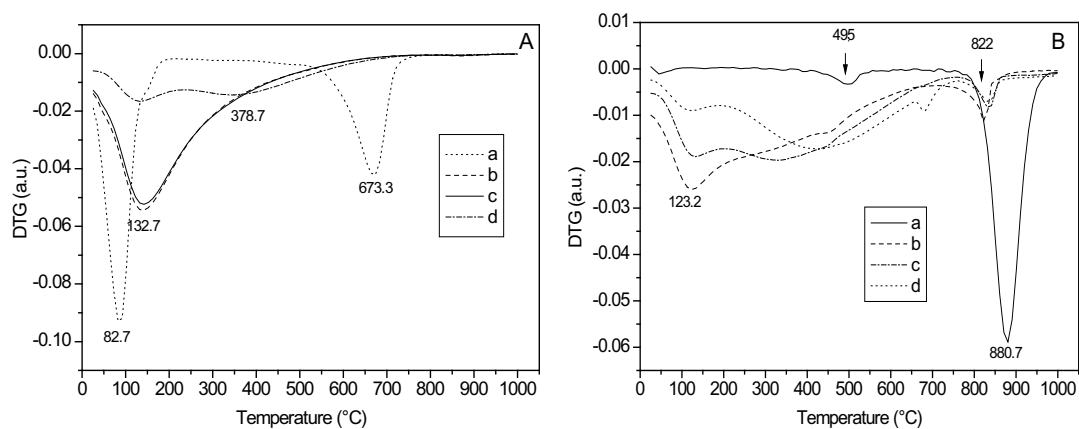
Figure 6 - DTG curves of raw montmorillonite (Aa) and samples after milling for 3 h (Ab); 6 h (Ac); 9 h (Ad); raw talc (Ba) and samples after milling for 6 h (Bb); 9 h (Bc); 12 h (Bd).
