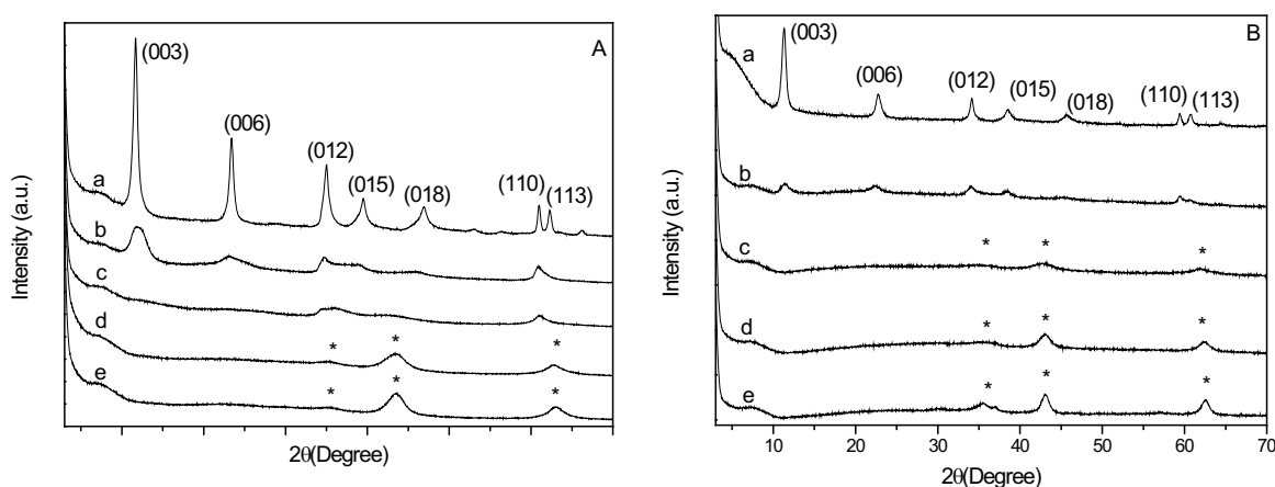
Figure 1– PXRD data of Mg 2 Al(OH) 6 (CO 3 ).3H 2 O (Aa); Mg 2 Fe(OH) 6 (CO 3 ).2.5H 2 O (Ba) and LDH calcined at: 200°C (Ab; Bb); 300°C (Ac; Bc); 400°C (Ad; Bd); 500°C (Ae; Be) respectively.
