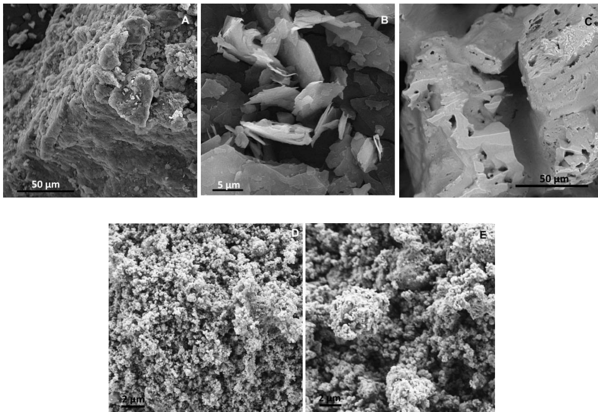
Figure 5 - SEM images of MMT (A), talc (B), K_2HPO_4 (C), milled MMT/ K_2HPO_4 (D) and milled talc/ K_2HPO_4 (E). MR = 1:2 and milling times of 9 h and 12 h for MMT and talc, respectively.
