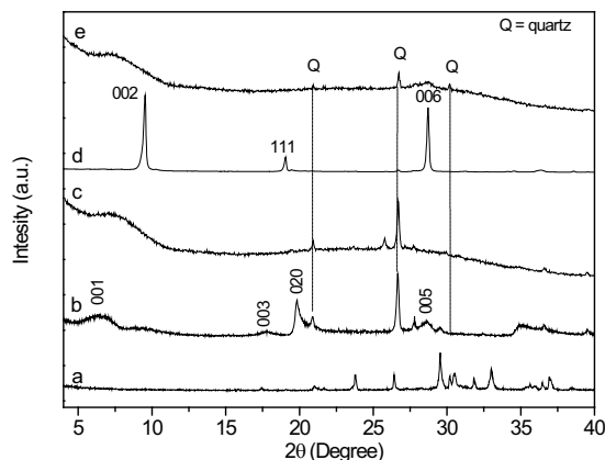
Figure 1 - XRD patterns of K_2HPO_4 (a), MMT (b), milled MMT/ K_2HPO_4 (c), talc (d) and milled talc/ K_2HPO_4 (e). MR = 1:2 and milling times of 9 h and 12 h for MMT and talc, respectively.
