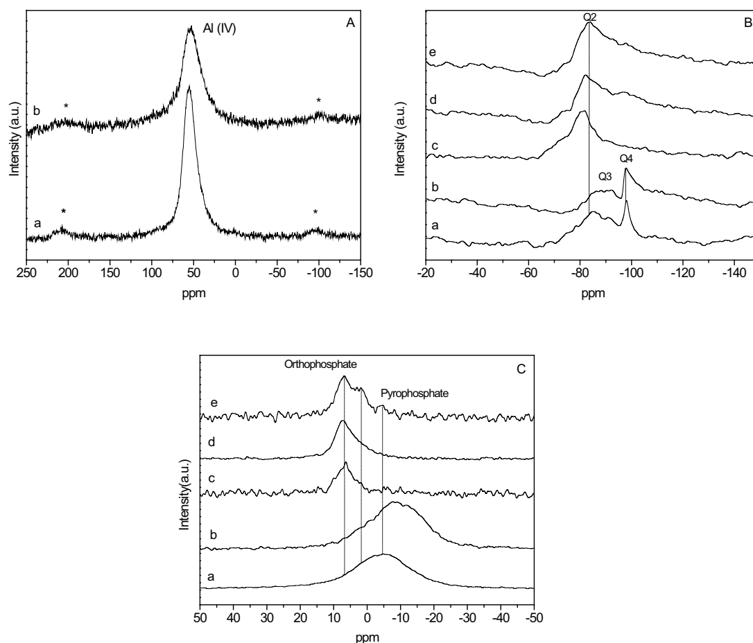
Figure 9 - 27 Al MAS NMR (A) and 29 Si MAS NMR (B) and 31 P MAS NMR spectra (C) of MMT/K 2 HPO 4 residues after 30 min (a) and after 31 days (b), talc/K 2 HPO 4 residues after 30 min (Bc, Cc), after 7 days (Bd, Cd) and after 31 days (Be, Ce).
