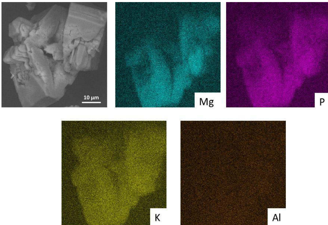
Figure 15 – EDX images of MgAl 200 /K 2 HPO 4 residues after 30 minutes.
