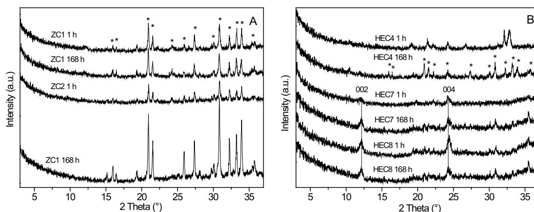
Figure 7 - XRD patterns of solid residues for Z mill (A) and for HE mill (B).* - K-Struvite; 002 and 004 indicate the basal peaks of chrysotile.
