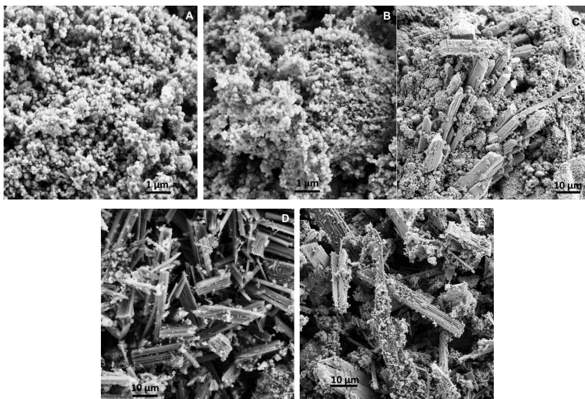
Figure 10 - SEM images of MMT/ \text{K}_2\text{HPO}_4 residues after 30 minutes (A), 31 days (B) and talc/ \text{K}_2\text{HPO}_4 residues after 30 minutes (C), 7 days (D) and 31 days (E).
