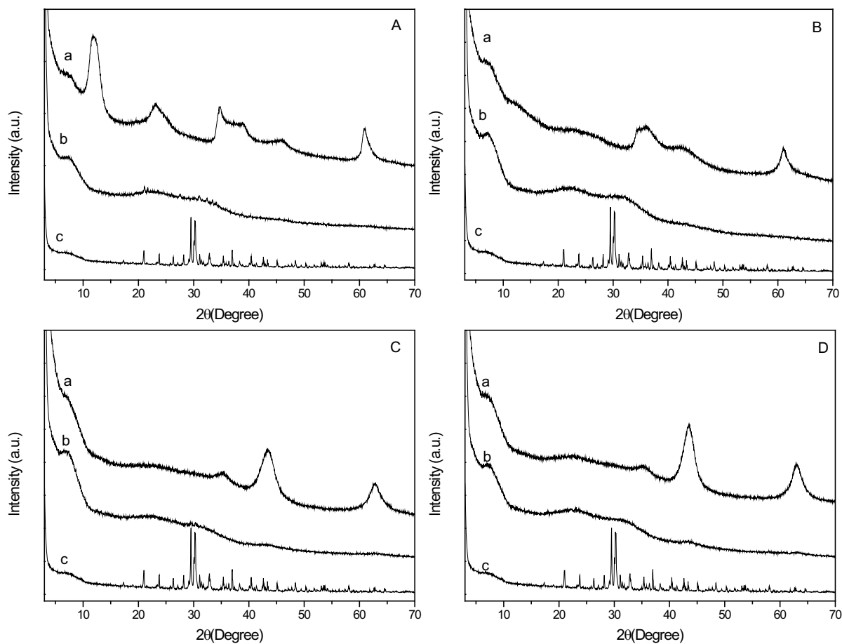
Figure 3– XRD data of Mg_2Al(OH)_6(CO_3) \cdot 3H_2O calcined at: 200°C (Aa); 300°C (Ba); 400°C (Ca); 500°C (Da). Milled samples (Ab; Bb; Cb; Db) and K_2HPO_4 (Ac; Bc; Cc; Dc) respectively.
