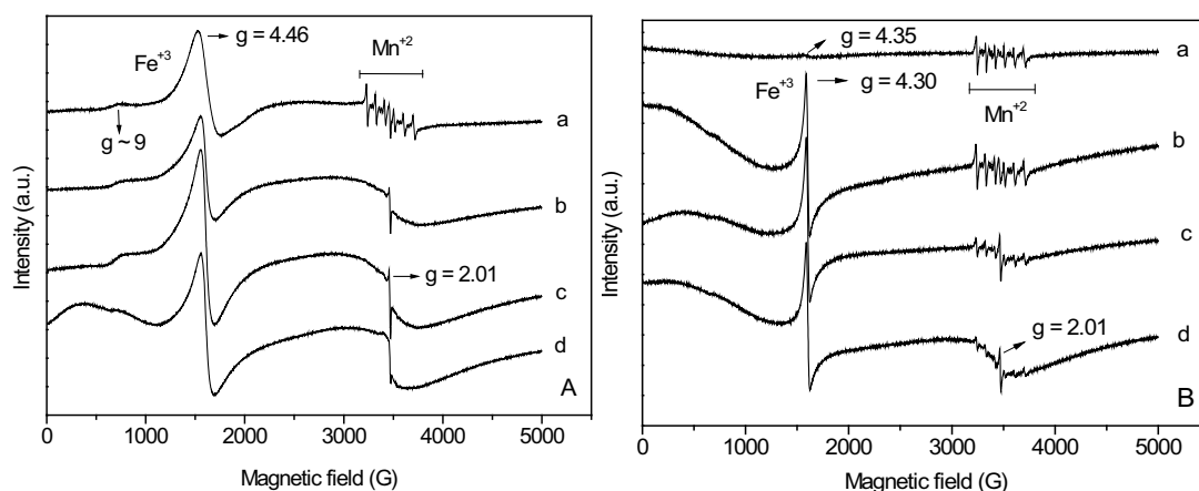
Figure 8 – EPR spectra of raw montmorillonite (Aa) and samples after milling for 3 h (Ab); 6 h (Ac); 9 h (Ad); raw talc (Ba) and samples after milling for 6 h (Bb); 9 h (Bc); 12 h (Bd).
