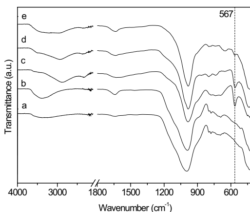
Figure 8 - FTIR spectra of MMT/ K_2HPO_4 residues after 30 min (a), MMT/ K_2HPO_4 residues after 31 days (b), talc/ K_2HPO_4 residues after 30 min (c), talc/ K_2HPO_4 residues after 7 days (d) and talc/ K_2HPO_4 residues after 31 days (e). MR = 1:2 and milling times of 9 h and 12 h for MMT and talc, respectively.
