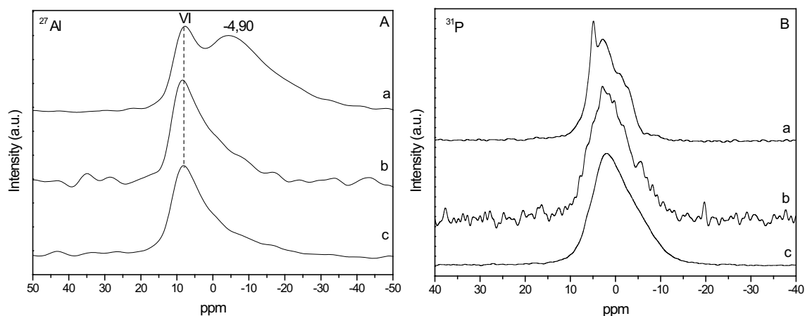
Figure 17 – Solid state NMR spectra of ^{27}\text{Al} for the solid residues of the \text{MgAl}_{200}/\text{K}_2\text{HPO}_4 systems after 30 min (Aa), 7 days (Ab) and after 31 days (Ac) and ^{31}\text{P} NMR spectra of the \text{MgAl}_{200}/\text{K}_2\text{HPO}_4 systems after 30 min (Ba), 7 days (Bb) and after 31 days (Bc).
