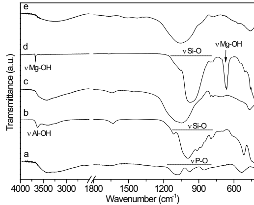
Figure 2 – FTIR spectra of K_2HPO_4 (a), MMT (b), milled MMT/ K_2HPO_4 (c), talc (d) and milled Talc/ K_2HPO_4 (e). MR = 1:2 and milling times of 9 h and 12 h for MMT and talc, respectively.
