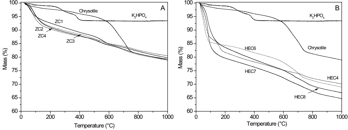
Figure 4 - Thermogravimetric (TGA) curves of samples ground in Z mill (A) and HE mill (B).
