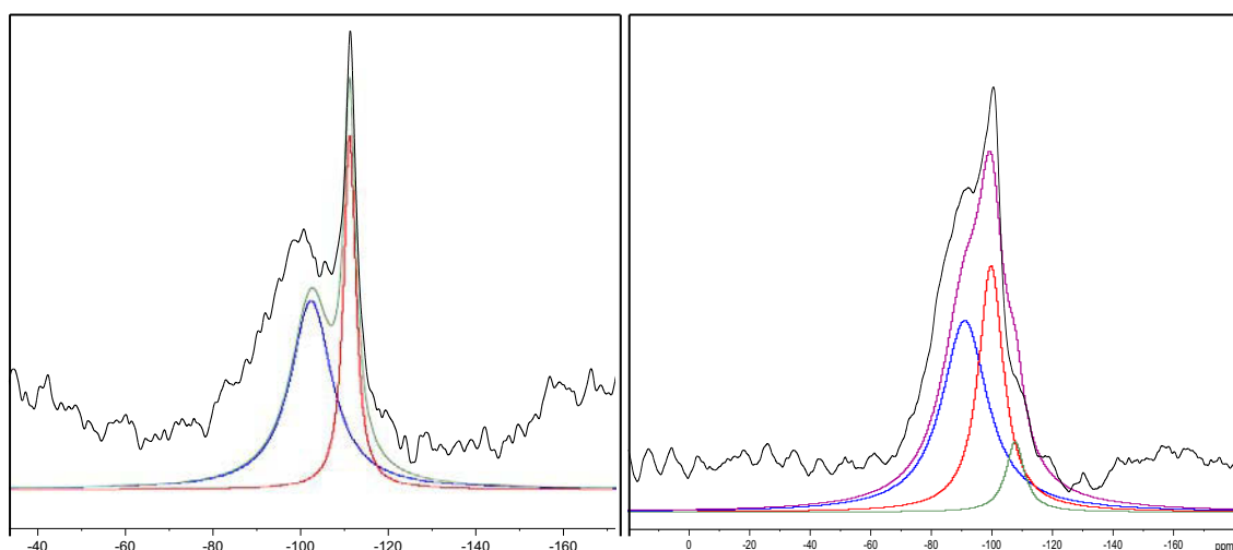
Figure 8 – ^{29}\text{Si} MAS NMR deconvoluted spectra of samples after milling montmorillonite for 3 h (left) and talc for 6 h (right).
