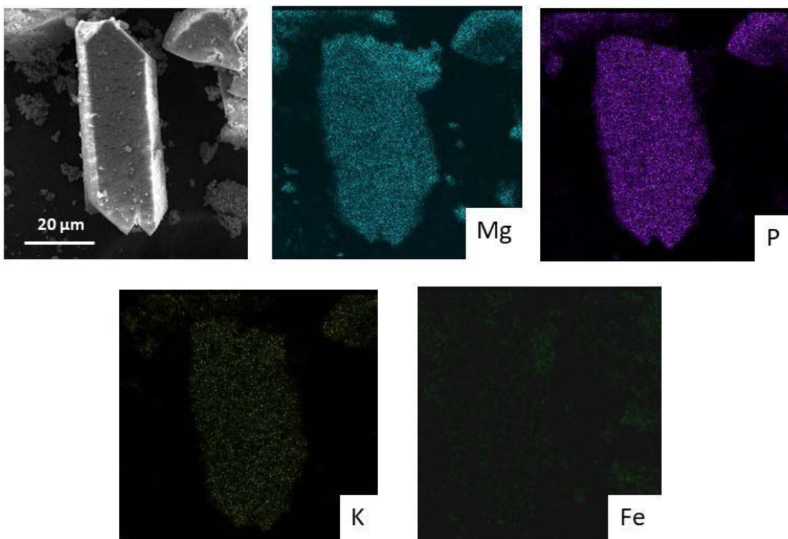
Figure 16 – EDX images of \text{MgFe}_{200}/\text{K}_2\text{HPO}_4 residues after 30 minutes.
