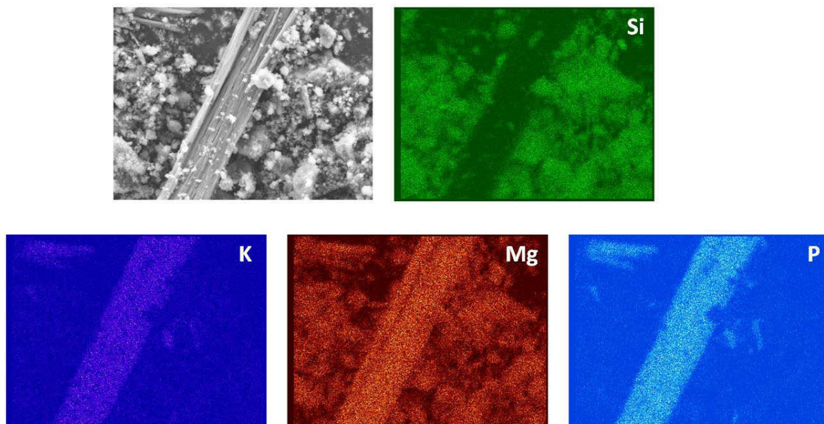
Figure 11- EDX mapping analyses of talc/ K_2HPO_4 residues after 7 days.
