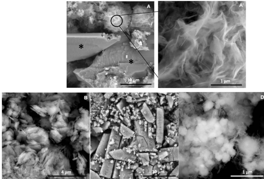
Figure 8 - SEM images of solid residues of ZC2 after 168 h of release (A, A'); HEC4 after 1 h (B) and after 168 h of release (C); HEC8 after 168 h of release (D). K-Struvite indicated by an *.
