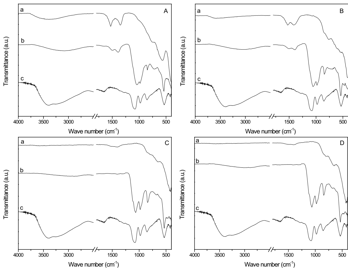
Figure 5 – FTIR data of \text{Mg}_2\text{Al}(\text{OH})_6(\text{CO}_3)\cdot 3\text{H}_2\text{O} calcined at: 200°C(Aa); 300°C (Ba); 400°C (Ca); 500°C (Da). Milled samples (Ab; Bb; Cb; Db) and \text{K}_2\text{HPO}_4 (Ac; Bc; Cc; Dc) respectively.
