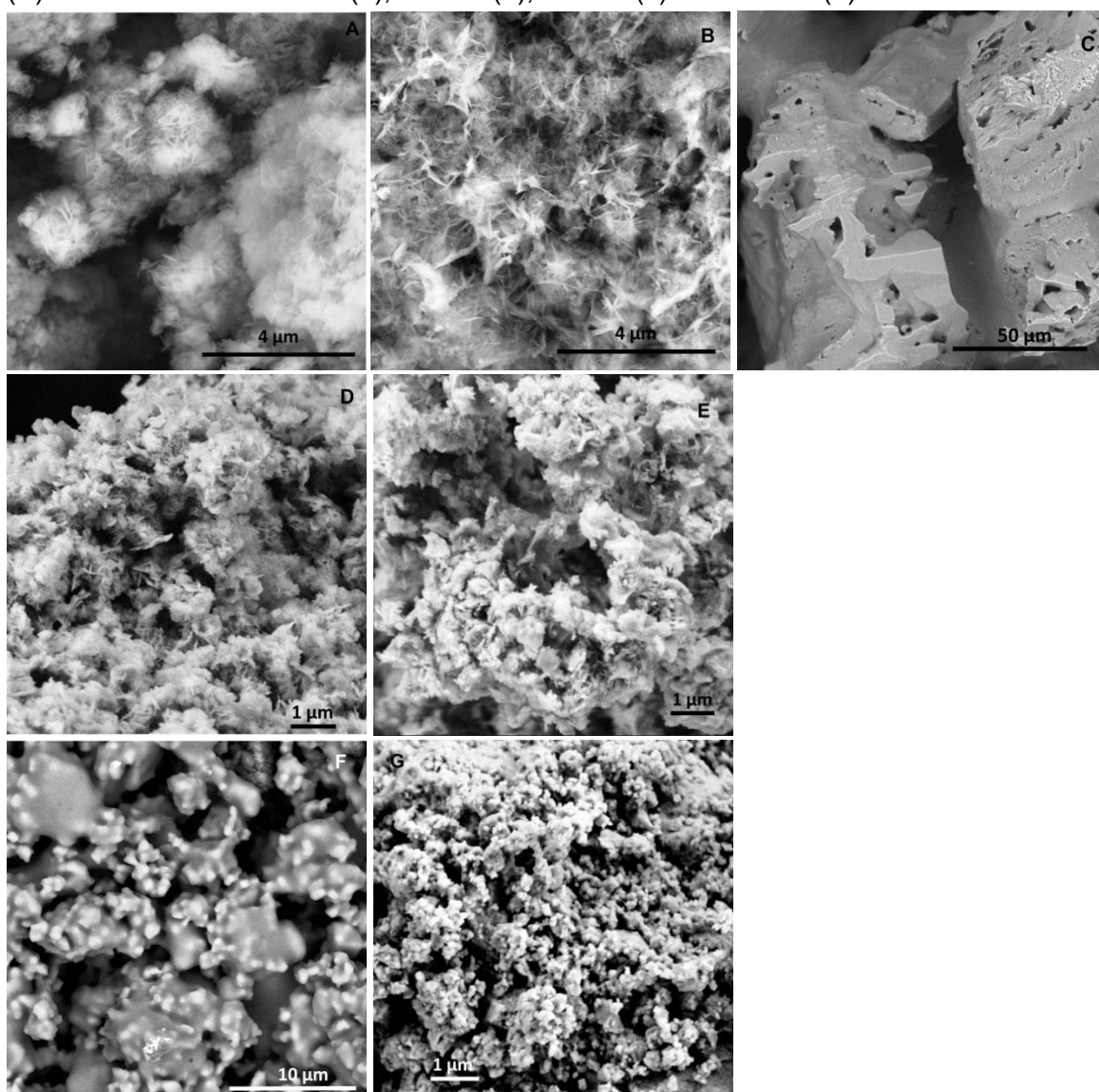
Figure 8 – SEM images of Mg_2Al(OH)_6(CO_3) \cdot 3H_2O (A), Mg_2Fe(OH)_6(CO_3) \cdot 2.5H_2O (B), K_2HPO_4 (C), MgAl calcined at 200 °C (D), MgFe calcined at 200 °C (E), MgAl_{200}/K_2HPO_4 (F), MgFe_{200}/K_2HPO_4 (G).
