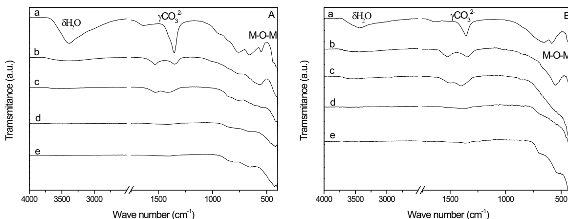
Figure 2 – FTIR data of \text{Mg}_2\text{Al}(\text{OH})_6(\text{CO}_3)\cdot 3\text{H}_2\text{O} (Aa); \text{Mg}_2\text{Fe}(\text{OH})_6(\text{CO}_3)\cdot 2.5\text{H}_2\text{O} (Ba) and calcined samples at: 200^\circ\text{C} (Ab; Bb); 300^\circ\text{C} (Ac; Bc); 400^\circ\text{C} (Ad; Bd); 500^\circ\text{C} (Ae; Be) respectively.
