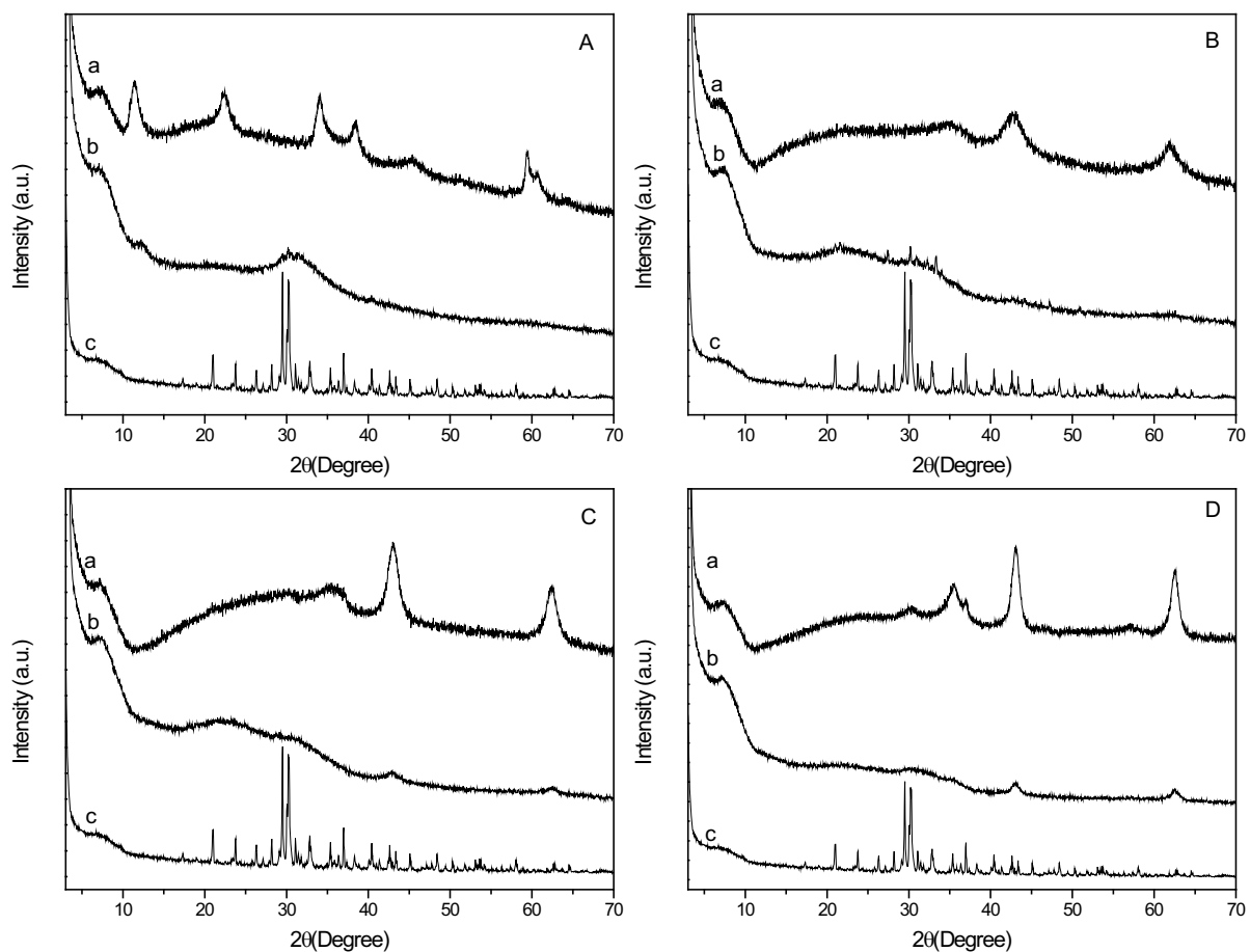
Figure 4 – XRD data of \text{Mg}_2\text{Fe}(\text{OH})_6(\text{CO}_3) \cdot 2.5\text{H}_2\text{O} calcined at: 200°C (Aa); 300°C (Ba); 400°C (Ca); 500°C (Da). Milled samples (Ab; Bb; Cb; Db) and \text{K}_2\text{HPO}_4 (Ac; Bc; Cc; Dc) respectively.
