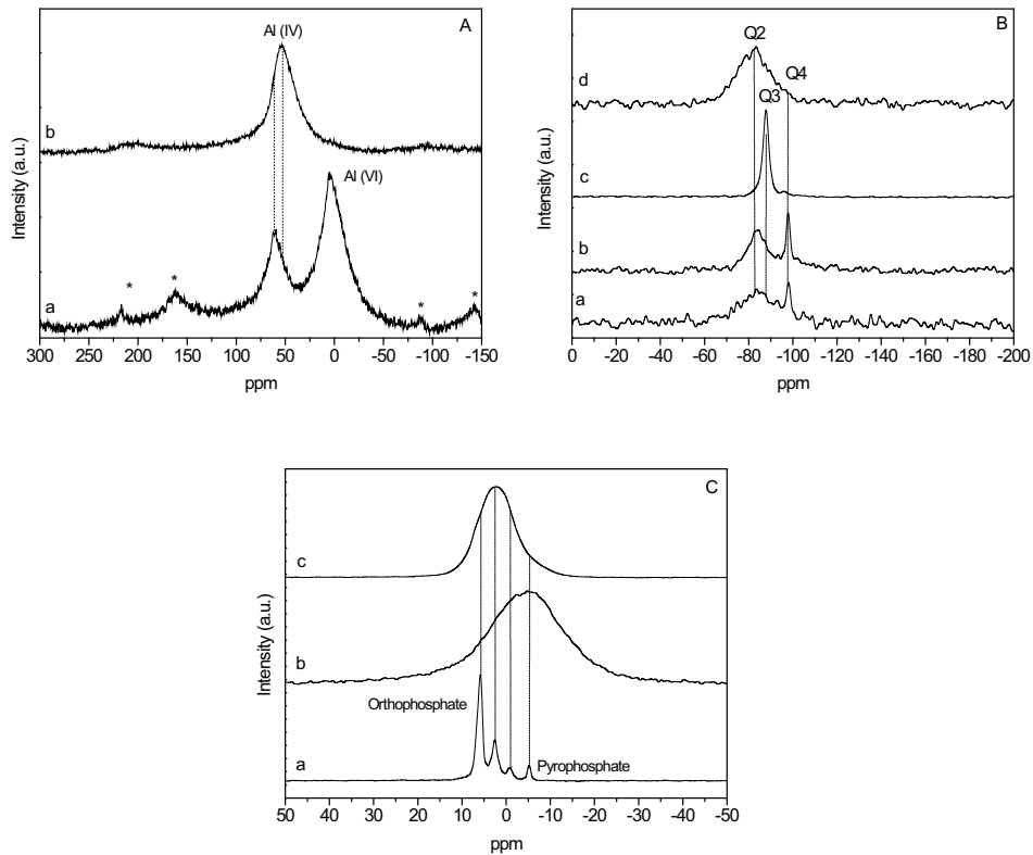
Figure 3 - ^{27}Al MAS NMR spectra of MMT (Aa) and milled MMT/ K_2HPO_4 (Ab); ^{29}Si MAS NMR spectra of MMT (Ba), milled MMT/ K_2HPO_4 (Bb), talc (Bc) and milled talc/ K_2HPO_4 (Bd); ^{31}P MAS NMR spectra of K_2HPO_4 (Ca), milled MMT/ K_2HPO_4 (Cb) and milled talc/ K_2HPO_4 (Cc). MR = 1:2 and milling times of 9 h and 12 h for MMT and talc, respectively.
