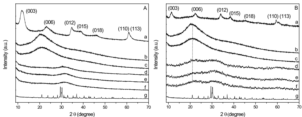
Figure 18 - X-ray diffractograms for K 2 HPO 4 (Ag and Bg), Mg 2 Al(OH) 6 (CO 3 ).3H 2 O (Aa), Mg 2 Fe(OH) 6 (CO 3 ).2.5H 2 O (Ba), CMC (Ab and Bb), CMC milled for 3 h (Ac and Bc) and samples: HFC1 (Ad), HFC2 (Ae), HFC3 (Af), HFC4 (Bd), HFC5 (Be) and HFC6 (Bf).
