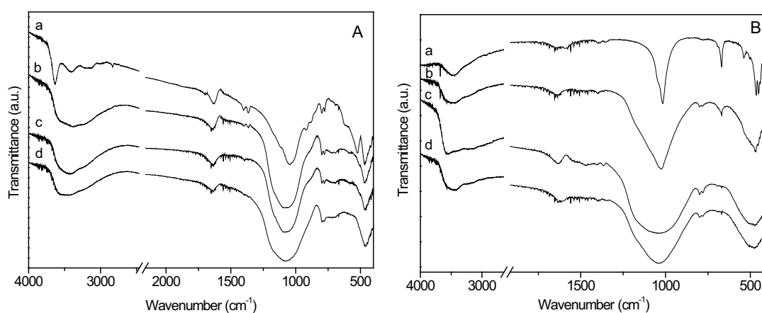
Figure 4 – FTIR spectra of raw montmorillonite (Aa) and samples after milling for 3 h (Ab); 6 h (Ac); 9 h (Ad); raw talc (Ba) and samples after milling for 6 h (Bb); 9 h (Bc); 12 h (Bd).
