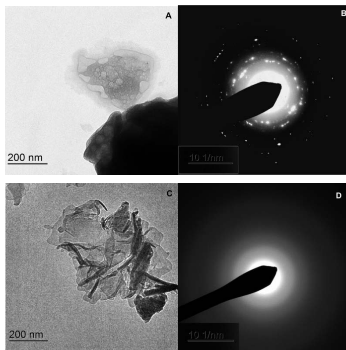
Figure 9 - TEM images (A,C) and SAED spectra (B,D) for the sample HEC4 after 1 h of release.
