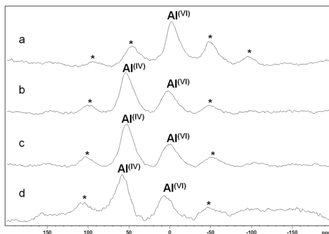
Figure 9 - ^{27}\text{Al} MAS NMR spectra of raw montmorillonite (a), and samples after milling for 3 h (b); 6 h (c); 9 h (d). * Side rotating bands.
