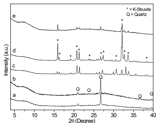
Figure 7 - XRD patterns of MMT/ K_2HPO_4 residues after 30 min (a), MMT/ K_2HPO_4 residues after 31 days (b), talc/ K_2HPO_4 residues after 30 min (c), talc/ K_2HPO_4 residues after 7 days (d) and talc/ K_2HPO_4 residues after 31 days (e). MR = 1:2 and milling times of 9 h and 12 h for MMT and talc, respectively.
