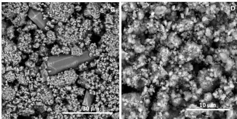
Figure 14 - SEM images of MgAl 200 /K 2 HPO 4 residues after 1 h ( A) and 168 h ( B), also of MgFe 200 /K 2 HPO 4 residues after 30 minutes (C) and 168 h (D).
