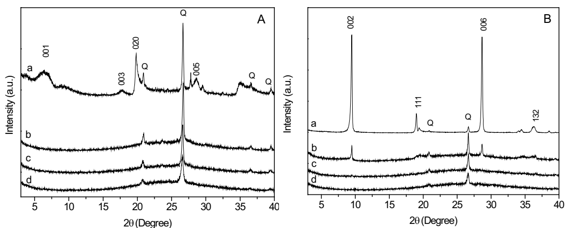
Figure 3 - X-ray diffraction patterns of raw montmorillonite (Aa) and samples after milling for 3 h (Ab); 6 h (Ac); 9 h (Ad); raw talc (Ba) and samples after milling for 6 h (Bb); 9 h (Bc); 12 h (Bd)
