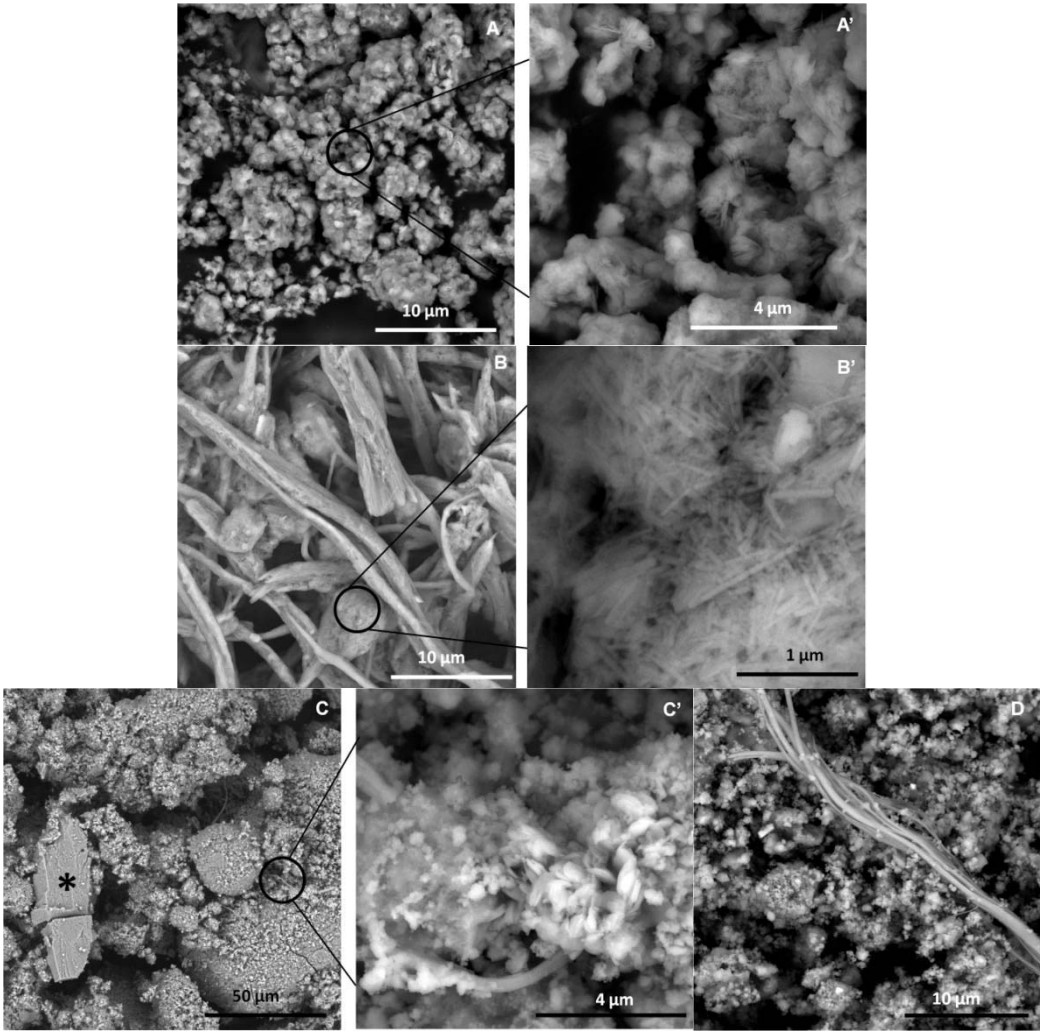
Figure 3 - SEM images of HEC4 (A,A'), HEC6 (B,B'), HEC7 (C,C') and HEC8 (D), respectively. K-Struvite indicated by an *.
