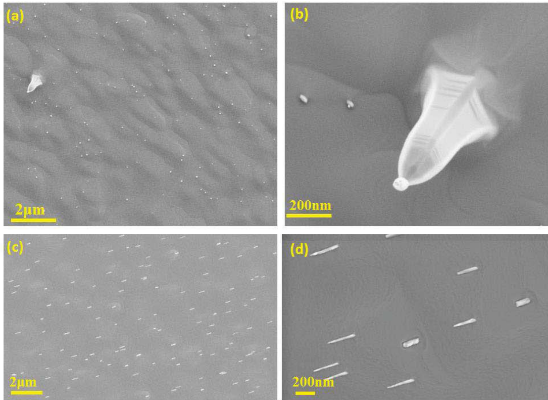
Fig. 2.23: SEM images of doped GaAs nanowires with 30 \text{ cm}^3/\text{min} of diethylzinc (a) and (b) and 80 \text{ cm}^3/\text{min} for (c) and (d).
