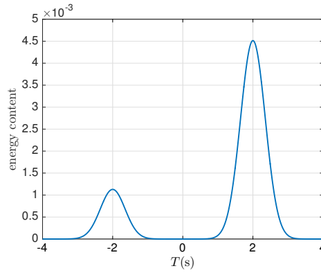
Fig. 3.2 Energy content of F(t) (composed of two disjoint gaussian functions): \int_{\mathbb{R}} \mathbf{W}[F](t; \omega) d\omega normalized to total energy
