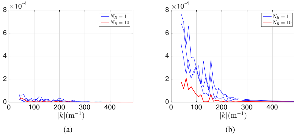
Fig. 4.21 Residual errors along \omega = \pm c_0 k for coherent wave: (a) |R^+| , (b) |R^-|
