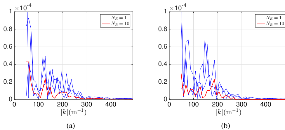
Fig. 4.24 Residual errors along \omega = \pm c_0 k for incoherent wave: (a) |R_T^{\text{sd}}| , (b) |R_{TS}^{\text{sd}}|
