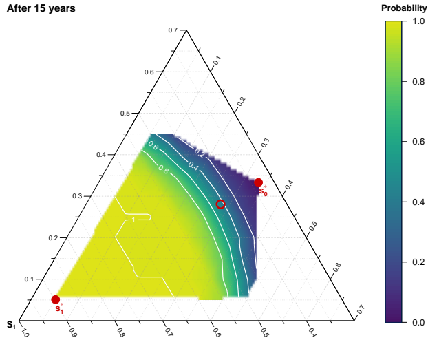
Figure 6.10. Probability of selecting equilibrium s_1^* after 15 years. Taking any point within the triangle as a starting point, the colour scale depicts the probability of the system to be closer than 0.3 units to s_1^* after 15 years. The area was sampled using 33 starting points with 1000 simulations for each, and the probability functions was obtained by linear interpolation..
