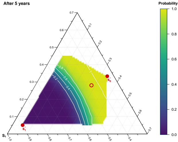
Figure 6.4. Probability of selecting equilibrium s_0^* after 5 years. Taking any point within the triangle as a starting point, the colour scale depicts the probability of the system to be closer than 0.3 units to s_0^* after 5 years. The area was sampled using 33 starting points with 1000 simulations for each, and the probability functions was obtained by linear interpolation.
