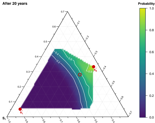
Figure 6.7. Probability of selecting equilibrium s_0^* after 20 years. Taking any point within the triangle as a starting point, the colour scale depicts the probability of the system to be closer than 0.3 units to s_0^* after 20 years. The area was sampled using 33 starting points with 1000 simulations for each, and the probability functions was obtained by linear interpolation.
