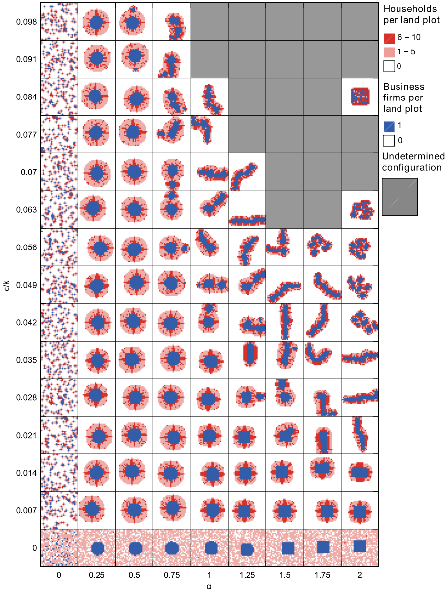
Figure 4.5. Simulated long-run equilibrium configurations. Simulated long-run configurations are given for 135 parametrizations on \alpha and c/k , where \alpha is the distance-decay parameter of the agglomeration economies and c/k is the relative commuting cost. If no long-run equilibrium was reached, the configuration is set undetermined.
