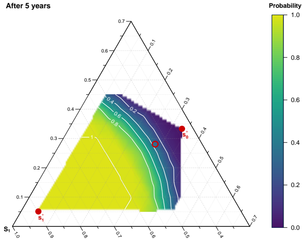
Figure 6.8. Probability of selecting equilibrium s_1^* after 5 years. Taking any point within the triangle as a starting point, the colour scale depicts the probability of the system to be closer than 0.3 units to s_1^* after 5 years. The area was sampled using 33 starting points with 1000 simulations for each, and the probability functions was obtained by linear interpolation.
