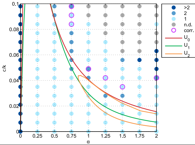
Figure 4.10. Pre-border corrected multicentricity of the simulated long-run equilibrium configurations. Blue colour scale denotes the number of disconnected business districts in the simulated long-run equilibrium configurations for 135 parametrizations on \alpha and c/k , where \alpha is the distance-decay parameter of the agglomeration economies and c/k is the relative commuting cost. Pink circles highlight the runs that underwent border effects. Coloured lines delineate the equilibrium conditions of the continuous completely mixed ( U_0 ), monocentric ( U_1 ), and rotational duocentric ( U_2 ) urban configurations.
