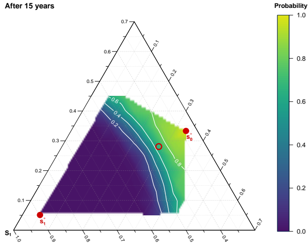
Figure 6.6. Probability of selecting equilibrium s_0^* after 15 years. Taking any point within the triangle as a starting point, the colour scale depicts the probability of the system to be closer than 0.3 units to s_0^* after 15 years. The area was sampled using 33 starting points with 1000 simulations for each, and the probability functions was obtained by linear interpolation.
