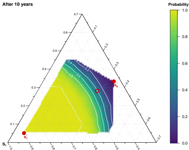
Figure 6.9. Probability of selecting equilibrium s_1^* after 10 years. Taking any point within the triangle as a starting point, the colour scale depicts the probability of the system to be closer than 0.3 units to s_1^* after 10 years. The area was sampled using 33 starting points with 1000 simulations for each, and the probability functions was obtained by linear interpolation.
