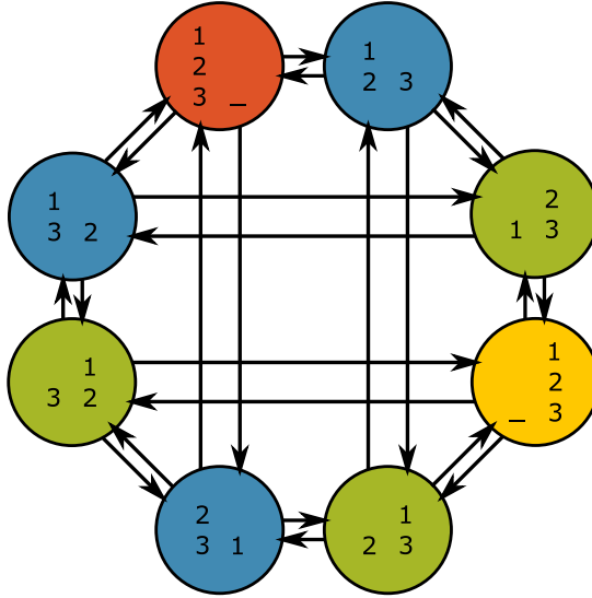
Figure 5.4. Partition of the states into macro-states in the case N = 3 and M = 2 . Each circle represents a state. Colours depict the different items of the partition, and arrows show which state can be related to another by the move of a single agent.
