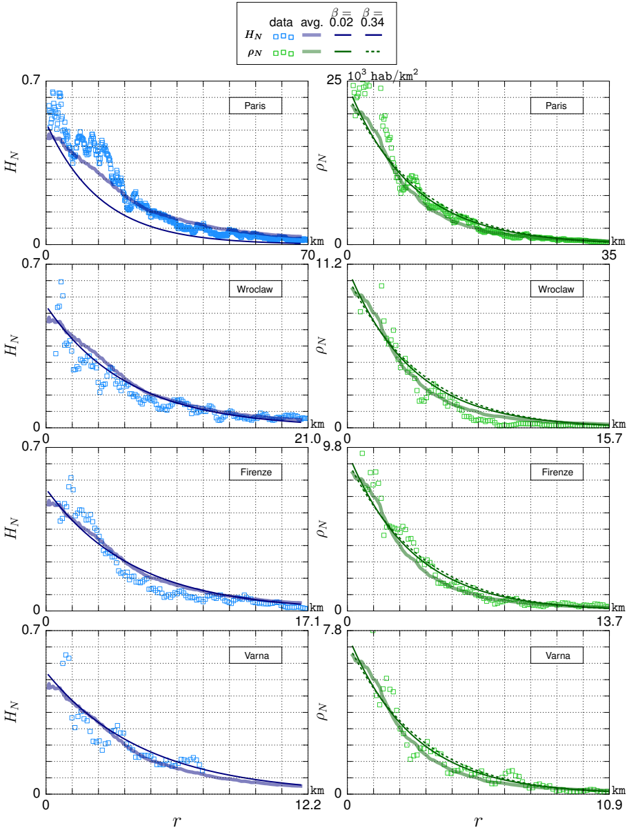
Figure 3.7. Second summary plot of the results. Fitted average profiles compared to individual profiles. Left panel: housing share profile. Right panel: population density profile. Axes have been rescaled to maintain the average curves at the same position across subplots.
