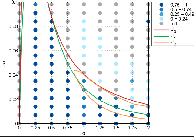
Figure 4.11. Circularity of the simulated long-run equilibrium configurations. Blue colour scale denotes the number of disconnected business districts in the simulated long-run equilibrium configurations for 135 parametrizations on \alpha and c/k , where \alpha is the distance-decay parameter of the agglomeration economies and c/k is the relative commuting cost. Coloured lines delineate the equilibrium conditions of the continuous completely mixed ( U_0 ), monocentric ( U_1 ), and rotational duocentric ( U_2 ) urban configurations.
