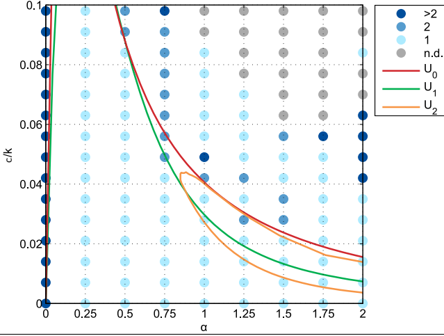
Figure 4.6. Multicentricity of the simulated long-run equilibrium configurations. Blue colour scale denotes the number of disconnected business districts in the simulated long-run equilibrium configurations for 135 parametrizations on \alpha and c/k , where \alpha is the distance-decay parameter of the agglomeration economies and c/k is the relative commuting cost. Coloured lines delineate the equilibrium conditions of the continuous completely mixed ( U_0 ), monocentric ( U_1 ), and rotational duocentric ( U_2 ) urban configurations.
