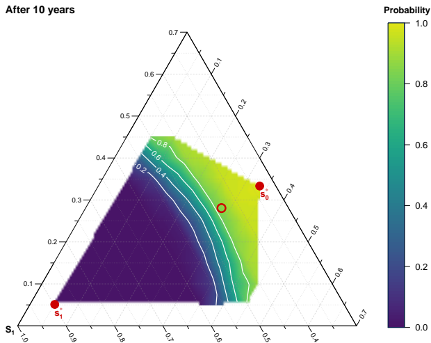
Figure 6.5. Probability of selecting equilibrium s_0^* after 10 years. Taking any point within the triangle as a starting point, the colour scale depicts the probability of the system to be closer than 0.3 units to s_0^* after 10 years. The area was sampled using 33 starting points with 1000 simulations for each, and the probability functions was obtained by linear interpolation.
