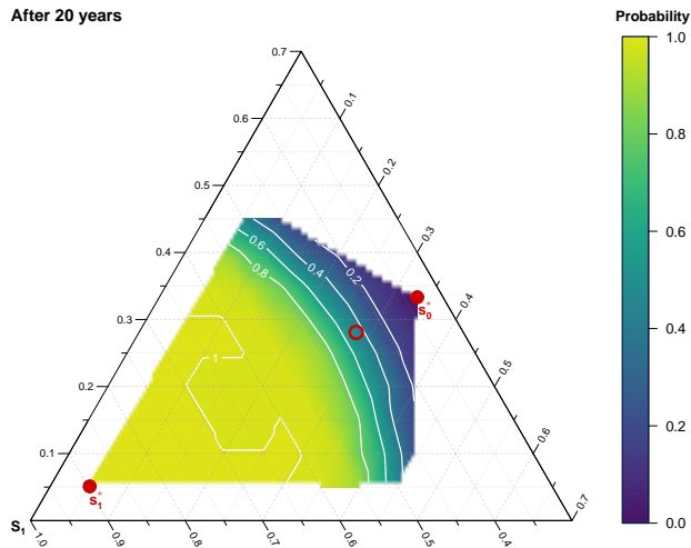
Figure 6.11. Probability of selecting equilibrium s_1^* after 20 years. Taking any point within the triangle as a starting point, the colour scale depicts the probability of the system to be closer than 0.3 units to s_1^* after 20 years. The area was sampled using 33 starting points with 1000 simulations for each, and the probability functions was obtained by linear interpolation..
