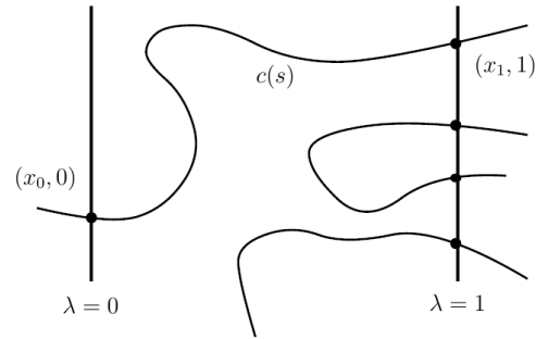
Figure 1.1: Different zero paths.
