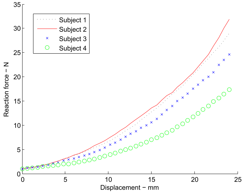
Figure 4.6: Experimental data - Response of 4 subjects to a localized compression of 25 mm depth with a 30 mm diameter cylinder
