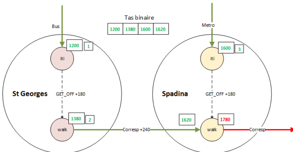
FIGURE 20 – Interdictions des correspondance multiples
