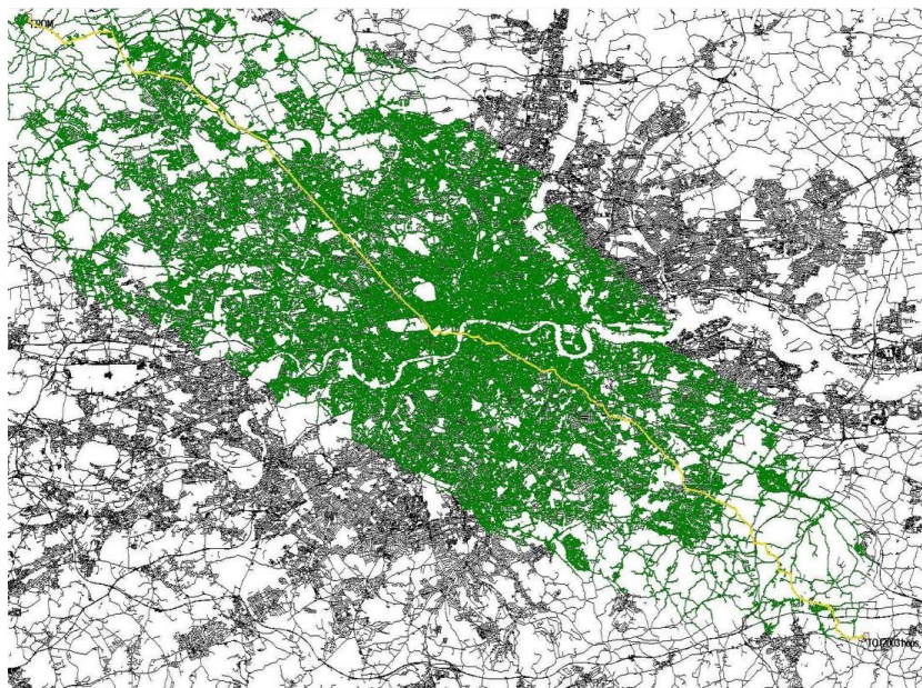
FIGURE 11 – Algorithme A^*
