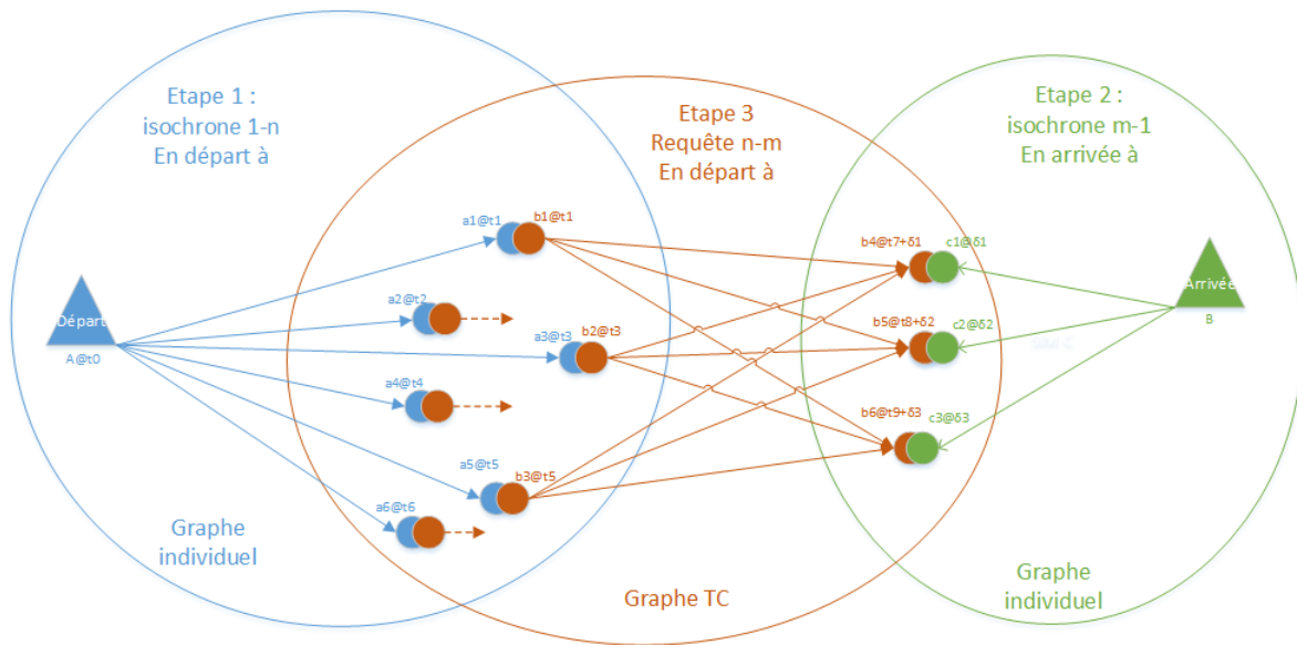
FIGURE 18 – Calcul combiné marche/TC/marche
