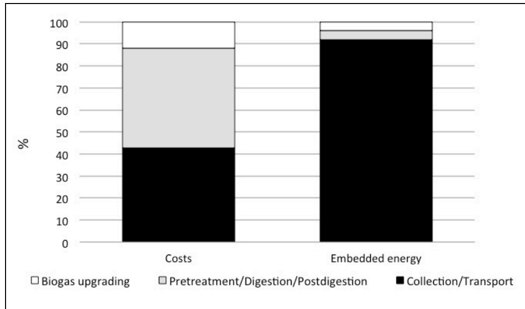
Figure 4-6 Distribution of resources consumption between the different phases of the AD chain for the economic and energy indicators
