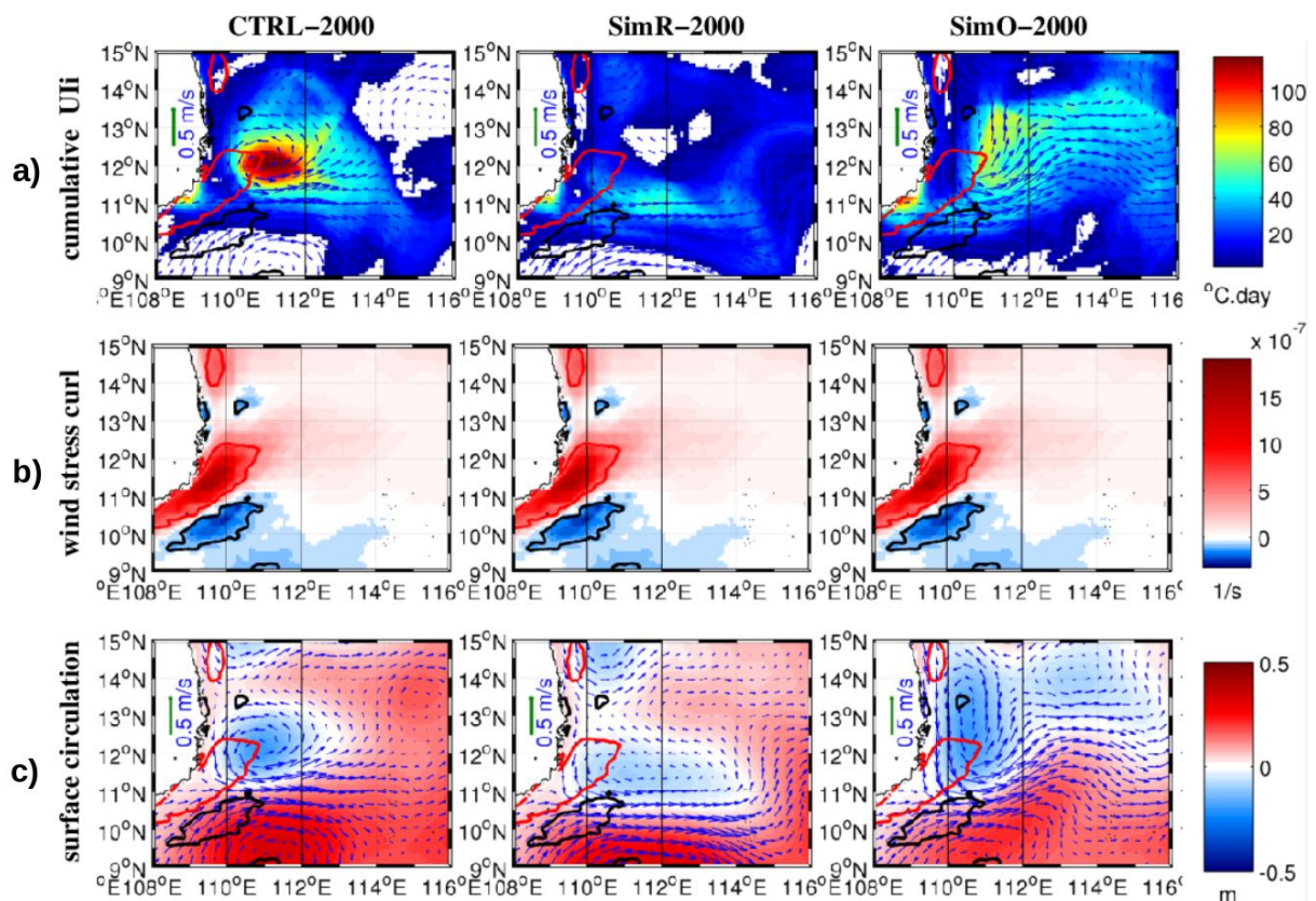
Figure 4.8: Similar to Figure 4.7 but among CTRL and SimR and SimO in the year 2000 whose wind fields are the same.
