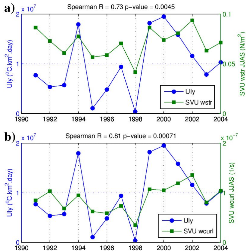
Figure 4.6. Upwelling and wind relation. Yearly time series of upwelling strength Uly ( ^{\circ}\text{C}\cdot\text{km}^2\cdot\text{day} , blue) in CTRL and mean JJAS SVU wind stress (a, \text{N}\cdot\text{m}^{-2} , green) and mean JJAS SVU wind stress curl (b, \text{s}^{-1} , green) from CFSR. The correlation coefficient and p-value between those time series is also indicated.
