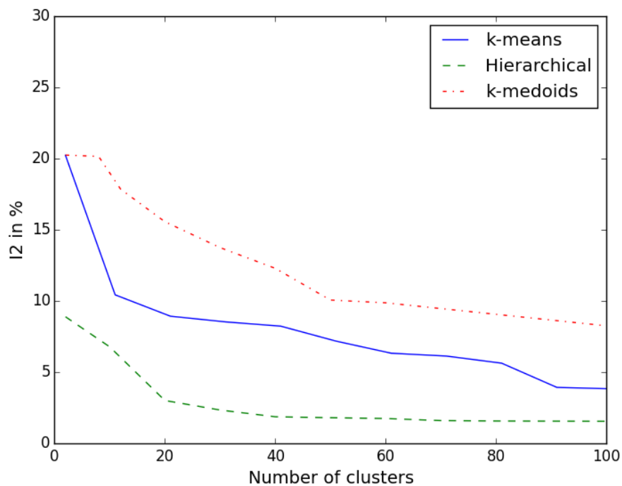
FIGURE II.4: Average redispach effort, as a function of the number of clusters, for 300 scenarios corresponding to different levels of net load.
