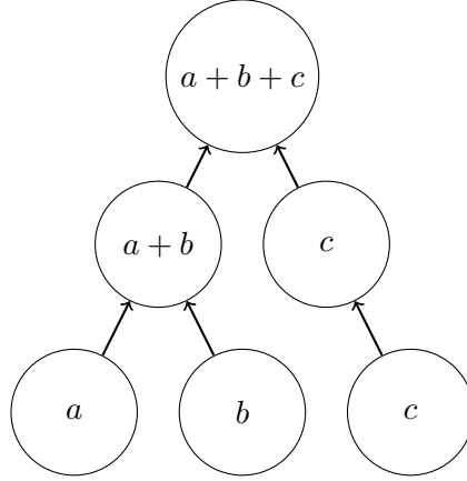
FIGURE II.1: Graphical representation of hierarchical clustering.
