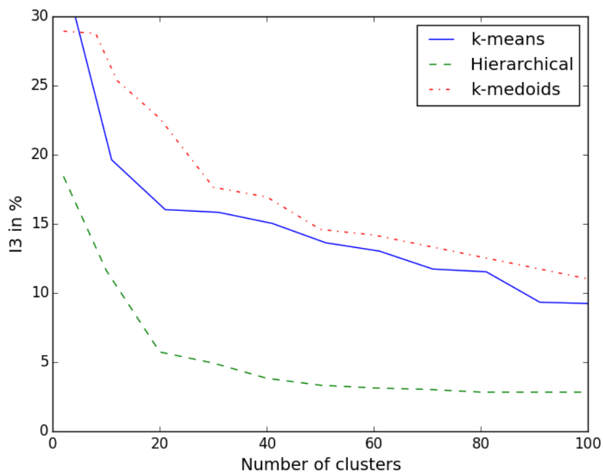
FIGURE II.5: Maximum redispach effort, as a function of the number of clusters, for 300 scenarios corresponding to different levels of net load.
