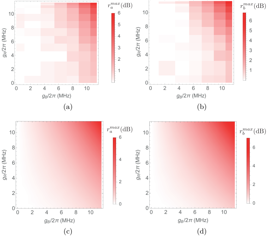
Figure 38: Measured single mode anti-squeezing on modes a (a) and b (b). Antisqeezing parameter r_{a,b}^{max} in dB is plotted as a function of pump coupling rates g_B and g_R determined from noise measurements Fig. 20 and Fig. 29a. (c) Predicted antisqeezing from input-output theory for the mode a and (d) for the mode b .
