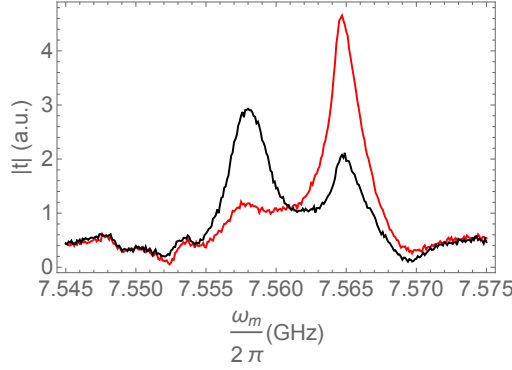
Figure 65: Amplitude of the signal transmitted by conversion from buffer to the memory as a function of frequency, for the qubit initially prepared in the ground state using the cooling protocol (red) and in the excited state (black).
