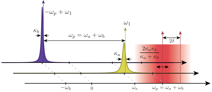
Figure 16: Pumping scheme in amplification mode. The two resonant modes a and b are represented by their Lorentzian response functions. The pump tone applied at the sum of their resonance frequencies provides the energy for the amplification process and determines the amplitude gain. The pump can be applied in the vicinity of \omega_a + \omega_b given by \gamma_0 = \frac{2\kappa_a\kappa_b}{\kappa_a + \kappa_b} \simeq \kappa_a . A signal injected on the mode a at the frequency \omega_1 will be amplified at that same frequency and converted to the mode b at the frequency \omega_c - \omega_1 within the amplifier bandwidth. If the pump is applied with a detuning 2\delta > 2\kappa , we are in a non standard regime of off-resonant pumping.
