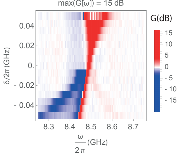
Figure 23: Measured gain in dB as a function of signal frequency f_a = \frac{\omega_a}{2\pi} and pump detuning \delta . For every detuning, the pump amplitude p_B is tuned so that the maximum gain \max(G[\omega]) = 15 dB. For detuning \delta < \kappa , there is one peak at \omega = \omega_a . For \delta > \kappa , there are two discernable peaks at \omega_a and \omega_a + 2\delta .
