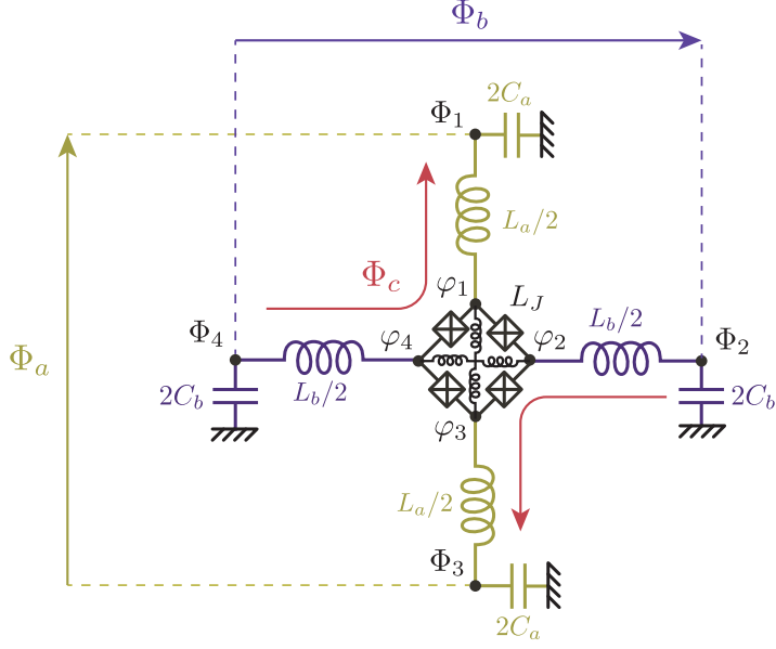
Figure 11: Lumped circuit model of the Josephson Mixer. \Phi_a and \Phi_b are the two differential \lambda/2 modes and \Phi_c is the common excitation mode.
