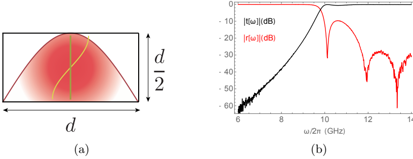
Figure 74: (a) Cross-section of a waveguide with largest supported wavelength mode TE_{10} . Planar \frac{\lambda}{2} buffer mode is represented in yellow. (b) Measured transmission and reflection coefficients for WR62 waveguide with cutoff frequency f_c = 9.5 GHz.
