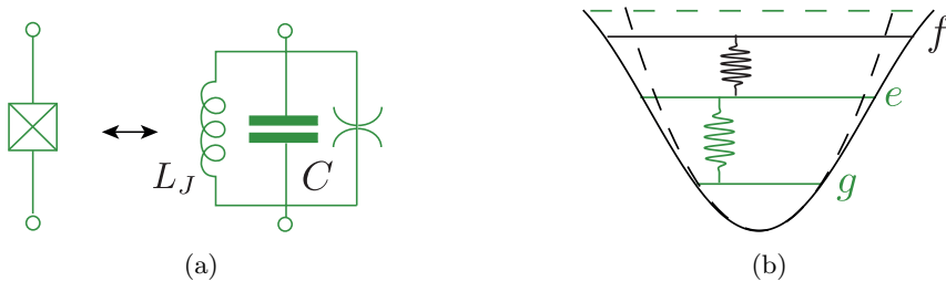
Figure 46: (a) Equivalent LC circuit of a Josephson junction. Transmon qubit is obtained by shunting the junction with a large capacitor formed by two big superconducting antennas. (b) Transmon energy levels in its electromagnetic phase potential.
