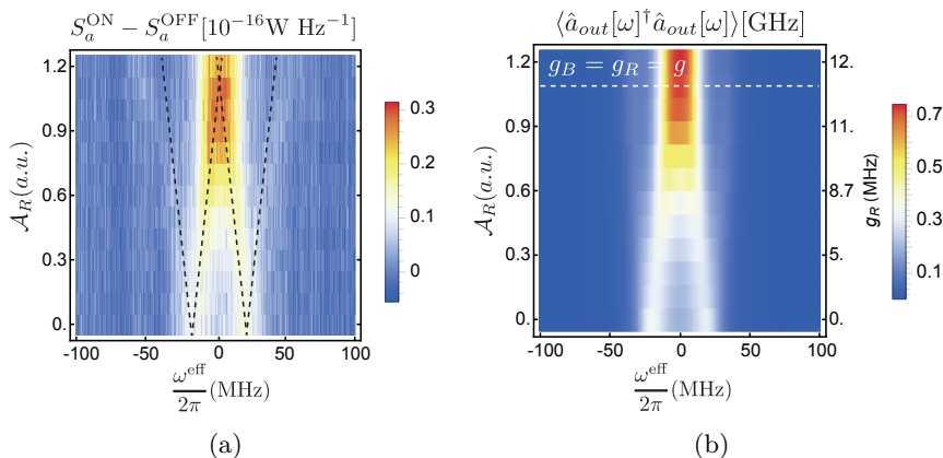
Figure 2: Spectroscopic evidence of the ultrastrong coupling. (a) Measured power spectral density of the ground state radiation. (b) Expected average number of photons in the outgoing mode. Each of the two resonances exhibits Rabi splitting proportional to the coupling rate g .
