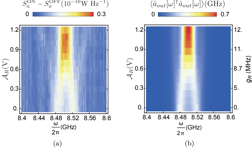
Figure 26: (a) Measured power spectral density on the output port of mode a as a function of frequency \omega and red pump amplitude \mathcal{A}_R in the proximity of the resonance frequency \omega_a of the mode a . The coupling of the blue pump is fixed to g_B = 2\pi \times 12.6 MHz. (b) The corresponding mean rate of emitted photons predicted from the input-output model Eq. (72).
