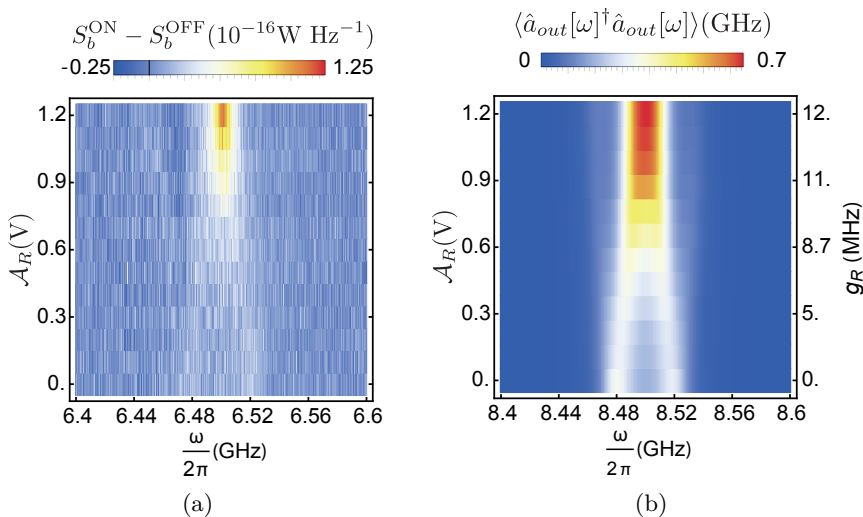
Figure 28: (a) Measured power spectral density on port b as a function of frequency \omega and red pump amplitude \mathcal{A}_R in the proximity of the resonance frequency \omega_b of the mode b . (b) Corresponding expectation value of the photon emission rate calculated from the input-output model.
