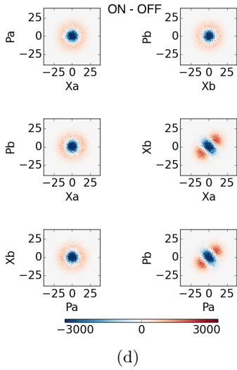
Figure 34: (a) Pulse sequence used in the experiment. Measured quadrature histograms in the EPR state with entangling pump (b) turned OFF, (c) turned ON and (d) subtraction between ON and OFF histograms for 6 different quadrature pairs. Each bin is 1 \times 1 wide and the color bars are expressed in number of counts.
