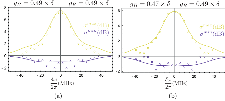
Figure 41: Measured minimum and maximum variance \sigma_{min} and \sigma_{max} as a function of frequency \delta\omega in the proximity of the origin of the rotating frame, corresponding to \omega_a + \delta in the laboratory frame. Figures (a) and (b) correspond to two different values of the coupling rate of the blue pump g_B . Full line corresponds to the expectation values calculated using the input-output theory.
