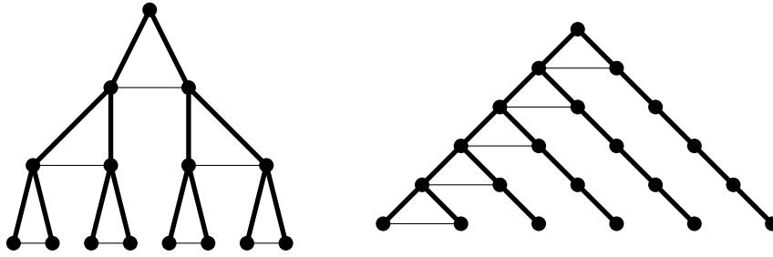
Figure 2.8: The graphs U_3 (left) and Q_5 (right).
