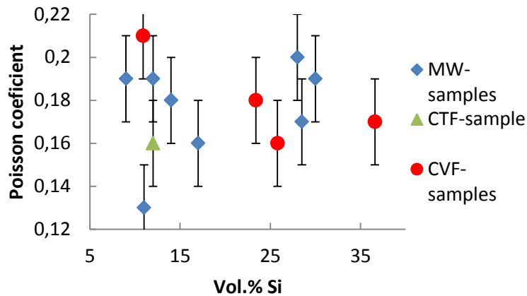
Figure III)47: Influence of the residual silicon amount on the Poisson coefficient
