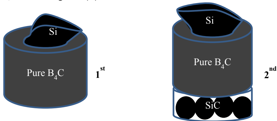
Figure III)1: Scheme of the two test rigs used for constant incident power tests
