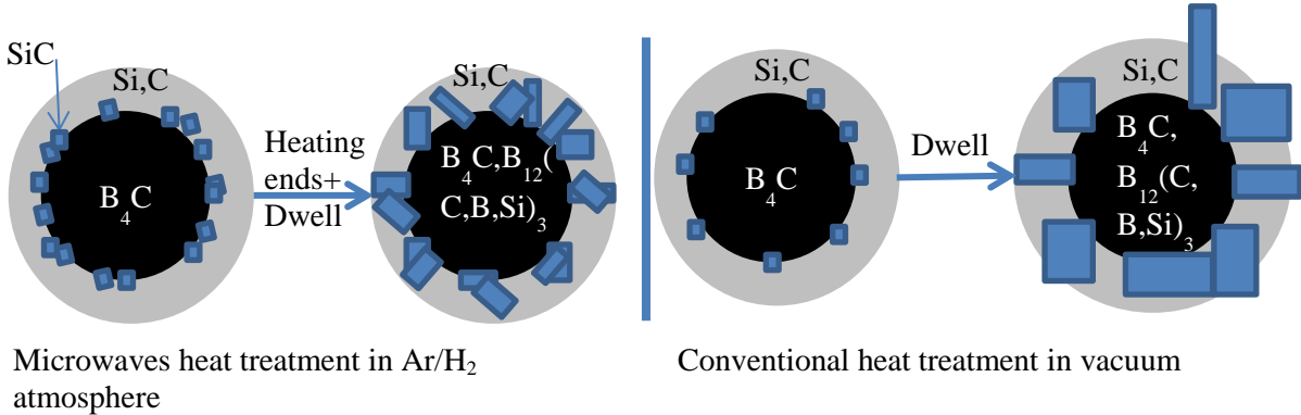
Figure III)43: Scheme of the silicon carbide precipitation
