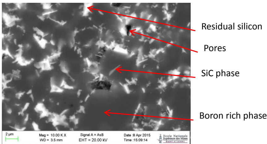
Figure III)14: Microstructure (SEM image) of the composite II. (Backscattered electron detector).
