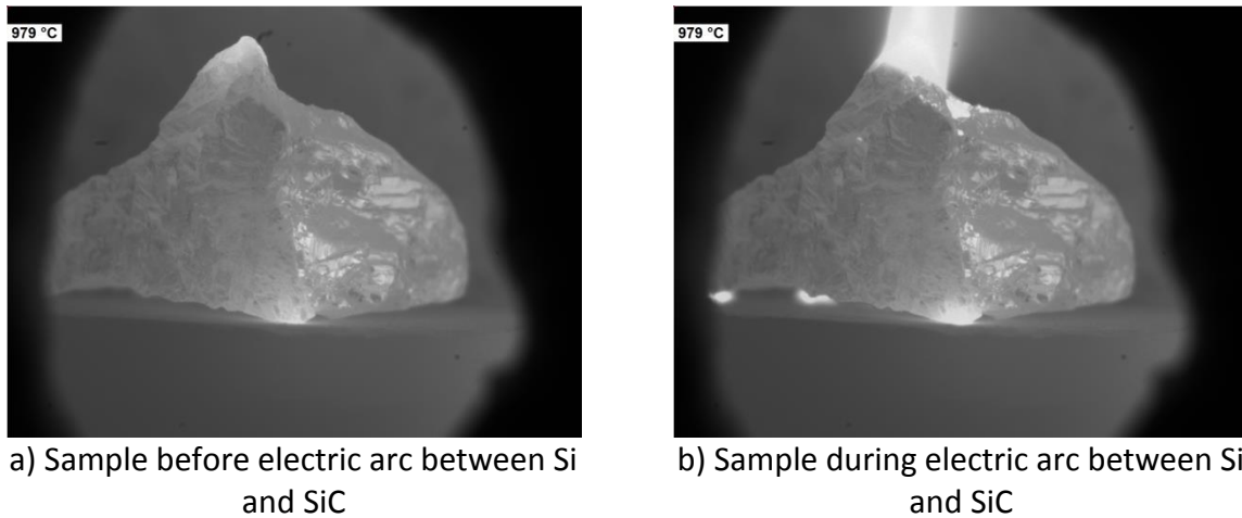
Figure III)6: Electric arc between SiC and silicon lump with local overheating
