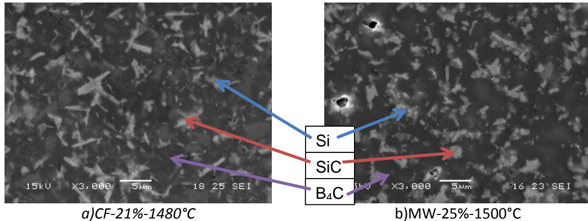
Figure III)36: Comparison of the microstructure of CVF and MW samples. SEM picture for secondary electron mode (SEI topography).
