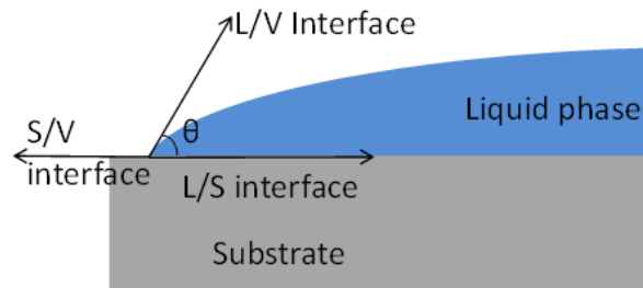
Figure I)4: Contact angle
