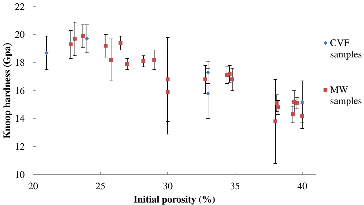
Figure III)51: Resume graph of compared hardness in function of the initial porosity
