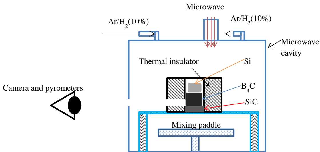
Figure II)3: scheme of the 2.45GHz microwaves cavity
