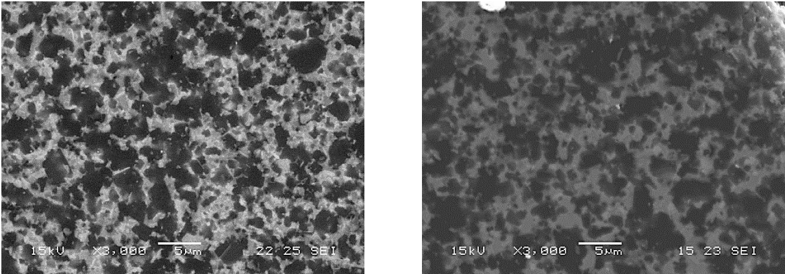
a) monomode heated sample b) multimode heated sample Figure III)30: Microstructure of a) monomode heated sample (40% Dth) and b) multimode sample (40% Dth)
