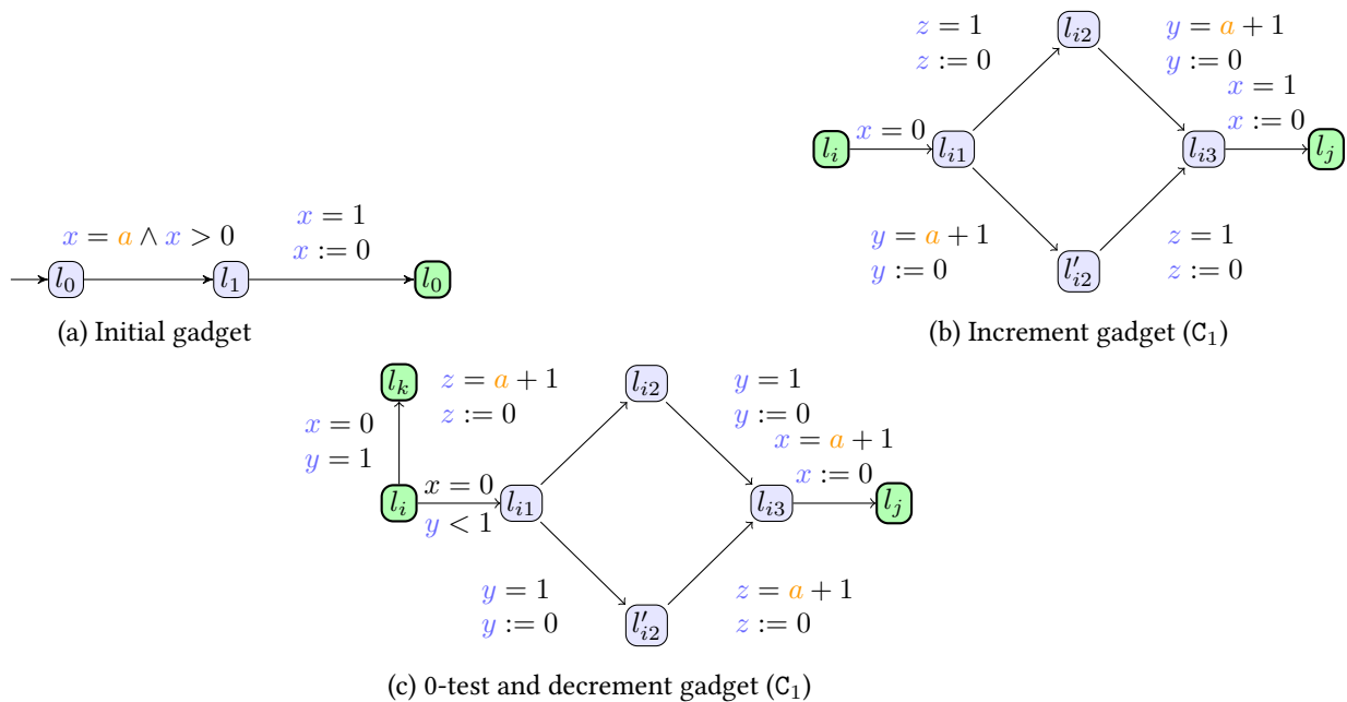
Figure 3.5 – EF-emptiness: gadgets
