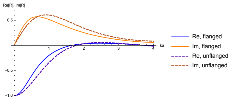
Figure 7.1 – Real and imaginary parts of the reflectance of a cylindrical orifice, approximated with Eq. 7.9, for the flanged (continuous lines) and unflanged (dashed lines) cases. In abscissa, the reduced frequency ka = \omega a / c , where a is the radius of the orifice.
