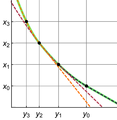
Figure 5.1 – Example of a nonlinear stiffness, represented by the convex, decreasing function x = f(y) , modeled piecewise with N = 3 parabolic sections. The functions f_0 , f_1 and f_2 are shown in broken lines, from black to orange. The function f is depicted in thick green continuous line. The discrete points (y_n, x_n) are in black, from which the parameters k_n , \kappa_n and h_n of the different pieces of the function f are calculated.
