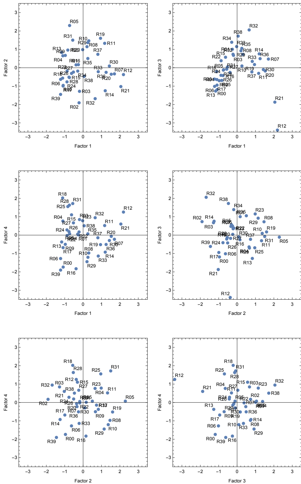
Figure C.2 – Plot of the canonical factors 1 to 4 of staticF (after standardization). The identifier of each individual reed is indicated on the graphs. The very strong reeds R12 and R21 appear as outliers for factor 3.
