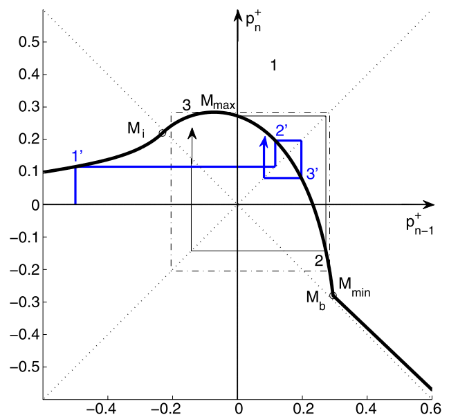
Fig. 3 Graphical illustration of the iteration, where an initial point 1 is iterated into point 2, 3, etc. (similarly for the point 1' , 2' , 3' ,...). Since the non-linear iteration function has a maximum f_{\max} , after a few steps the iteration remains inside an "iteration square" shown in broken lines. This square has its upper side tangent to the maximum of the function, at point M_{\max} , which after one iteration becomes point M_{\min} defining the lowest side of the square (ordinate f_{\min} ). Depending on the parameters, the iteration square contains or does not contain the contact point M_b and the flow inversion point M_i . Here, \gamma = 0.44 , \zeta = 0.8 , \lambda = 0.95
