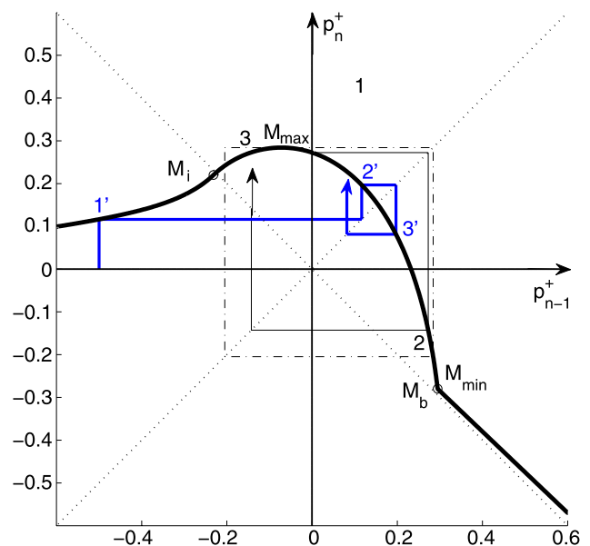
Fig. 3 Graphical illustration of the iteration, where an initial point 1 is iterated into point 2, 3, etc. (similarly for the point 1', 2', 3',...). Since the non-linear iteration function has a maximum f_{\max} , after a few steps the iteration remains inside an “iteration square” shown in broken lines. This square has its upper side tangent to the maximum of the function, at point M_{\max} , which after one iteration becomes point M_{\min} defining the lowest side of the square (ordinate f_{\min} ). Depending on the parameters, the iteration square contains or does not contain the contact point M_b and the flow inversion point M_i . Here, \gamma = 0.44 , \zeta = 0.8 , \lambda = 0.95
