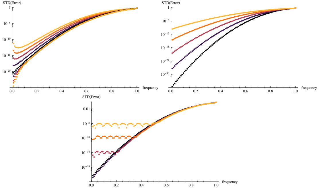
Figure 3: Frequency dependence of the standard deviation of the relative error in the optimal sector (75 central points with M = 219 ), between the interpolated and the analytic derivatives and antiderivatives of a truncated sampled \text{Cos}[2\pi \phi t] computed with Equation (5) and different values of the frequency \phi ; freq=1 correspond to the Nyquist frequency (2 samples per period). Upper left: Influence of the derivative (same colors as Figure 2). Upper right: Influence of the parameter \sigma : From dark to light: \sigma = 4\pi, 3.5\pi, 3\pi, 2.5\pi and 2\pi , with N = \infty . Bottom: Influence of the number of terms in Equation (8): From dark to light: N = \infty, N = 15, N = 12, N = 10 and N = 8 , with \sigma = 3\pi .
