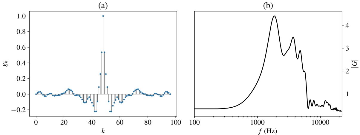
Figure B.9: Simplified impulse response g_k and transfer function G and (for F_s = 44.1 kHz).
