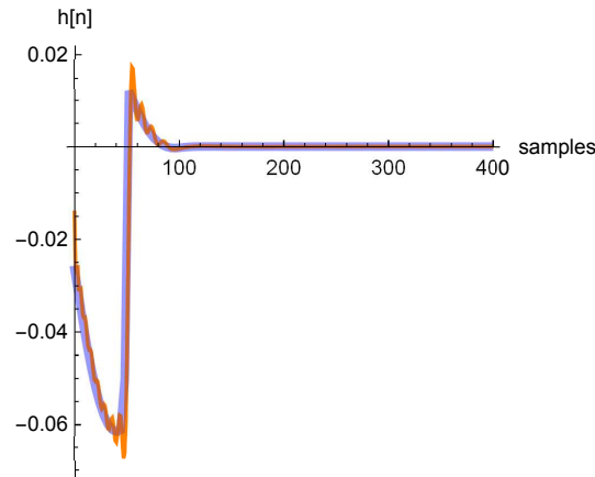
Figure 7.5 – Discrete impulse response of the reflector R_g of the flared duct depicted on Fig. 7.3. Blue: after oversampling / downsampling of the analytical function, as discussed in §7.4.2. Orange: discrete impulse response of the filter illustrated on Fig. 7.4 (b). The Gibbs phenomenon is a consequence of the frequency band limitation (see Appendix E). The amplitude of the ripples has to be controlled by the least squares fit in such a way that the simulated scattering matrix remains i) passive at every frequency and ii) accurate in the pass band.
