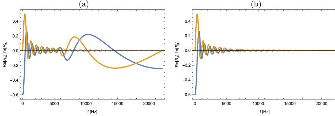
Figure 7.3 – Simulated flared duct with constant curvature ( r_g = 10 mm, r_d = 20 mm, L = 200 mm, \Upsilon = 30 ).
